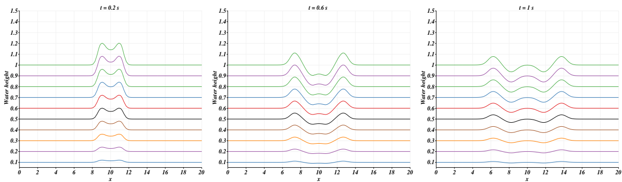
Fig 4.59. Vertical cross-sections at y = 0 of water heights from t = 0.2s to t = 1s for the multilayer circular dam-break on a flat bottom using 10 layers.
