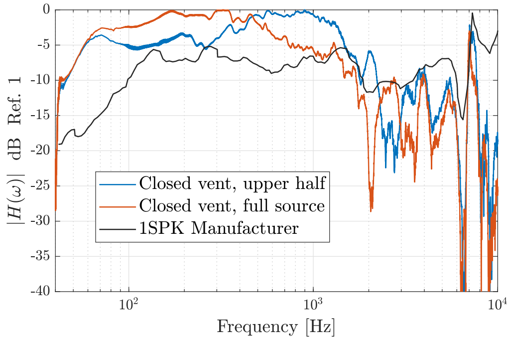
Figure 5.11: Measured spectra (normalized to \max 0 dB) of the 2 m NDP source with closed cabinet (as used during in-situ measurements) for two conditions: driving only one half of the array and the entire array (as used in measurements). Data is overlaid with SPL informed by the manufacturer normalized by its peak at 7 kHz.
