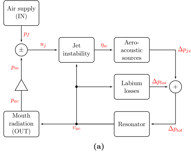
Figure 4.1: Closed loop operation in wind instruments of self-sustained oscillation type.
