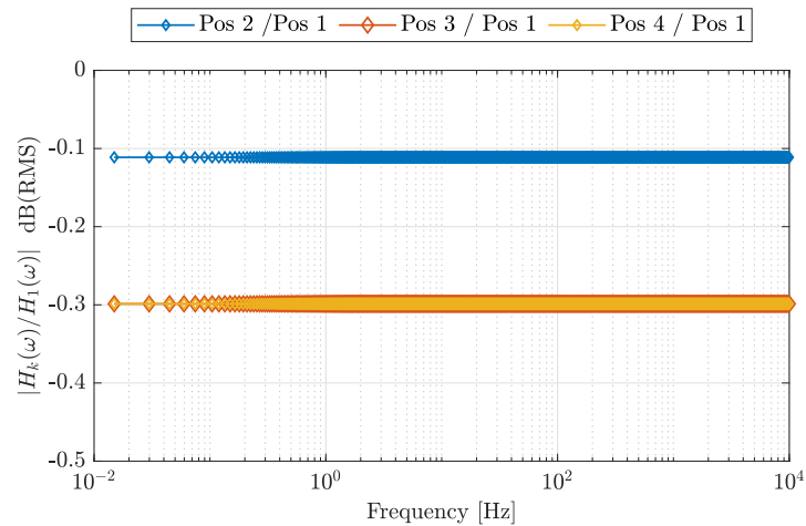
Figure 5.12: Measured pressure differences of the 2 m source across the spectrum for the vertically aligned acquisition locations using the lowest measurement point as a reference. Data is filtered per thirds of octave bands and scaled by the db(RMS) of each sub-band driving the full array source.
