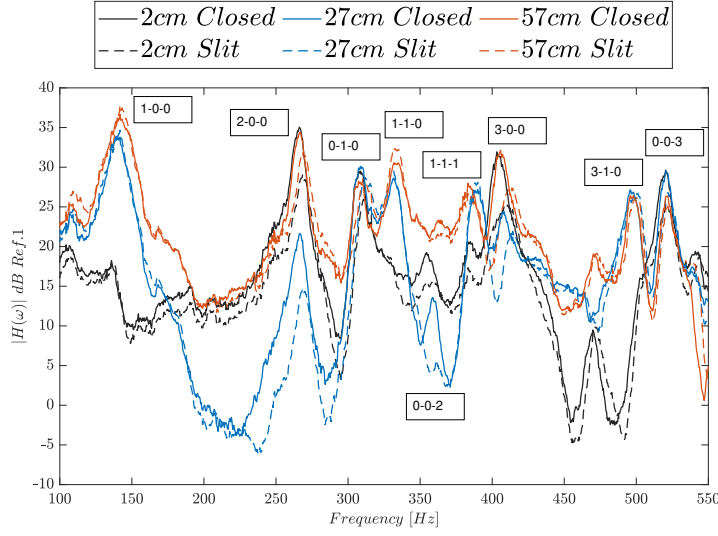
Figure 6.12: Measured internal pressure field for a cavity with no apertures and one aperture at different internal positions. Distances are referred over the X -axis and away from the center of the front wall. The values for the modal frequencies annotated (closed cavity) may be found in Table 6.2.
