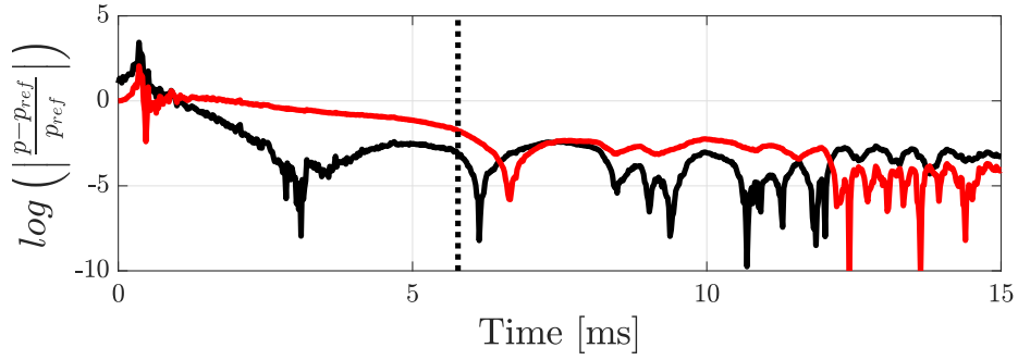
(a) Simulation errors for p_{\text{grv}}
