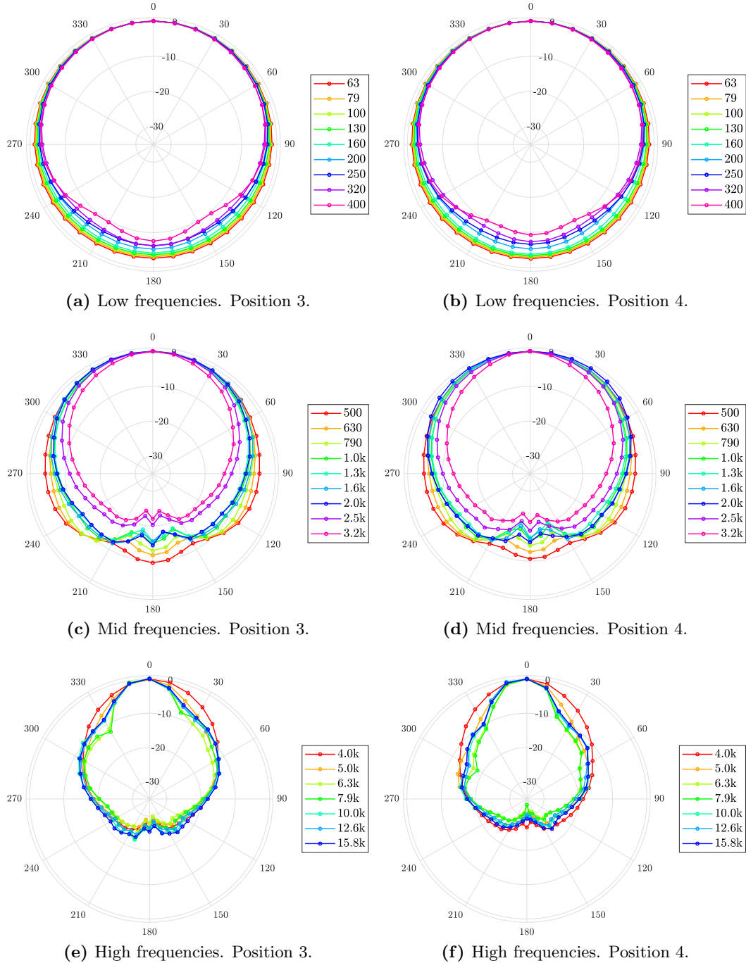
Figure 5.10: Directivity of the 2m source measured at 1 m. Left: on axis with the space in between the two speakers at half the height of the source. Right: on axis with the membrane cone of the speaker immediately above half the height of the source.
