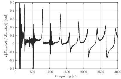
(c) Fitted phase error
