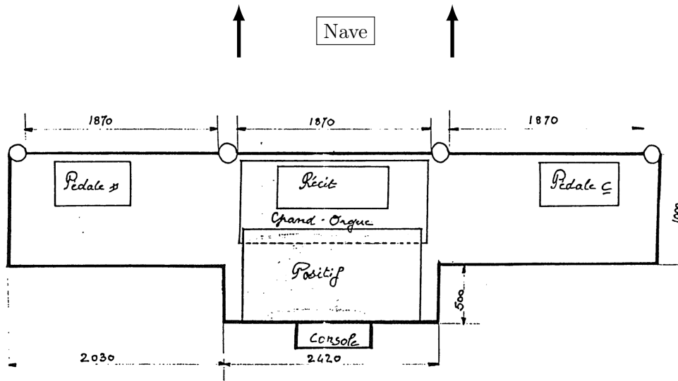
Figure 1.3: Layout of the buffet of the Orgue Dallery. Units in mm. Height of the buffet: 3300 mm. Source: [Dubois and Lueders, 2002].
