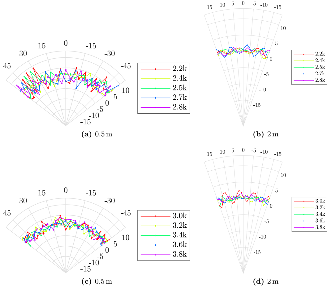
Figure B.11: Lateral organ rigid walls only. Measured pressure, relative SPL dB rms normalized by free propagation reference.
