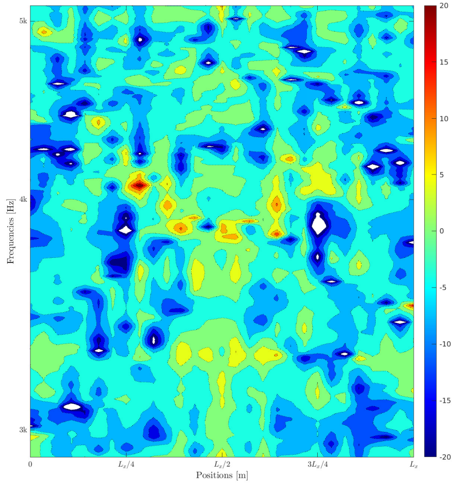
Figure B.7: Mid frequencies of the measured facade pressure transfer function. Walls removed, only 16 cylinders at the front array. Measurement distance: 0.2m from the front array. The effect of the reference field with no pipes and walls has been subtracted.
