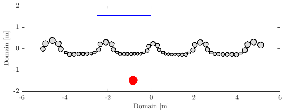
Figure 6.23: Geometry of the NDP tribune organ façade. Annotations: source position (●), acquisition line every 1 cm (—)
