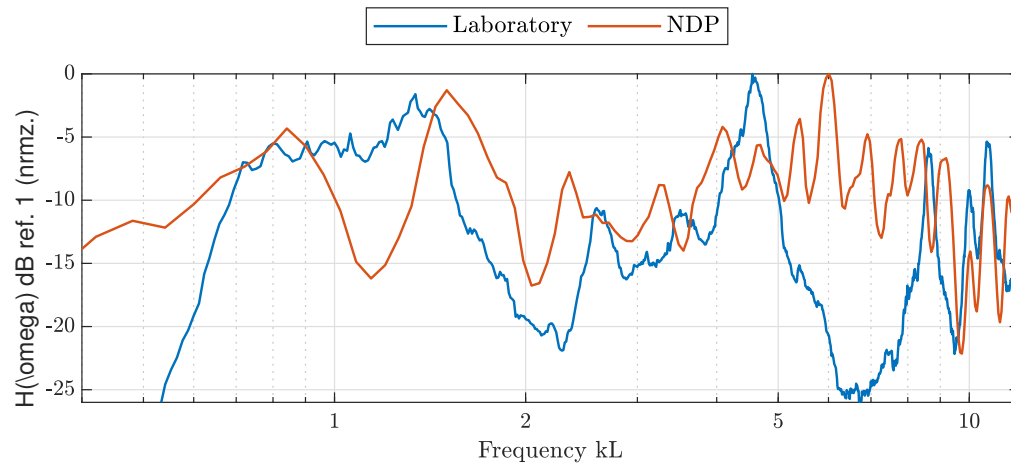
Figure 6.22: NDP buffet internal response as excited by a big balloon explosion compared with the internal response of the laboratory cavity. No pipes in the interior, and semi-open conditions (façade). The characteristic length is taken as L = \sqrt{L_x^2 + L_y^2 + L_z^2} , where for the NDP organ only the height of the first floor of windchests is considered ( L_{y,NDP} = \sim 2 m).
