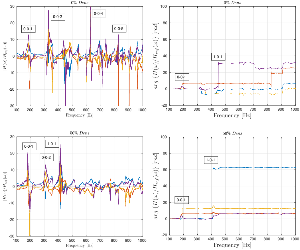
Figure 6.13: Magnitudes (left) and phases (right) of pressure at the slit for different vertical alignments. Tracing the decrease in frequency of the X – Z -mode with increasing density of scatterers, it indicates that the average effect of one cylinder diminishes the resonance by -0.378 Hz. Bottom microphone to mid-low microphone: Mic1/Mic2 —; mid-height to mid-low microphone: Mic3/Mic2 —; mid-top to mid-low: Mic4/Mic2 —; top microphone to mid-low: Mic5/Mic2 —. A complete set of measured data at different densities may be found in Figure B.4 and Figure B.5 (Appendix B).
