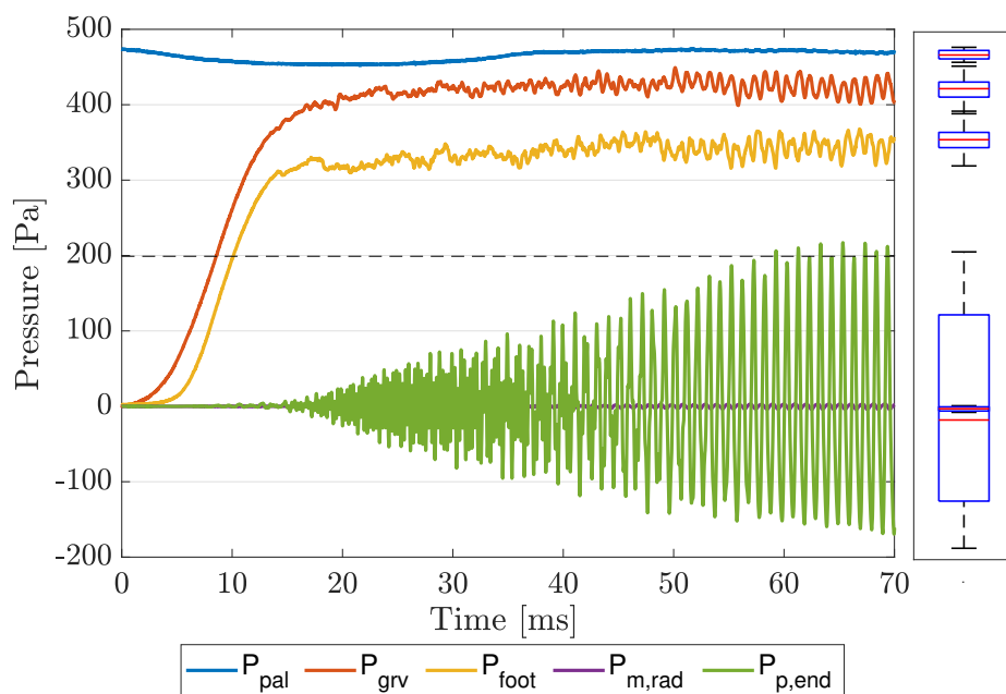
Figure 3.3: Left: overview of measured pressure time-series showing the transient build-up of Pipe 5, with geometry details in Table 3.1. The horizontal dashed line indicates the target pressure amplitude inside the resonator reached in SS. Right: data deviation, over 20 periods in SS.
