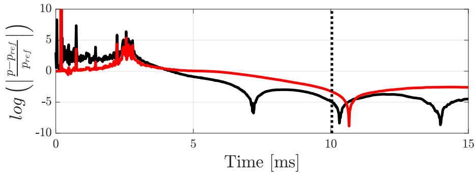
(b) Simulation errors for p_{\text{foot}}
