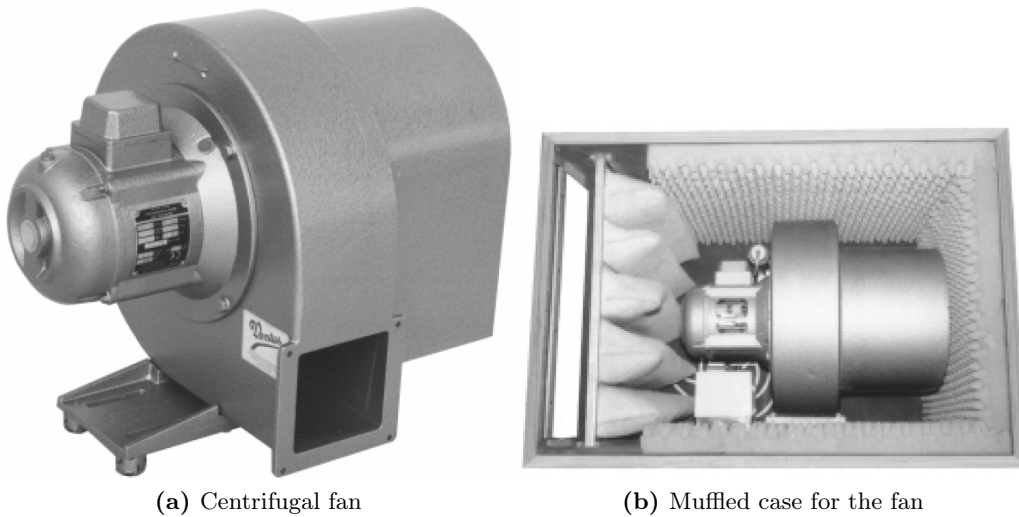
Figure 2.4: Electric wind supply system example. Images by Laukhuff Orgelbau.
