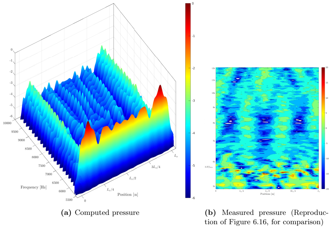
Figure B.2: Computed scattered pressure (normalized dB) in the range 5.5 kHz to 10 kHz as per [Mellow and Kärkkäinen, 2011] model, spanning the width the laboratory setup, with a grid spacing of 2 mm and a frequency bin of 2 Hz.
