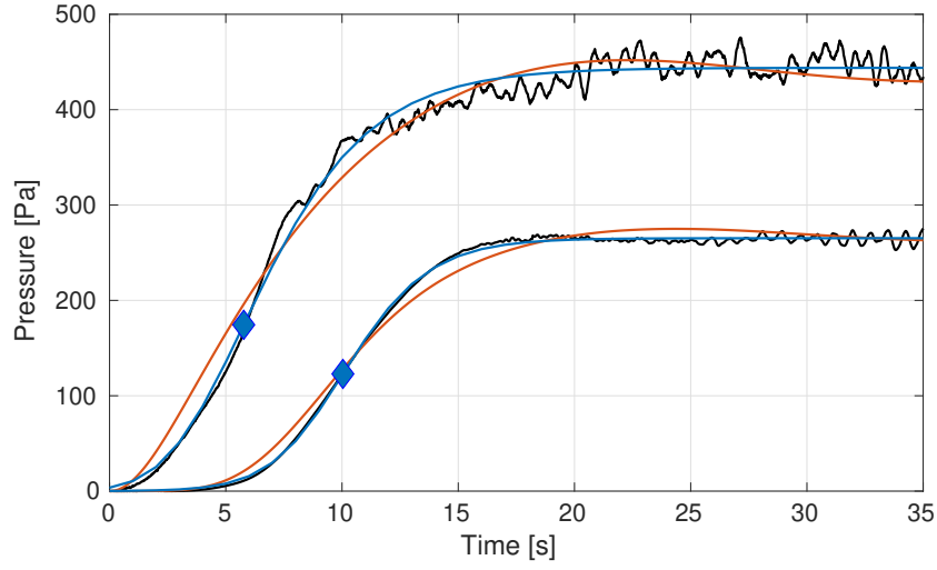
Figure 3.12: Measured pressure transient overlaid with time-stepping numerical solution of Equation (3.3) and the fitted model for p_{\text{grv}} and p_f . Markers indicate the maximum growth rate. Measured pressure (—), physical model (—), fitted model (—).
