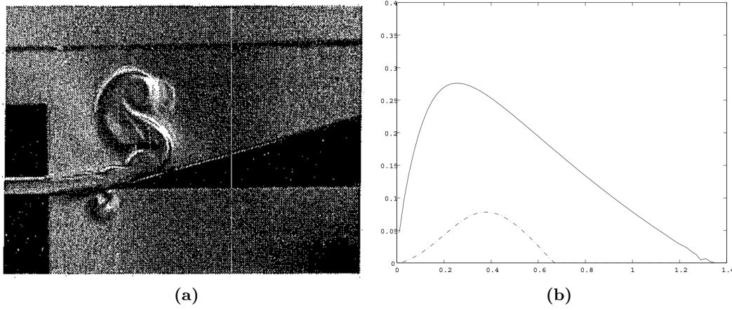
Figure 2.6: (a) Schlieren visualization of the outward jet deflection at the mouth-labium region and vortex pairs. Image credit: B. Fabre and A. Ernoul, 2016. (b) Numerical resolution of Rayleigh's equation in [Verge et al., 1994a, Ségoufin, 2000] showing the dominance of the sinuous modes (antisymmetric) of the perturbation over the varicous ones (symmetric). Data shows the dimensionless spatial amplification \alpha_i \cdot b against dimensionless frequency by the Strouhal number, Str = \omega b / U_o . Antisymmetric solution (—) and symmetric solution (---).
