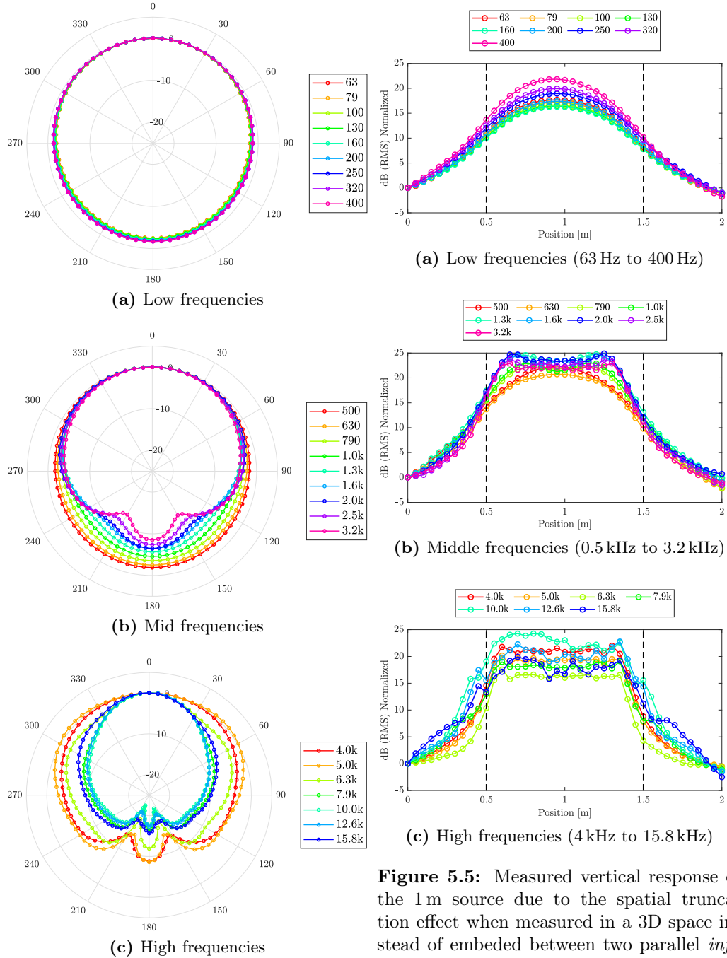
Figure 5.4: Directivity of the 1m source due to the spatial truncation effect when measured in a 3D space instead of embedded between two parallel infinite planes. Data analyzed in thirds of octave bands. The dashed black line indicates the range of acquisition locations in front of the source. Normalized data at 0° per band.
