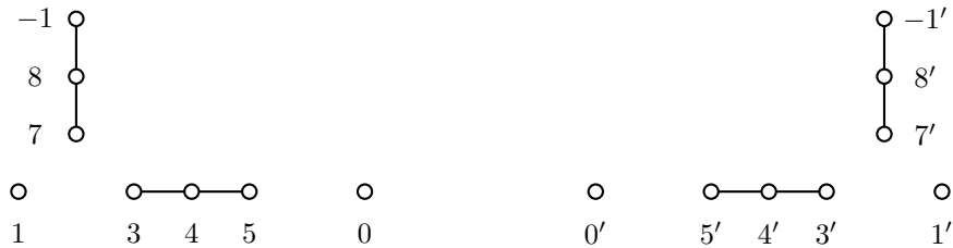
Figure 2.12: Dynkin diagram corresponding to the 16 simple roots that survive the breaking by the Wilson lines (2.4.32).
