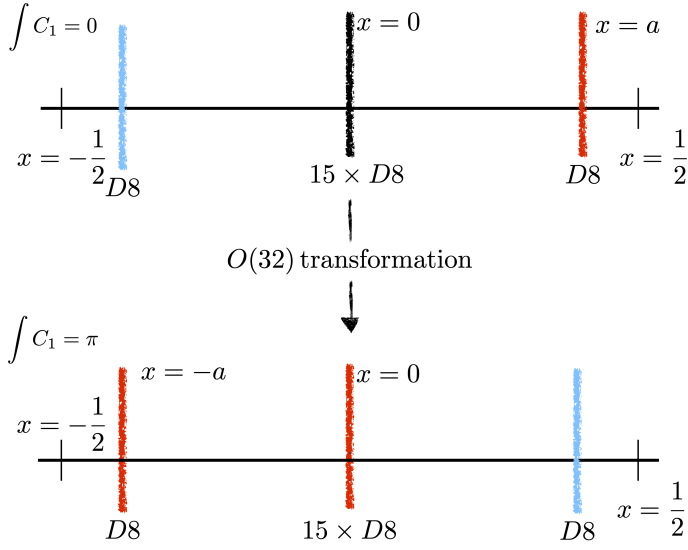
Figure 6.1: The type I' theory describes D8 branes on an interval, depicted here as the real line \mathbb{R} subject to periodic identifications. O8^- planes are found at x \in \mathbb{Z}/2 . The top section of the figure describes 15 D8 branes sitting at the origin and a single D8 brane moved to x = a . There is no Wilson line. Thanks to the anomaly described in the main text, acting with an O(32) transformation flips the position of the D8 brane to x = -a and introduces a discrete Wilson line. Since the brane at x = -a can also be obtained simply by moving the D8 to the left, we discover that the discrete Wilson line is not an invariant notion.
