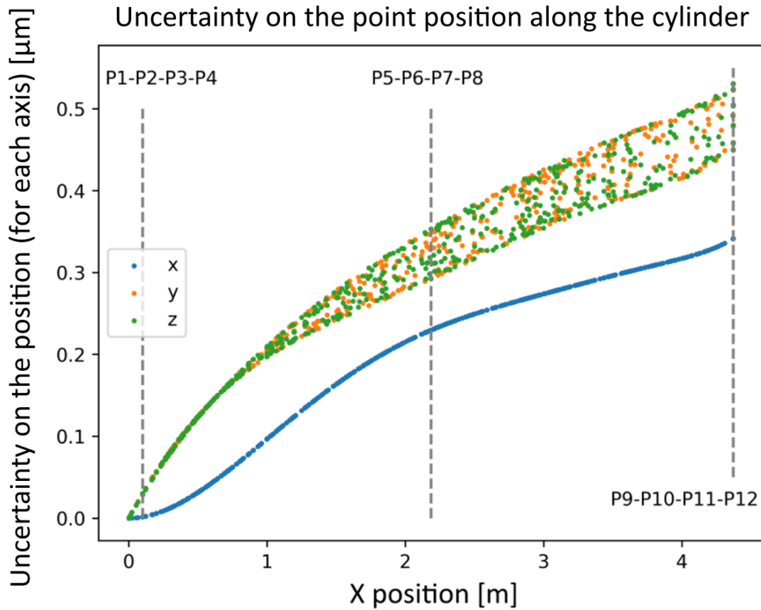
Figure 3.27: Simulations with additional implementations. Uncertainty on the point position for 500 points randomly scattered on the cylinder (sorted by their longitudinal position). The X position of the points P1 to P12 have been highlighted.
