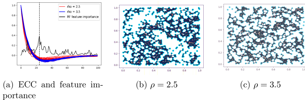
Figure 9.4: ORBIT5K classification problem: \rho = 2.5 VS \rho = 3.5 .
