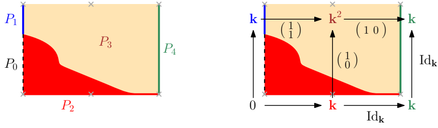
Figure 3.1: A graphical representation of the partition of the convex hull \text{conv}(G) (left), superimposed with its associated module M (right). The regions P_0, P_1, P_2, P_3, P_4 of \text{conv}(G) are represented respectively by the black dashed line segment, the blue segment, the red region (including the bottom red segment), the orange region and the green segment. The nodes of the grid G are represented as gray crosses.
