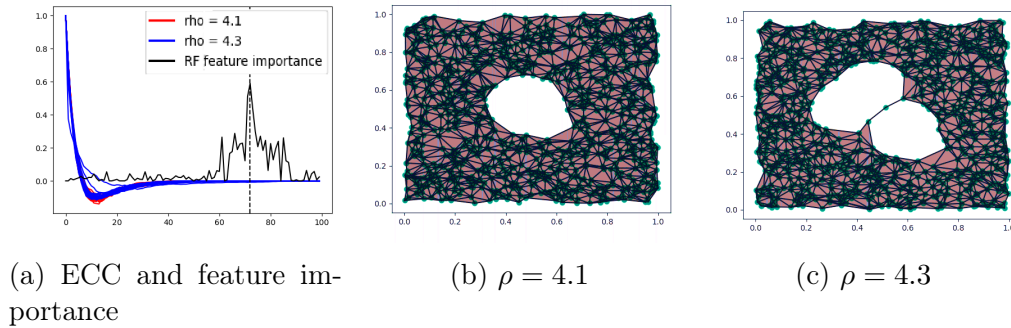
Figure 9.3: ORBIT5K classification problem: \rho = 4.1 VS \rho = 4.3 .
