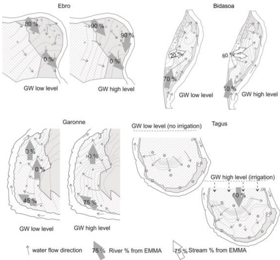
Figure 6: Flow nets of the study sites. Groundwater (GW) high and low level periods are considered separately. River water percentage in the aquifer is also shown.
