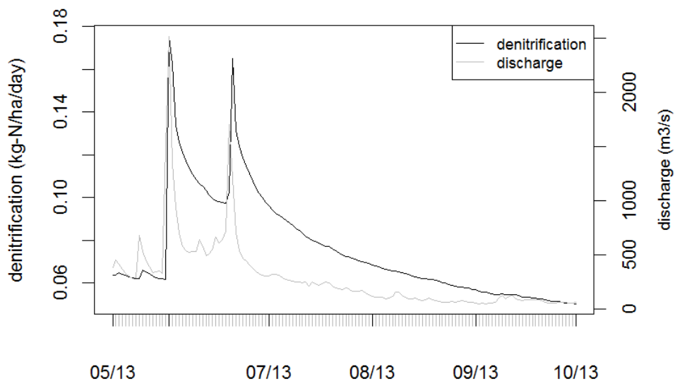
Figure 5-7: Temporal evolution of simulated integrated denitrification (average of the study area) and observed discharge.
