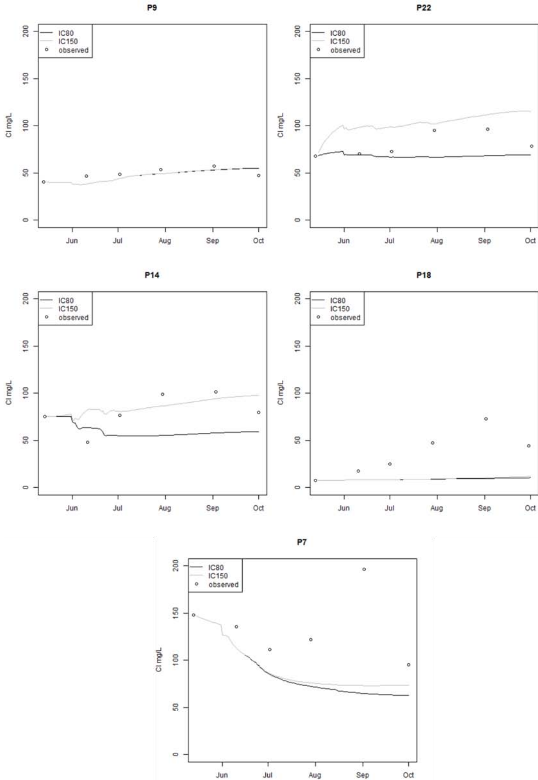
Figure 4-10 (a to e): Simulated and observed Cl concentrations for the five piezometers with continuous hydraulic head records. Black and grey lines correspond to the initial concentrations of 80 \text{ mg L}^{-1} (scenario IC80) and 150 \text{ mg L}^{-1} (scenario IC150) respectively in the agricultural area
