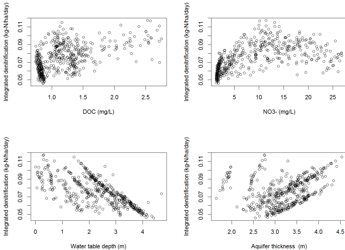
Figure 5-11 : Spatial relationship between integrated denitrification activity and DOC and nitrate (NO 3 ) groundwater concentrations, water table depth and aquifer thickness. The points represent the average of the values for each cell.
