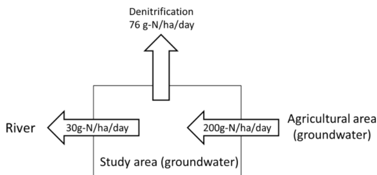
Figure 5-14: Nitrates mass balance of the study area groundwater for the simulated period. Groundwater fluxes from the agricultural area to the study area and from the study area to the river are shown as well as the N-removal through denitrification.
