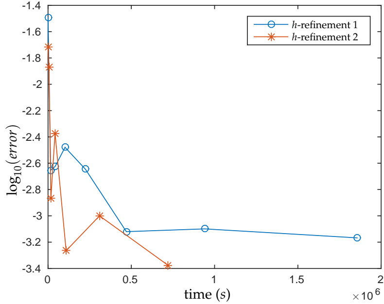
Figure 4.9: Cumulative time to compute the primal eigenvalues under h -refinement for Algorithm 4.3.1 and Algorithm 4.3.2. Data from the Maire and Talay benchmark problem with p = 1, q = 0 in the primal problem. Computed on 8 OpenMP threads.
