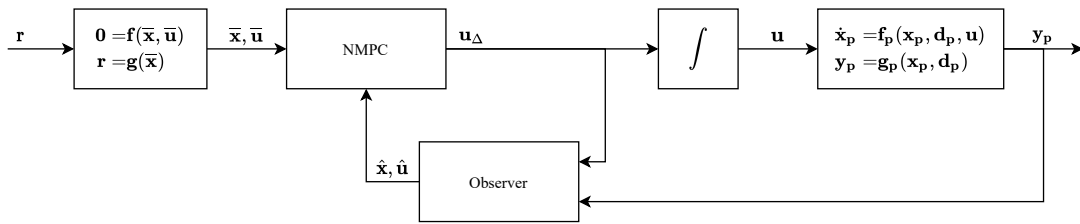
Figure 2.29 – NMPC block diagram for offset-free control.
