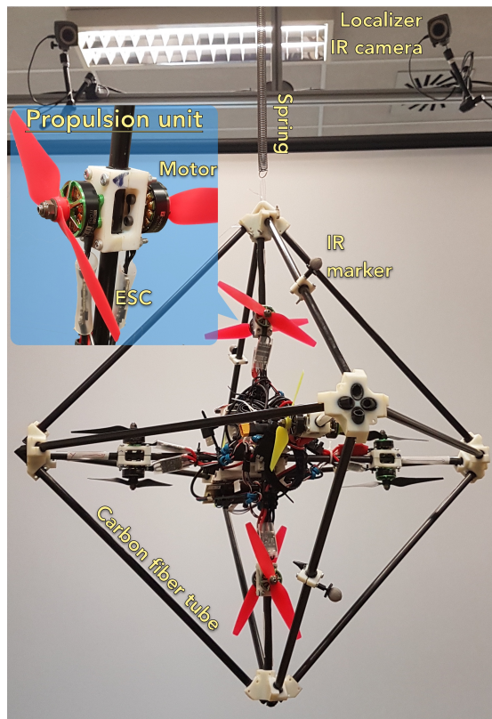
Figure 2.5 – Aerial Wrench Generator.
