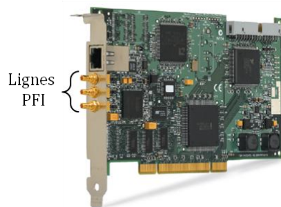
Figure II.25 Carte NI PCI-1588.
