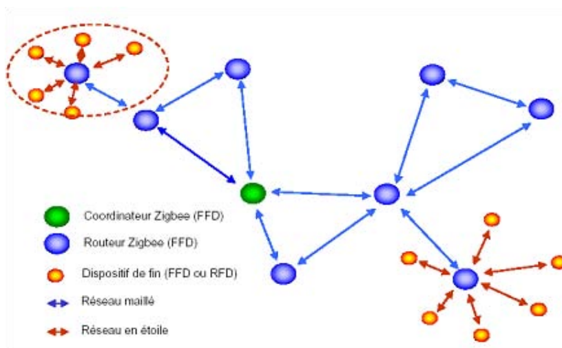
Figure I.10 Topologies LR-WPAN 9 .
