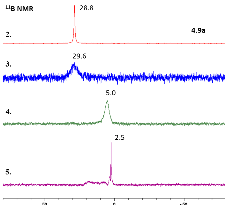
2. Pure boronic acid 4.9a in \text{CDCl}_3 ; 3. Boronic acid 4.9a , 5 Å powdered activated MS (20 mg), \text{CDCl}_3 , 25 °C, 10 sec 4. Boronic acid 4.9a (5.4 mg, 0.025 mmol), (S)-ibuprofen (6.3 mg, 0.03 mmol, 1.2 eq), 5 Å activated powdered MS (50 mg) in \text{CDCl}_3 , 25 °C, 30 mins 5. Mixture of entry 4 + pyridine (2 \mu\text{L} , 2 mg, 0.025 mmol, 1 eq), 25 °C, 3 mins.
