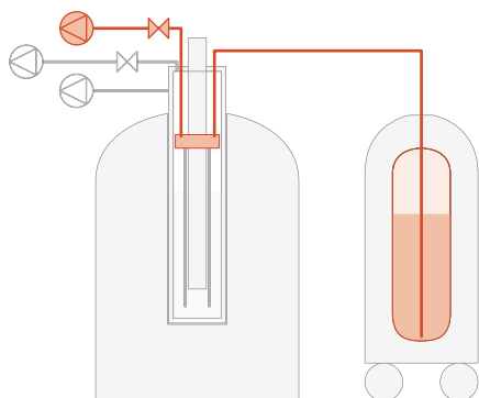
Figure 3.1: A. Diagram of the polarizer detailing the components of the cryostat. B-C. Helium flow path to bring helium inside the cryostat through the phase separator and to pump on the sample space, respectively.
