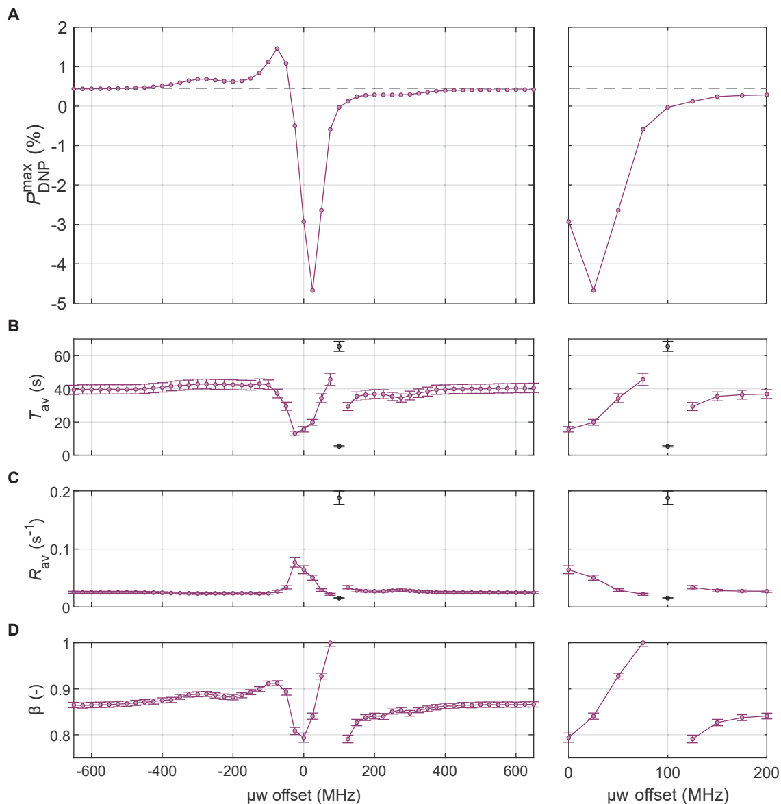
Figure 3.28: A. \mu w spectrum of PANI with \chi = 0.2 on a broad range of \mu w frequencies. B-C. Average build-up time and rate constant T_{av} and R_{av} , respectively, obtained from the stretched exponential fit of the build-ups using Eq. 3.34. D. Stretched coefficient obtained by fitting the build-ups with a stretched exponential model. The build-up with \mu w frequency +100 MHz could not be fitted with a stretched exponential (see Fig. 3.29) and was fitted with a biexponential function instead (see Eq. 3.47 and Fig. 3.29). The fitted values of the biexponential model are shown as black dots on Panel B and C.
