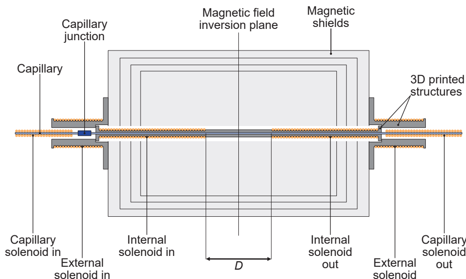
Figure 6.13: Schematic representation of the inversion chamber. Dark gray elements represent 3D-printed structures. Filled yellow circles represent wires of solenoid coils. A photograph of the internal coil is shown in Fig. 6.8.
