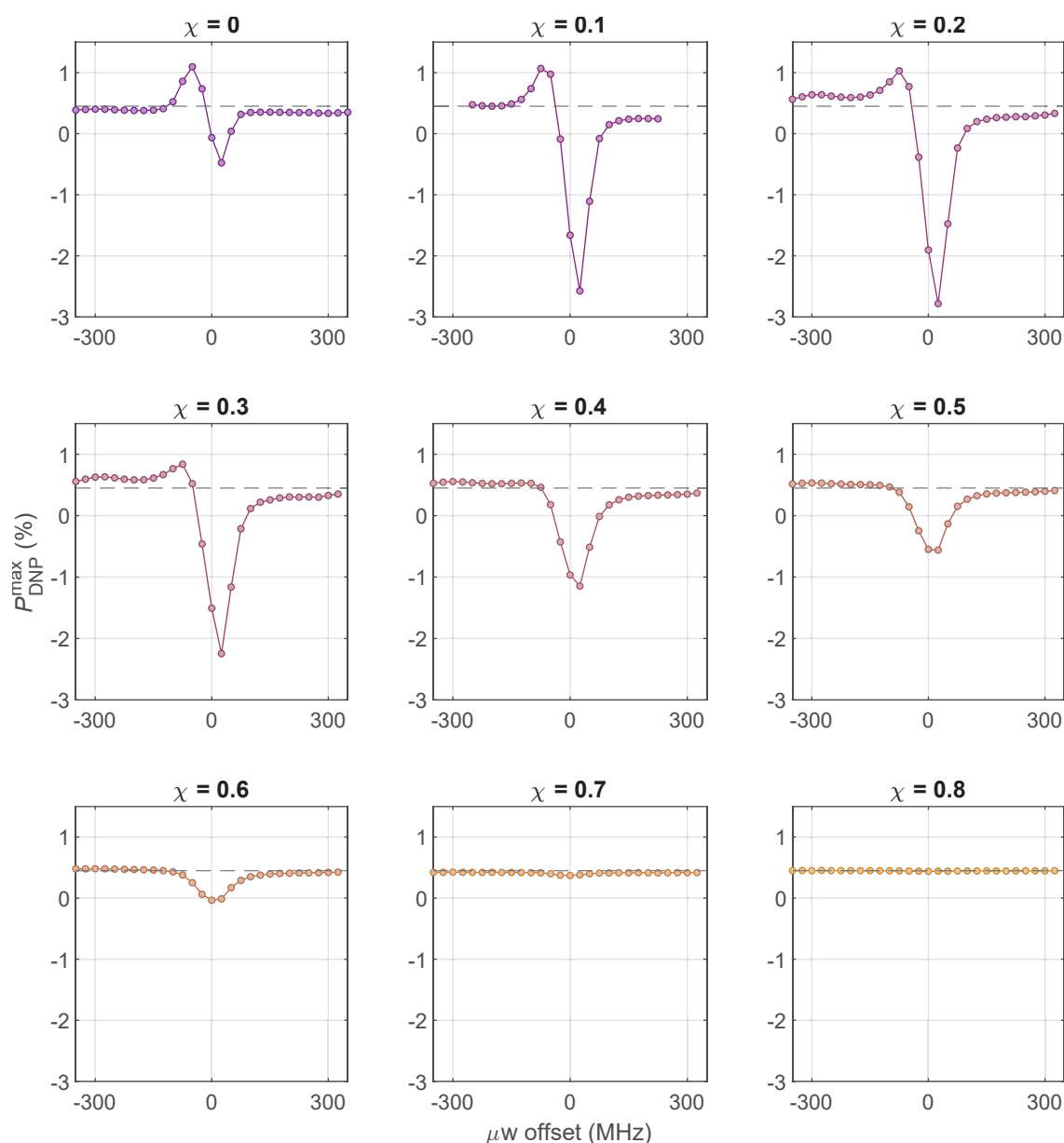
Figure 3.27: \mu\text{w} spectra for PANI with various values of expected conversion \chi from EB to ES, for \approx 30 mg of sample at 1.6 K. The horizontal dashed line corresponds to the Boltzmann equilibrium polarization of ^1\text{H} spins P_{eq} \approx 0.45\% .
