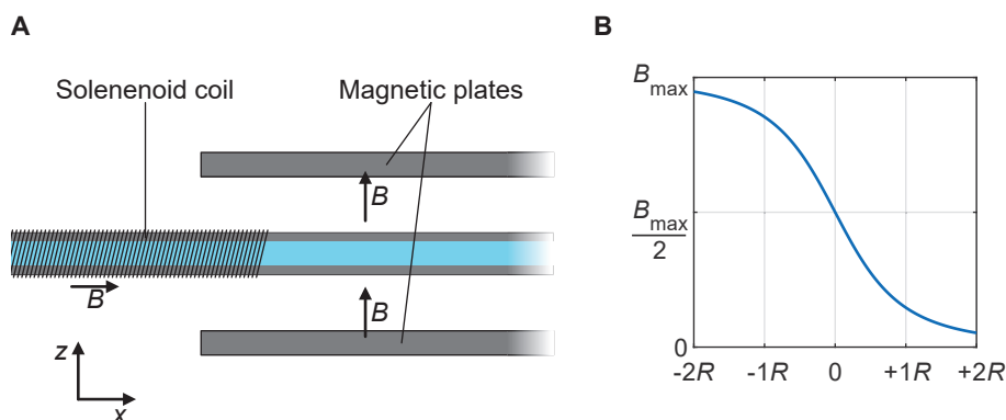
Figure 6.7: A. Schematic representation of a capillary surrounded by a solenoid coil on one side and by two magnetic plates on the other. B. Magnetic field at the center of a solenoid (with L \gg R , where L and R are the radius and the length of the solenoid, respectively), with respect to its maximum field strength B_{\max} , as a function of position, calculated using Eq. 6.19 (more details in Sec. 6.2.3). The origin is located at the edge of the solenoid.
