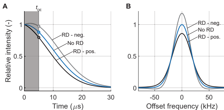
Figure 3.7: A-B. Schematic representation of the effect of RD on the FID and the NMR spectrum, respectively. The dots on the curves of Panel A represent the signal intensity at the end of the dead time t_{DE} , that is, the first recorded point of the FID.
