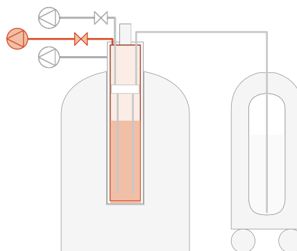
Figure 3.1: A. Diagram of the polarizer detailing the components of the cryostat. B-C. Helium flow path to bring helium inside the cryostat through the phase separator and to pump on the sample space, respectively.
