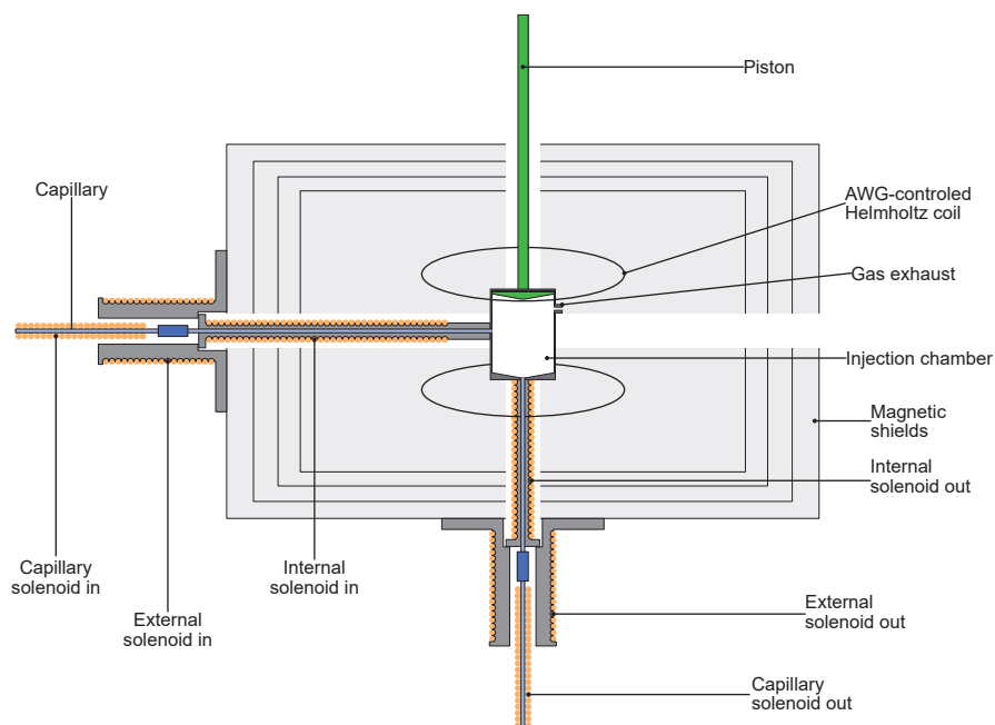
Figure 6.19: Schematic representation of an experimental setup for ^1\text{H} \rightarrow ^{13}\text{C} polarization transfer by adiabatic field inversion on a static sample, where the field profile over time is generated by an AWG controlled-Helmholtz coil.
