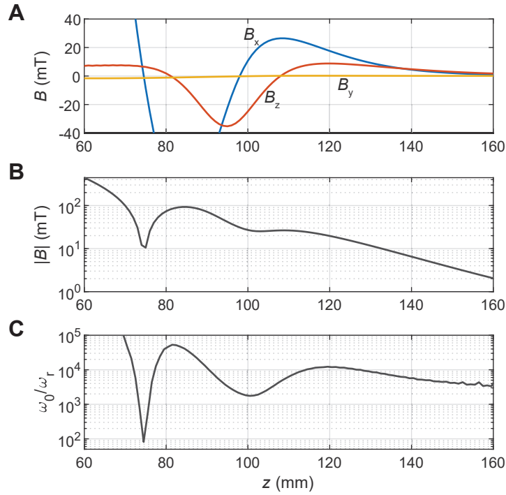
Figure 6.4: A-B . Projections along Cartesian axes and norm of the stray field of the Bruker Fourier 80 benchtop spectrometer as a function of the distance to the center, respectively. C . Ratio of the Larmor frequency of ^{13}\text{C} spins moving at 5 \text{ m.s}^{-1} along the z -axis and the rotation rate of the magnetic field.
