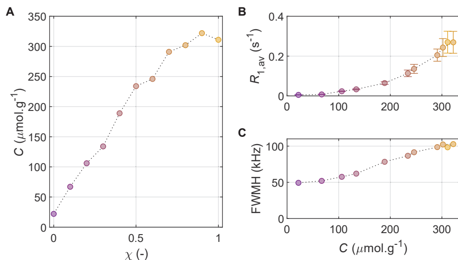
Figure 3.25: A. Electron spin concentration of PANI samples as a function of the protonation ratio \chi , determined by X-band EPR at room temperature. B-C. Average relaxation rate obtained by fitting a stretched exponential (see Eq. 3.33) to the ^1\text{H} thermal equilibrium build-ups and FWHM of the ^1\text{H} signal of the same samples at thermal equilibrium at 1.6 K, respectively, as a function of the electron spin concentration shown in Panel A.
