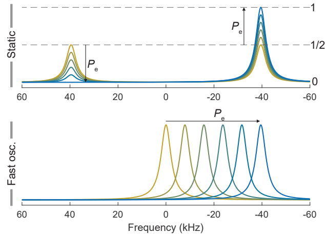
Figure 2.13: Numerical simulation of ^1\text{H} NMR spectra for a ^1\text{H} spin interacting with an electron spin with a hyperfine interaction of 79 kHz for the case of an electron with static spin state and with a rapidly fluctuating state. The simulated FID is the expectation value of \hat{I}_{1+} with 512 time increments of 4 \mu\text{s} . A 5 kHz line broadening and zero filling to 2048 points were applied prior to Fourier transform.
