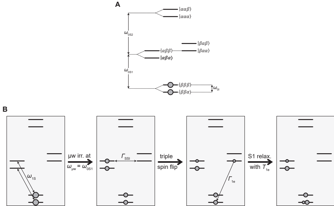
Figure 3.16: A. Eight energy levels of a 2 electron-1 nucleus spin system used to describe the CE, where the electrons are assumed to be fully polarized while the nucleus has polarization P_1 \approx 0 . Because of the matching condition of Eq. 3.20, the |\alpha\beta\beta\rangle and |\beta\alpha\alpha\rangle states are degenerate. B. Schematic representation of the steps of CE-DNP. \Gamma_{SS1} is the triple spin-flip rate connecting the |\alpha\beta\beta\rangle and |\beta\alpha\alpha\rangle states.
