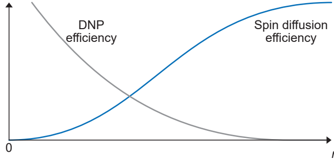
Figure 5.1: Schematic representation of the efficiency of DNP and spin diffusion as a function of the distance to the electron r .
