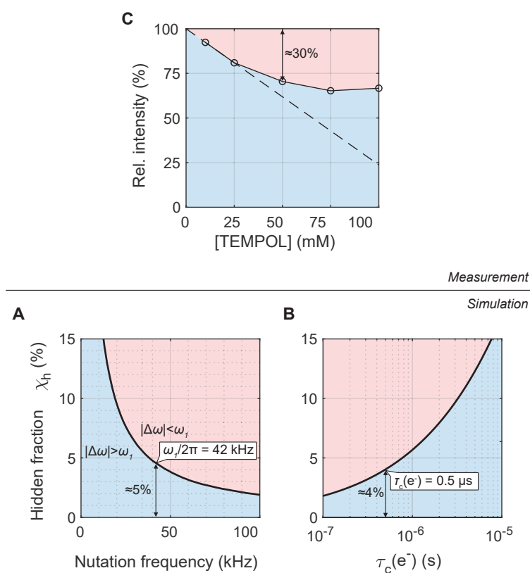
Figure 5.9: A. Relative ^1\text{H} signal as a function of TEMPOL radical concentration in DNP juice at 3.8 K (open circles) showing that the presence of the radical quenches \approx 30\% of the NMR signal for a concentration of 50 mM. The dashed line represents a linear interpolation of the first two points. B. Simulated fraction of the spins that are hidden because they are unaffected by rf pulses as a function of the pulse bandwidth. \Delta\omega and \omega_1 are the paramagnetic shift and nutation frequency of the pulses, respectively, used to discriminate between visible and hidden spins. C. Simulated fraction of the spins that are hidden because of the reduction in transverse relaxation time constant due to PRE. The light blue and pink areas represent the visible and hidden fraction of the ^1\text{H} spins, respectively.
