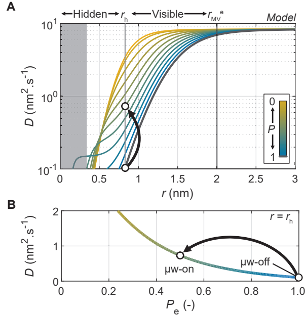
Figure 5.26: A. Calculated spin diffusion coefficient as a function of the distance to the electron for the same spin system for different electron polarization \bar{P} between 0 and 1 in steps of 0.1 (see Eq. 5.49). The vertical black and gray lines represent the radius of the mean volume per electron and the limit between the visible and hidden spins, respectively. The gray area indicates the region where the model hypothesis breaks down ( 1/\tau_c < |A_{zzi}| ). B. Spin diffusion coefficient as a function of the electron polarization at the interface between hidden and visible spins. The arrow between the two hollow circles on both panels indicates the increase in diffusion coefficient upon switching on \mu\text{w} irradiation. The nuclear interdistance r_a , the nuclear broadening due to nucleus-nucleus interactions, and the electron correlation time \tau_c are assumed to be 0.66 nm, 18 kHz, and 0.5 \mu\text{s} , respectively.
