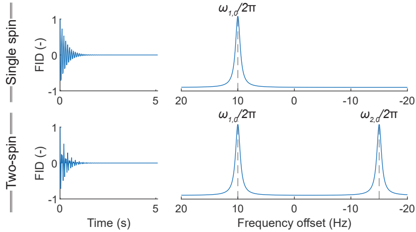
Figure 2.5: Numerical simulation of the spectra for pulse-acquire experiments for a single-spin system and a homonuclear two-spin system (top and bottom, respectively). The plots on the right are the Fourier transform of the plots on the left. Simulation with 256 time increments of 10 ms, Fourier transform after applying \delta \nu_{1/2} = 1 Hz of line broadening and zero-filling to 1024 points. For both the FIDs and the spectra, the real part of the signal is displayed.
