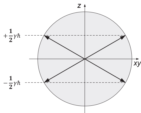
Figure 2.1: Representation of the magnetic moment of a spin 1/2 and its projection along a reference axis.
