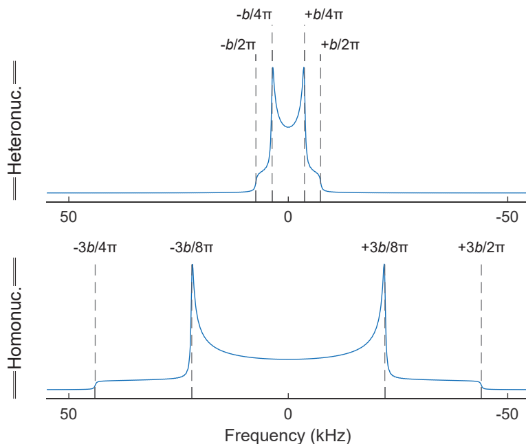
Figure 2.11: Numerical simulation of ^1\text{H} NMR spectra at high-field for heteronuclear and homonuclear dipolar coupled spins, for ^1\text{H} - ^{13}\text{C} and ^1\text{H} - ^1\text{H} pairs, respectively, separated by 1.6 \text{ \AA} . The initial polarization of the spins was assumed to be 0.001. A \pi/2 pulse was simulated on the ^1\text{H} spins, prior to propagation of the free evolution during 512 time steps of 4 \mu\text{s} . The simulated FID is the expectation value of \hat{I}_{1+} and \hat{I}_{1+} + \hat{I}_{2+} for the hetero and homonuclear cases, respectively. It was averaged over 1000 increments of the angle between the internuclear vector and the magnetic field from 0 to \pi . A 500 Hz line broadening and zero filling to 2048 points were applied prior to Fourier transform.
