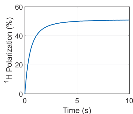
Figure 6.14: ^1\text{H} DNP build-up at 1.6 K and 7.05 T for 100 \mu\text{l} of 0.4 M ^{13}\text{C} -formate, [3\text{-}^{13}\text{C}] -pyruvate, [2\text{-}^{13}\text{C}] -pyruvate and [1\text{-}^{13}\text{C}] -pyruvate in DNP juice doped with 50 mM TEMPOL.
