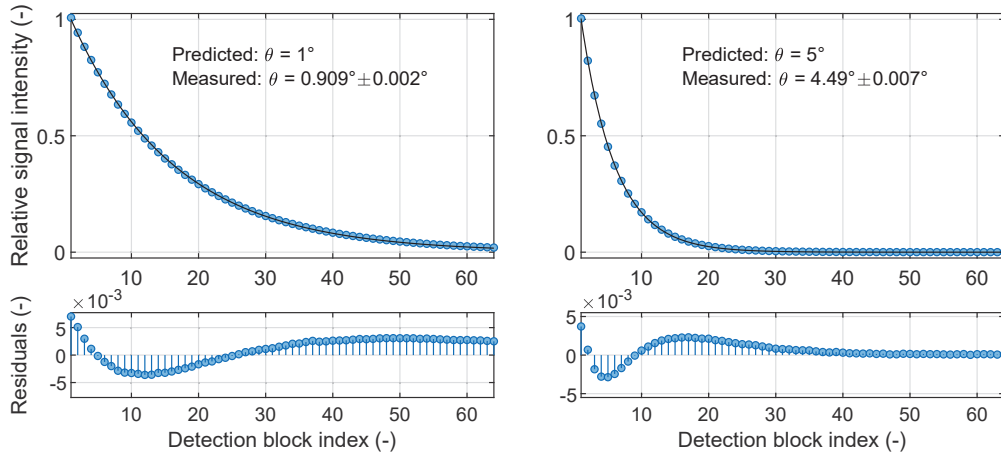
Figure 3.9: Fit of the signal decay under the magnetization depletion by small angle pulses for predicted angles of 1^\circ and 5^\circ on a sample of 3 M [1-^{13}\text{C}] -acetate and 50 mM TEMPOL in DNP juice at 1.2 K, using Eq. 3.15. Prior to detecting the decay, the ^{13}\text{C} spins were hyperpolarized by multi-contact CP to reach high SNR. Each point is the sum of N_S = 256 and 64 transients in the case of 1^\circ and 5^\circ pulses, respectively.
