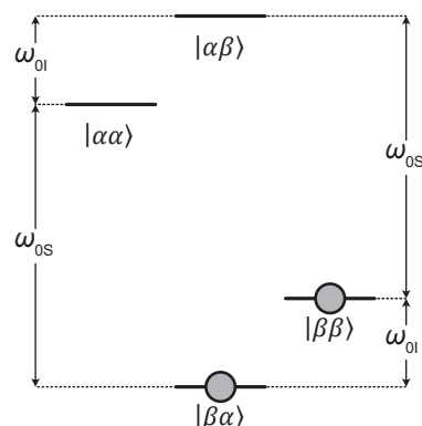
Figure 3.12: Schematic representation of the four levels of a 1 electron-1 nucleus spin system. The gray dots represent the populations at thermal equilibrium (i.e., without DNP), in conditions where the electron spin is fully polarized and the nucleus has polarization P_I \approx 0 .
