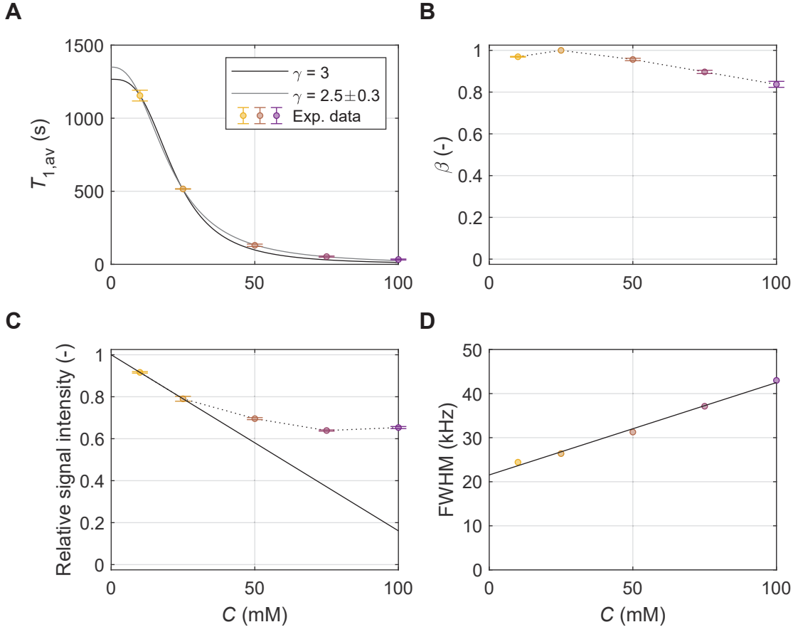
Figure 3.20: A. Average spin-lattice relaxation time constant of DNP juice as a function of radical concentration at 3.8 K shown as colored dots, obtained by fitting Eq. 3.33 to the data of Fig. 3.19 (converted from T_1 to T_{1,av} using Eq. 3.34). The black and gray lines correspond to the model of Eq. 3.42 and Eq. 3.42 with \gamma = 3 and with \gamma left as a free parameter, respectively. B-C. \beta coefficient and intensity at t \rightarrow \infty , respectively, obtained from the same fit as on Panel A. The black line on Panel C is a linear regression of the first two points of the curve. D. FWHM of the thermal equilibrium signal as a function of radical concentration, obtained using Topspin's built-in function hwcal . The colored dots and the black line are the experimental data points and the linear regression, respectively.
