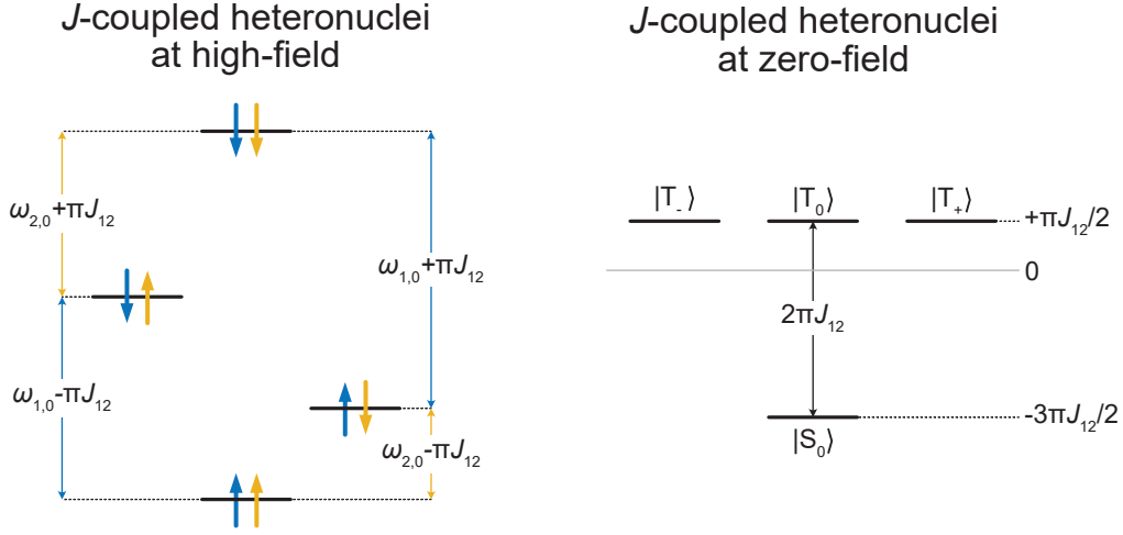
Figure 2.8: Comparison of the energy diagrams for J -coupled heteronuclear spins at high- vs zero-field for a positive J -coupling constant.
