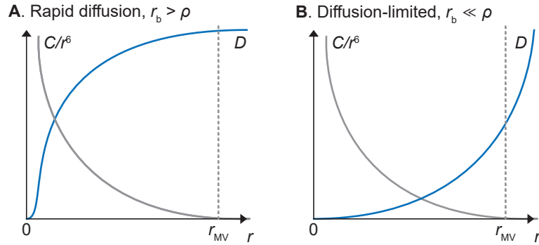
Figure 5.2: Schematic representation of rapid spin diffusion (A) vs diffusion-limited (B)
