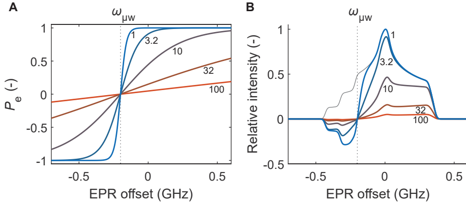
Figure 3.18: A-B. Electron polarization along the EPR line for \alpha = 0 and various values of \beta shown next to curves as spin temperature T_\beta in mK and corresponding EPR spectra, respectively. The unperturbed simulated EPR spectrum is shown for comparison in light gray on Panel B.
