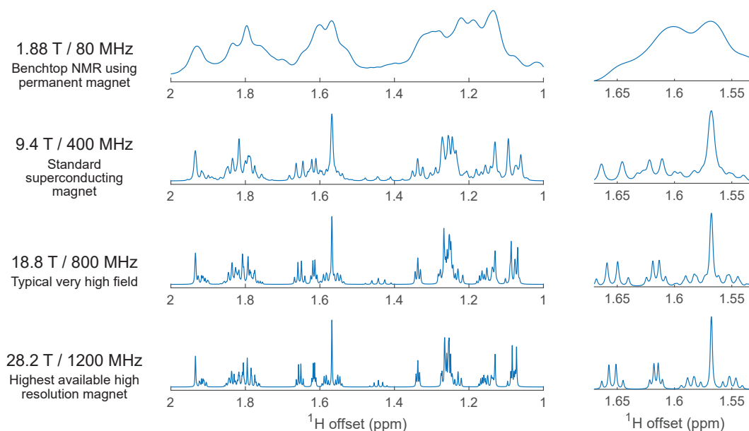
Figure 1.3: Effect of the magnetic field strength on the resolution of high-field NMR illustrated by the simulation of ^1\text{H} spectra at various magnetic fields for the same mix of 12 molecules, with equal concentration with random couplings between -15 and +15 Hz and with random chemical shifts between 1 and 2 ppm (with spin topology A_3B_2C , A_3B_3 , A_2B_2 , A_4B , A_3B_2C , A_2B_2\dots ) with a line broadening of 2 Hz. Each spectrum is normalized to the maximum intensity. The spectra on the right are a zoom of those on the left.
