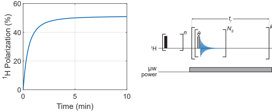
Figure 3.5: Example of an experimental DNP build-up curve of 100 \mu\text{L} of DNP juice doped with 50 mM TEMPOL, recorded at 1.6 K in our polarizer using small angle pulses with \theta = 0.1^\circ for detection where each point is the sum of N_S = 64 transients with a repetition time t_r = 5 s, after a saturation with typically n = 30 \pi/2 pulses.
