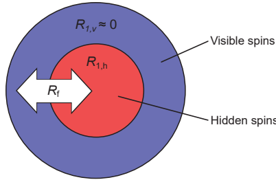
Figure 5.6: Schematic representation of the model used to analyze HypRes results. The relaxation rate constant of the visible spins R_{1,v} is assumed to be negligible. Polarization flows between the visible and hidden reservoirs at flow rate R_f , while the hidden spins relax to thermal equilibrium at rate R_{1,h} . Adapted from Ref. [68] according to the terms of the Creative Commons Attribution-NonCommercial 4.0 International Public License.
