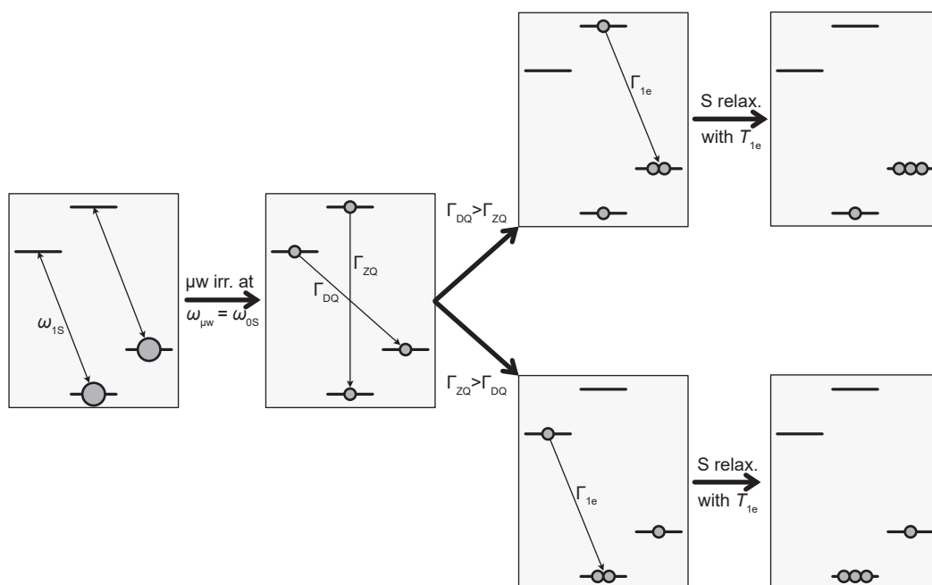
Figure 3.15: Schematic representation of the steps of OE-DNP. \Gamma_{1e} , \Gamma_{ZQ} and \Gamma_{DQ} are the rate of electron spin-lattice relaxation and of ZQ and DQ electron-nucleus cross-relaxation, respectively.
