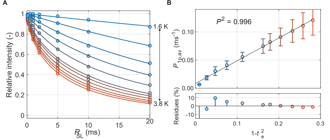
Figure 4.7: A. R_{1\rho}(^1H) measurements at various temperatures measured using the pulse sequence shown in Fig. 4.6A. The measured signal integrals are fitted with Eq. 4.14 shown as dots and lines, respectively. The curves are normalized by the fitted value of I_0 . B. Linear regression of the average relaxation rate R_{1\rho,av} (obtained from the fitted parameters of the curves in Panel A using Eq. 3.34) against 1 - P_e^2 .
