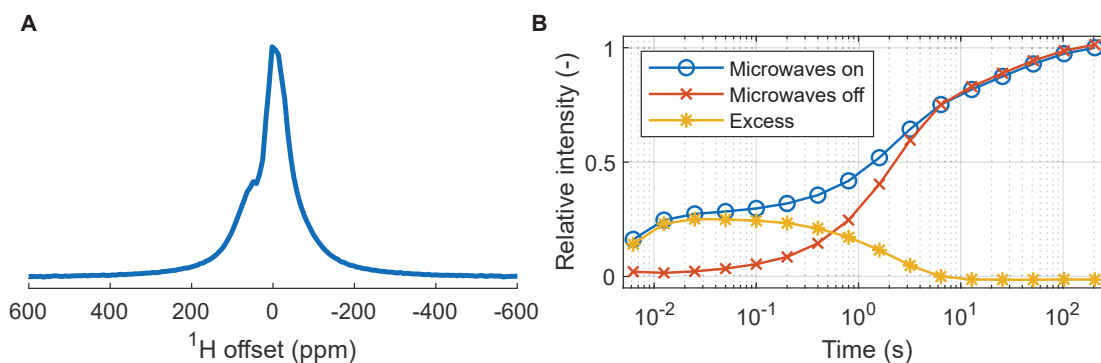
Figure 5.16: A. ^1\text{H} spectrum of 10 mM ASYMPolPOK in 4:6 \text{H}_2\text{O} :glycerol (v/v) at 14.0 T and 100 K under MAS at 8 kHz obtained by DNP. B. Corresponding HypRes curves. Contrary to experiments in static mode at low temperatures, these measurements were obtained with \pi/2 pulses, each point being an individual measurement. Adapted from Ref. [68] according to the terms of the Creative Commons Attribution-NonCommercial 4.0 International Public License.
