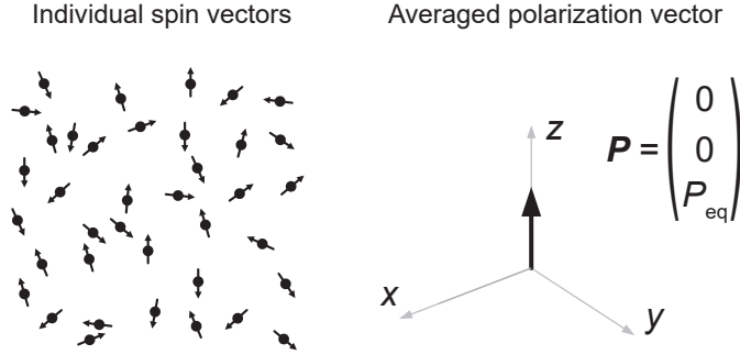
Figure 2.3: Representation of the polarization vector of an ensemble of spins whose average polarization points along the z -axis.
