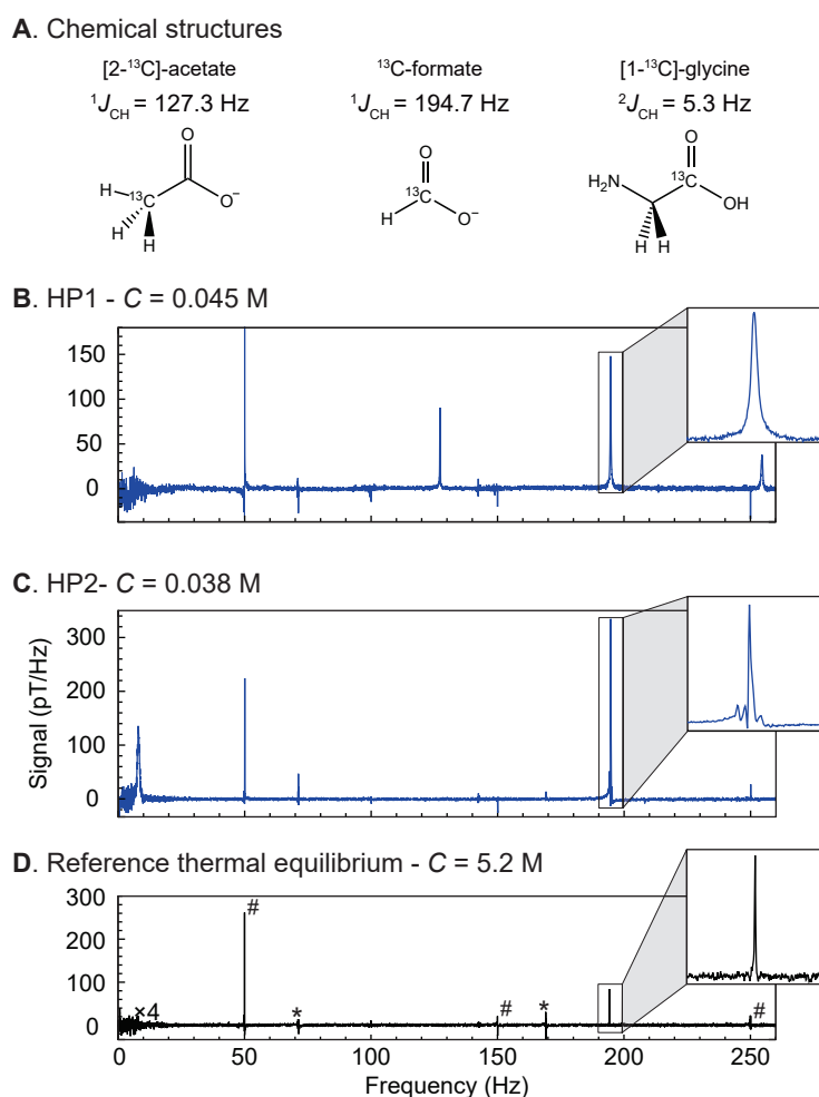
Figure 6.21: A. Chemical structures of the molecules whose signals appear in Panel B-C. B-C. Hyperpolarized ZULF spectra of sample HP1 and HP2, respectively. The concentration of 13 C-formate shown in the title was quantified by 1 H-NMR at 1.88 T. D. Reference signal of 5.2 M 13 C-sodium formate in D 2 O with thermal prepolarization at 2 T. The signal is the sum of 16 scans and is magnified by a factor \times 4 . The hash and asterisk symbols indicate noise peaks arising from the power line at 50 Hz and overtones and that of the probe-laser noise, respectively. The insets in Panel B-D show zooms of the 13 C-formate signal. Adapted with permission from Ref. [223] (Copyright 2023 American Chemical Society).
