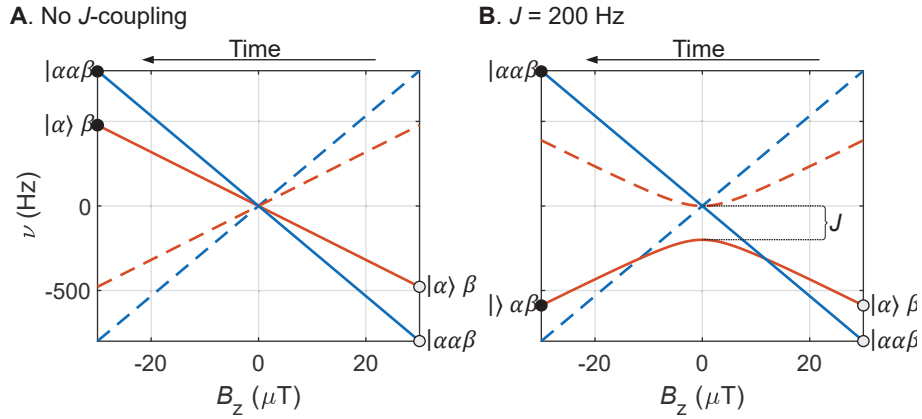
Figure 6.9: A-B. Comparison of the eigenfrequencies of the four levels of a ^1\text{H} - ^{13}\text{C} pair as a function of magnetic field without J -coupling and with J = 200 Hz, respectively. The white and black dots represent the populations of the states before and after the adiabatic field inversion, respectively, assuming initial polarization P(^1\text{H}) = 1 and P(^{13}\text{C}) = 0 .
