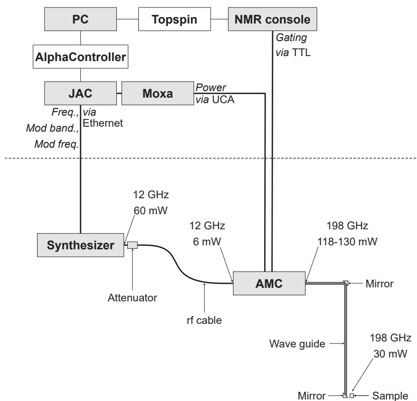
Figure 3.3: Setup of the \mu\text{W} source from the synthesizer to the sample space. The values of the \mu\text{W} power and frequency are given for several stages of transmission. Powers are approximate values, which were measured using different means depending on the stage. The top part of the diagram shows the communication between the control computer and the hardware components via two different softwares, Topspin and AlphaController.
