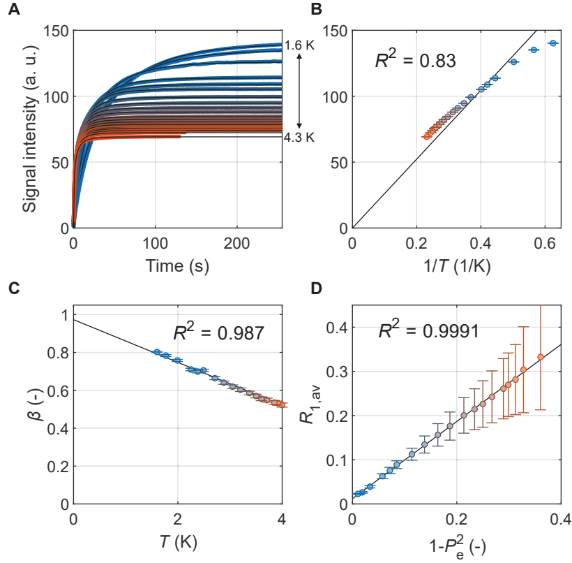
Figure 3.26: A. ^1\text{H} thermal equilibrium build-ups for 28.3 mg of PANI with \chi = 0.2 at 7.05 T between 1.6 and 4.3 K recorded with 1^\circ pulses. The colored and black curves represent the experimental signal intensity over time and stretched exponential fit (see Eq. 3.33), respectively. B. Fitted thermal equilibrium signal intensity obtained from Panel A showed as colored dots as a function of 1/T . The black line is a linear regression of the points (forced to go through 0). C-D. Fitted \beta coefficient and average relaxation rate (obtained from the fit using Eq. 3.34) as a function of temperature, respectively. The colored dots are the values obtained from Panel A and black lines are linear regressions with free y -intercept.
