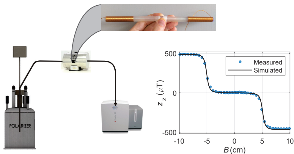
Figure 6.8: Experimental setup, where a ^1\text{H} -dDNP hyperpolarized solution is transferred to a liquid-state spectrometer via a magnetic field inversion chamber, consisting of \mu -metal magnetic shields and a pair of solenoids producing opposing magnetic fields which cancel in the middle.
