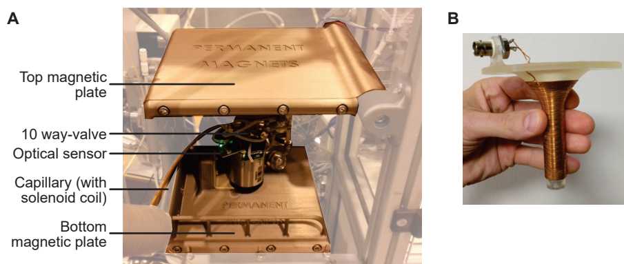
Figure 6.6: A. 10 way-valve of the fast dissolution, transfer, and injection system surrounded by a pair of magnetic plates. The capillary surrounded by a solenoid coil is the output capillary of the dissolution stick. B. Insert of the benchtop spectrometer surrounded by a solenoid coil.
