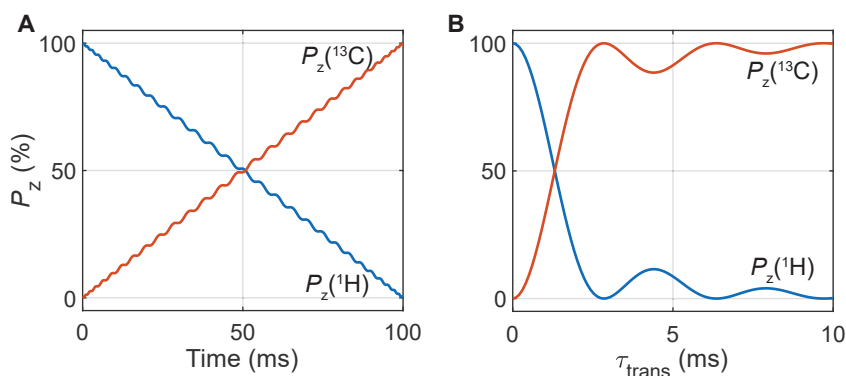
Figure 6.17: A-B. ^1\text{H} and ^{13}\text{C} polarizations along time for a transfer time of 100 ms and as a function of the transfer time, respectively, for ^{13}\text{C} -formate for a field inversion with constant adiabaticity ( \xi_0 dt = 10^{-10} s, B_0 = +385 \mu\text{T} with 200'000 propagation steps).
