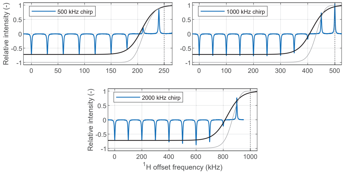
Figure 5.18: Relative inversion efficiency for chirp pulses of 0.5, 1, and 2 MHz inversion width, recorded by moving the center of the pulse. The blue lines are the data points. The vertical black dashed lines represent the theoretical inversion width. The black solid line is a manually fitted hyperbolic tangent function. The gray faint line is the simulated profile. Adapted from Ref. [68] according to the terms of the Creative Commons Attribution-NonCommercial 4.0 International Public License.
