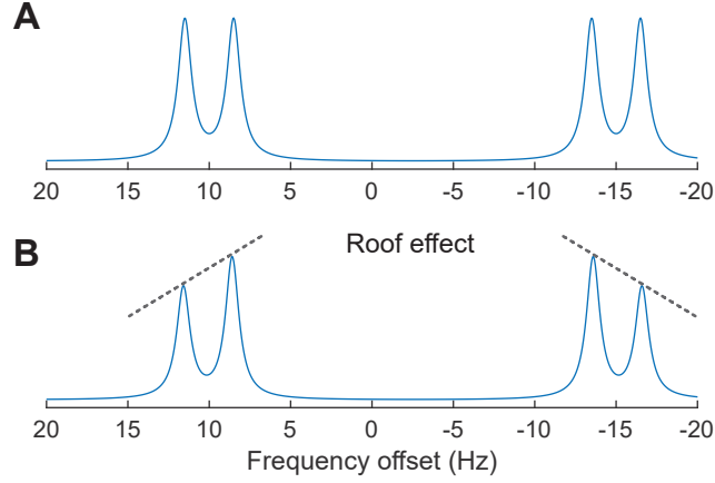
Figure 2.7: Numerical spectrum simulation using the same parameters as in Fig. 2.5 and Fig. 2.6 using the secularized form of J -Hamiltonian (see Eq. 2.112) and the complete form (see Eq. 2.110), respectively.
