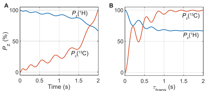
Figure 6.18: A-B. ^1\text{H} and ^{13}\text{C} polarizations along time for a transfer time of 2 s and as a function of the transfer time, respectively, for [1\text{-}^{13}\text{C}] -pyruvate for a field inversion with constant adiabaticity ( \xi_0 dt = 10^{-6} s, B_0 = +4.1 \mu\text{T} with 20'000 propagation steps).
