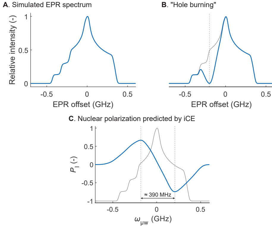
Figure 3.17: A. EasySpin simulation of the EPR spectrum of TEMPOL at 7.05 T with a Lorentzian broadening of 25 MHz using hyperfine coupling parameters A_{xx} = 19.8 MHz, A_{yy} = 22.1 MHz and A_{zz} = 108 MHz and g -tensor parameters g_{xx} = 2.00908 , g_{yy} = 2.00554 and g_{zz} = 2.00233 from Ref. [144]. B. Simulation of a hole burning by \mu w irradiation centered at -0.2 GHz and with a Gaussian profile with a width of FWHM \delta_{1/2} = 150 MHz. The blue and light gray lines represent the EPR spectrum before and after the hole burning, respectively. The dotted vertical line indicates the \mu w frequency. C. Simulated \mu w spectrum obtained using the iCE model in blue, assuming a Boltzmann electron polarization P_{S,eq} = 0.99 . The simulated EPR spectrum is shown for comparison in light gray.
