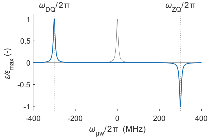
Figure 3.14: Simulated \mu w spectrum (in blue) for a ^1\text{H} spin polarized under SE-DNP at 7.05 T, corresponding to a nuclear Larmor frequency of 300 MHz. The EPR spectrum is shown in light gray, assuming a Lorentzian lineshape h(\omega) with an FWHM \delta_{1/2} = 10 MHz. The dotted vertical lines indicate the frequencies of the ZQ and DQ transitions. The frequency axis is shifted so that \omega_{0S} = 0 .
