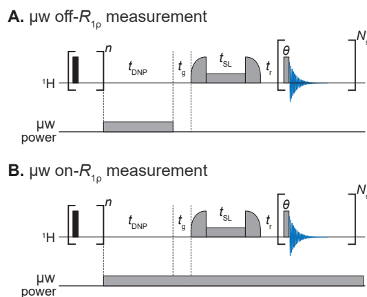
Figure 4.6: A-B. Pulse sequence diagrams for the measurement of R_{1\rho}(^1\text{H}) in the absence of and under \mu\text{w} irradiation, respectively. In Panel A, if R_{1\rho} is to be measured while the electron polarization is at Boltzmann equilibrium, t_g is set to 0.5 s, so that it is large compared to T_{1e} and so the electrons have time to relax between the instant where \mu\text{w} irradiation is gated and the spinlock. The pulse sequence in Panel A is used here for the determination of the relaxation parameters and T_{1e} measurements, whilst that in Panel B is used for the measurement of the EPR spectrum. A single R_{1\rho} measurement typically takes \approx 30 s to record.
