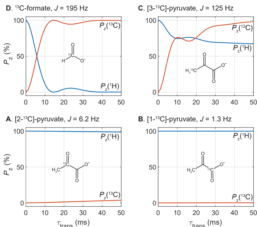
Figure 6.12: Numerical simulations of the final polarizations of ^1\text{H} and ^{13}\text{C} spins as a function of the time of transfer \tau_{\text{trans}} through the inversion chamber with the field profile of Fig. 6.11.
