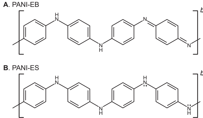
Figure 3.24: A-B. Chemical structures of the repeat units of the polymers PANI-EB and PANI-ES, respectively.
