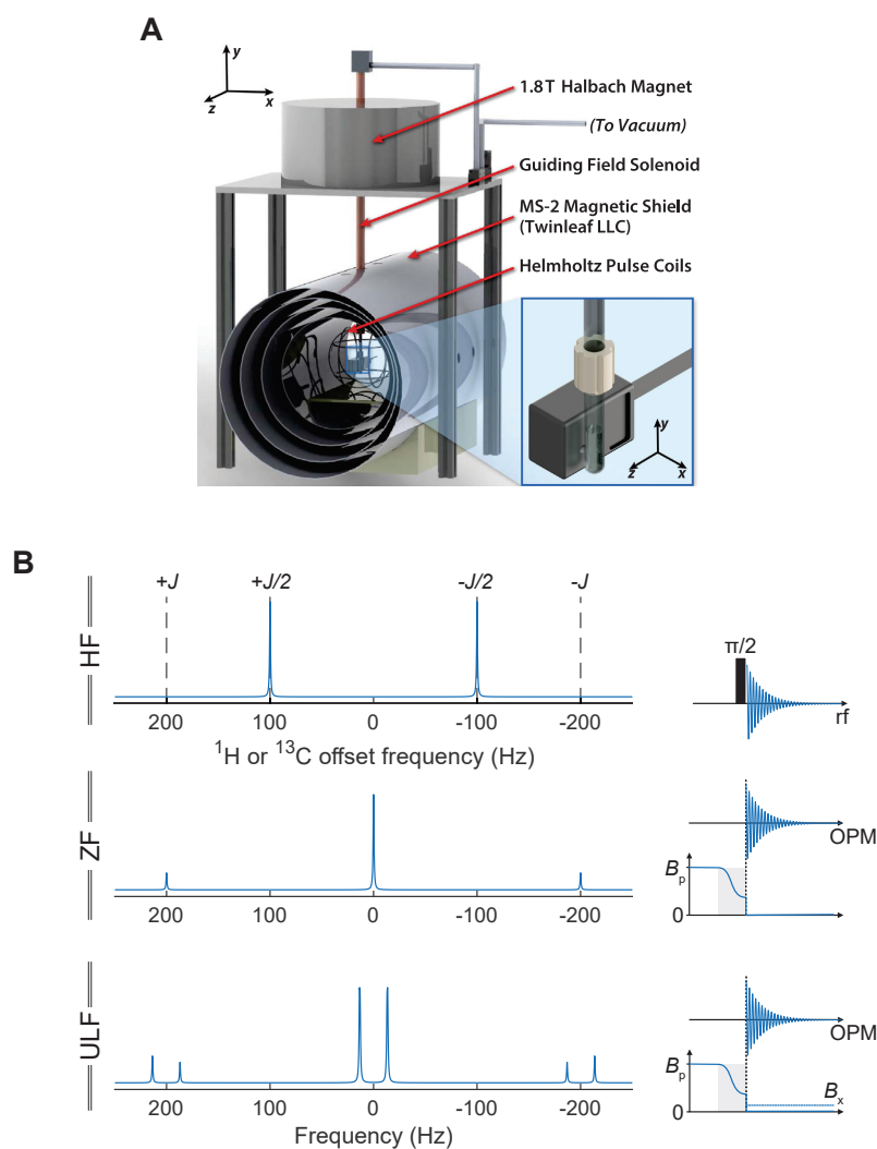
Figure 1.8: A . Typical setup for liquid-state ZULF NMR, reproduced with permission from Ref. [80]. The sample is prepolarized in a permanent magnet in Halbach array, shuttled to the zero-field chamber consisting of commercial magnetic shields, and detected using a commercial OPM. B . Difference between liquid-state NMR spectra at high-field (HF), zero-field (ZF), and ultra low-field (ULF). Simulation of spectra for an XA pair of ^1\text{H} and ^{13}\text{C} spins with a J -coupling J = 200 Hz. The high-field experiment corresponds to ^1\text{H} as well as ^{13}\text{C} detection as it yields the exact same spectrum. The zero-field experiments consist of a sudden transition from high-field to zero-field with initial prepolarization at field B_p . The ultra low-field experiment is the same as that at zero-field except that a small bias field of B_x = 500 nT is applied along the x -axis during detection. The grey squares on the pulse diagrams of the ZULF experiments indicate the moments where the sample is shuttled up and down (the simulation neglects the evolution of the system during the shuttling period). A line broadening of 1 Hz was applied to the FID prior to Fourier transform. Note that the axis convention of Panel A (reproduced with permission from Ref. [80]) is different from that used in this work.
