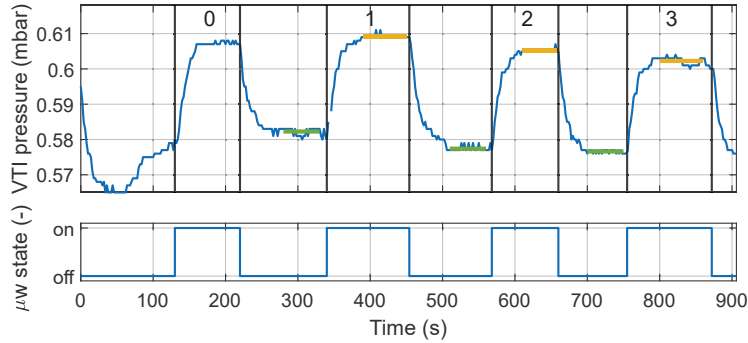
Figure 3.4: Example of measurement of the \mu\text{w} power deposited in the VTI realized by monitoring the change of pressure upon switching on \mu\text{w} irradiation in the helium bath at \approx 1.16 K. The green and yellow horizontal lines represent the base pressure and the pressure under \mu\text{w} irradiation, respectively, for the three consecutive measurements. In this case, the pressure difference was found to be 0.027 \pm 0.001 mbar, corresponding to a deposited power of 14.2 \pm 0.5 mW.
