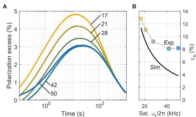
Figure 5.11: A. HypRes at 3.8 K after DNP in positive mode using a range of nutation frequencies for the \pi/2 saturation pulses (marked next to the curves in kHz). B. Size of the hidden reservoir measured experimentally (colored dots) using the maximum of the HypRes curves of panel A (see Eq. 5.27) and simulated using the procedure described above (black solid line). Adapted from Ref. [68] according to the terms of the Creative Commons Attribution-NonCommercial 4.0 International Public License.
