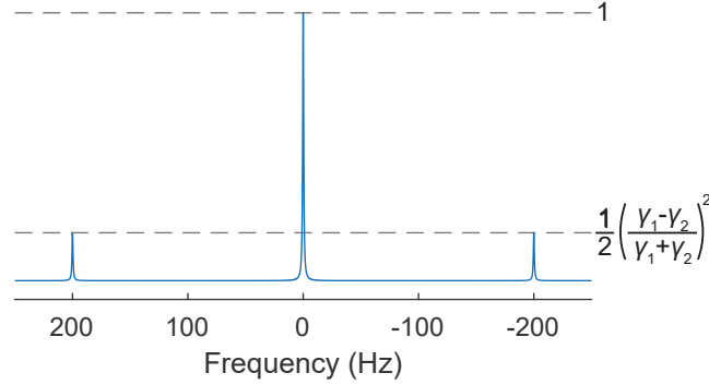
Figure 2.9: Spectrum simulation at zero-field for a pair of ^1\text{H} and ^{13}\text{C} spins with a J -coupling of 200 Hz. Simulation with 256 time increments of 10 ms and 1 Hz of line broadening and zero-filling to 1024 points prior to Fourier transform. The horizontal dashed lines indicate the ratio of the signals expected from the analytical solutions (see Eq. 2.130). The extra factor of 1/2 accounts for the fact the oscillating signal is split into positive and negative components while not for the stationary part.
