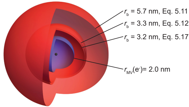
Figure 5.3: Representation of the spin diffusion barrier r_b for the solvent ^1\text{H} spins in DNP juice doped with 50 mM TEMPOL according to Blumberg, [173] Khutsishvili, [174] and Hovav et al. [190, 69] (see Eq. 5.11, 5.12 and 5.17, respectively) represented as red spheres compared with the mean volume per electron spin r_{\text{MV}}(e^-) represented as a blue sphere. The black sphere represents the electron. Adapted from Ref. [68] according to the terms of the Creative Commons Attribution-NonCommercial 4.0 International Public License.
