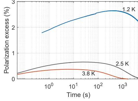
Figure 5.8: HypRes experiment in 2:3 H 2 O:glycerol ( v/v ), i.e., the fully protonated equivalent of DNP juice, doped with 50 mM TEMPOL. Adapted from Ref. [68] according to the terms of the Creative Commons Attribution-NonCommercial 4.0 International Public License.
