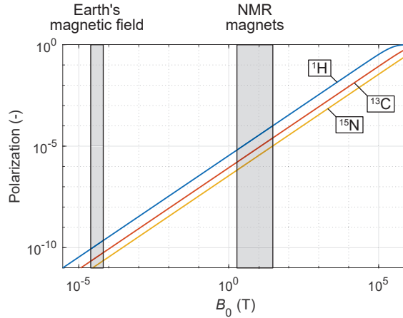
Figure 1.1: Effect of the magnetic field strength on nuclear polarization for three commonly used isotopes at a temperature of 298 K. The grey boxes indicate the span of the Earth's magnetic field and that of NMR magnets, from benchtop spectrometers using permanent magnets to the highest available high-resolution magnet.
