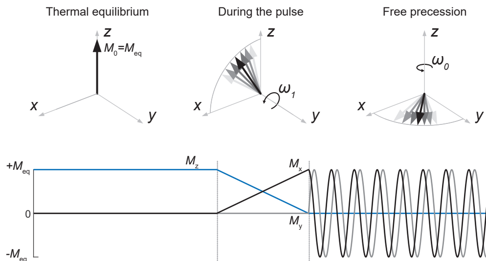
Figure 2.4: Magnetization of an ensemble of spin 1/2 (represented by a black arrow) tilted from the thermal equilibrium position to the transverse plane by a \pi/2 pulse along the y -axis. The magnetization vector then starts precessing about the z -axis under the Zeeman Hamiltonian.
