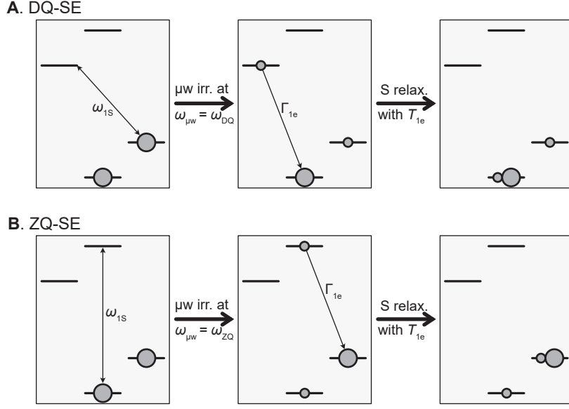
Figure 3.13: A-B. Steps of the SE-DNP mechanism for the DQ and ZQ transitions, respectively. \Gamma_{1e} is the rate of electron spin-lattice relaxation.
