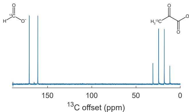
Figure 6.15: Hyperpolarized ^{13}\text{C} signal spectrum detected at 1.88 T using a single 5^\circ pulse obtained after ^1\text{H} -dDNP experiment by an adiabatic field inversion. The sample initially contained \approx 0.4 M of ^{13}\text{C} -formate, [3\text{-}^{13}\text{C}] -pyruvate, [2\text{-}^{13}\text{C}] -pyruvate and [1\text{-}^{13}\text{C}] -pyruvate but only ^{13}\text{C} -formate and [3\text{-}^{13}\text{C}] -pyruvate are visible on the spectrum.
