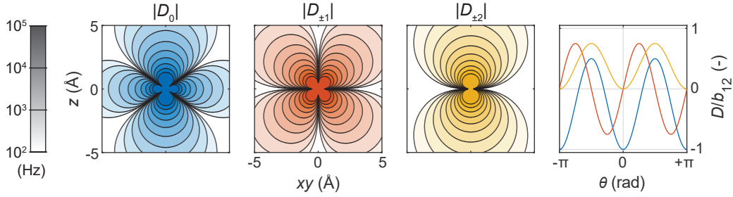
Figure 2.10: Spatial dependence of dipolar interaction for a pair of ^1\text{H} spins, with one spin located at the origin, expressed in Hz and as absolute values decomposed into spherical harmonics. The right plot shows the angular dependence of the dipolar coupling constants in relative intensity, for \phi = 0 .
