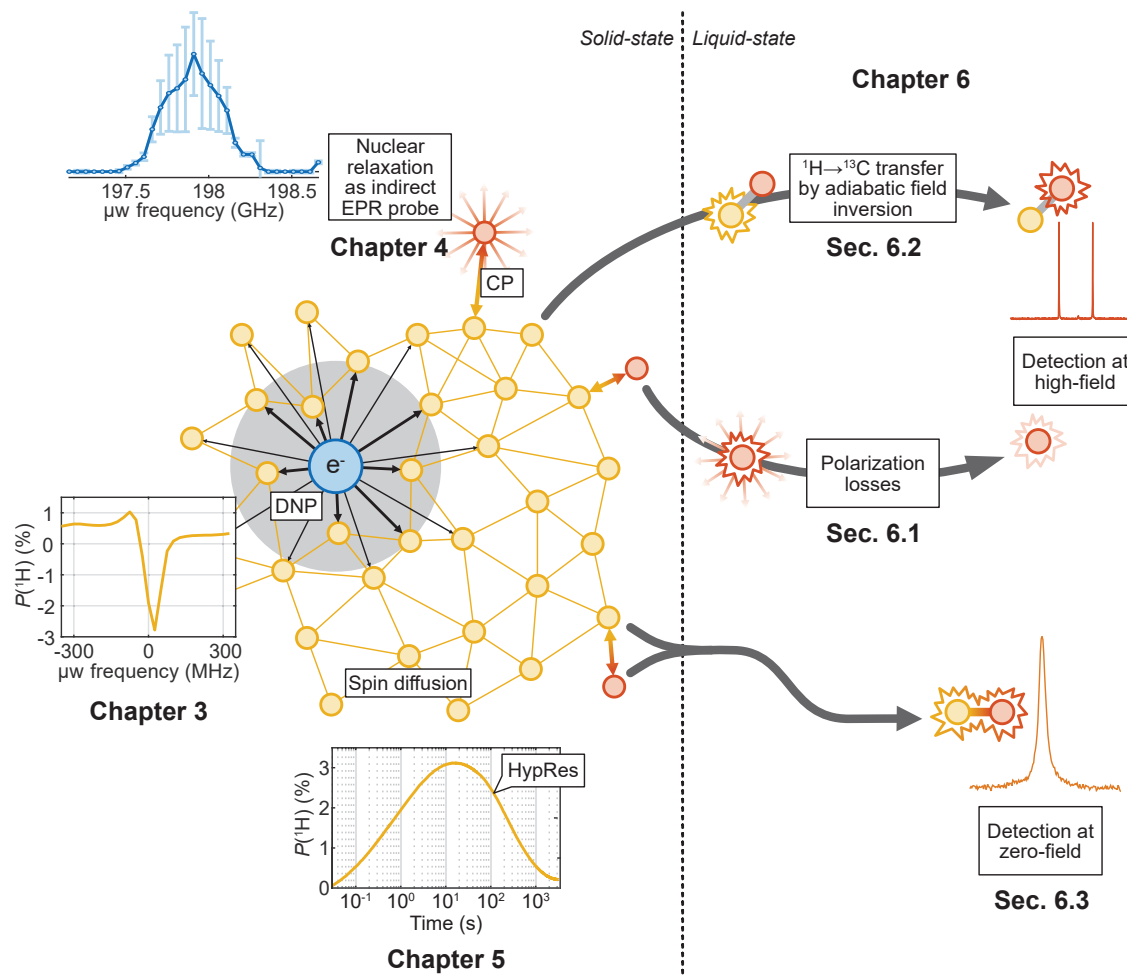
Figure 1.9: Schematic representation of electron and nuclear spins and the polarization transfers between them in dDNP experiments and in hyperpolarized liquid-state NMR at ZULF. The blue circle represents an electron spin (with e^- written in its center) interacting with surrounding ^1\text{H} spins. The gray circle around the electron spin represents the area within the spin diffusion barrier. Red circles represent ^{13}\text{C} spins, which are polarized either by CP in the solid-state or by adiabatic field inversion in the liquid-state.
