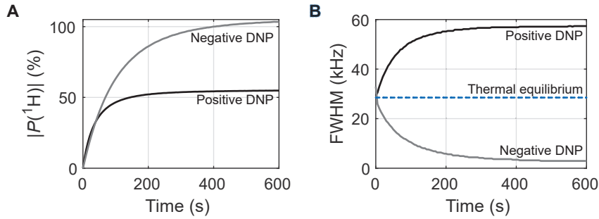
Figure 3.8: A-B. Absolute polarization and FWHM, respectively, for 100 \mu\text{l} of DNP juice doped with 50 mM TEMPOL under positive and negative DNP.
