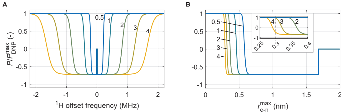
Figure 5.19: A. Estimated relative polarization profiles of the ^1\text{H} spins at the end of the preparation as a function of Larmor frequency shift taking into account the imperfection of the pulses. The dip near zero is due to the narrow band saturation at the end of the preparation phase. B. Estimated relative polarization profiles of the ^1\text{H} spins at the end of the preparation as a function of the distance to the electron spin, converted from panel A using Eq. 5.41. The numbers next to the curves indicate the theoretical widths of the inversion pulses in MHz. Adapted from Ref. [68] according to the terms of the Creative Commons Attribution-NonCommercial 4.0 International Public License.
