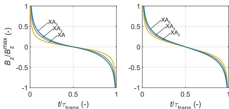
Figure 6.16: Normalized constant adiabaticity field profiles for ^{13}\text{C} - ^1\text{H} \text{XA}_n spin systems for n between 1 and 6.
