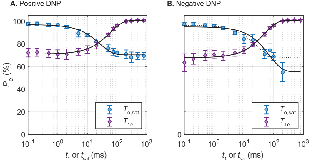
Figure 4.5: A-B. Measurement of the time constant of the electron spin-lattice relaxation time T_{1e} and the electron saturation time T_{e,sat} using the pulse sequences in Fig. 4.4, under positive and negative DNP, respectively. Colored dots and black solid lines correspond to measured electron polarizations and model curves (see Eq. 4.13), respectively. The model shown as a dotted line on Panel B was performed fixing P_\infty to the value of P_0 obtained from the T_{1e} measurement under negative DNP. Each curve was recorded in 30 – 35 min.
