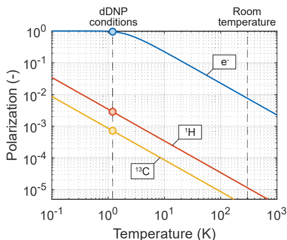
Figure 1.6: Electron spin polarization as a function of temperature at a magnetic field of 3.35 T (i.e. that used for the first reported dDNP experiment), compared with the nuclear spin polarization of ^1\text{H} and ^{13}\text{C} spins.
