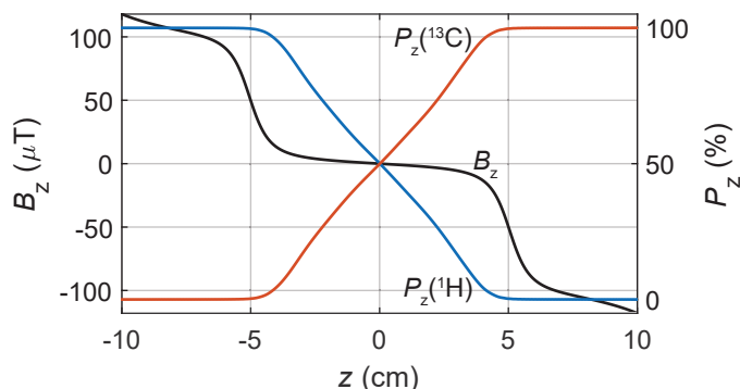
Figure 6.11: Simulated field profile inside the inversion chamber and ^1\text{H} and ^{13}\text{C} polarizations along the transfer in black, assuming a J -coupling of 195 Hz and initial polarization P(^1\text{H}) = 1 and P(^{13}\text{C}) = 0 , corresponding to ^{13}\text{C} -formate in \text{D}_2\text{O} . Details of the spin dynamical simulation are given in the text. Details on the simulation of the field profile are given in Sec. 6.2.3
