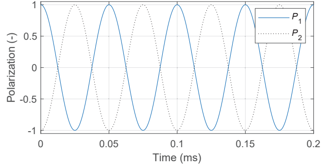
Figure 2.12: Numerical simulation of the polarization along the z -axis for a pair of dipolar coupled spins with a coupling of 20 kHz along time initially in the |\alpha\beta\rangle state. Propagation over 1000 time increment of 0.2 ms.
