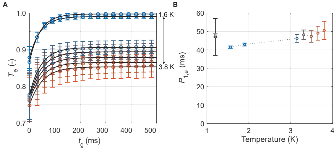
Figure 4.8: A. T_{1e} measurement via R_{1\rho}({}^1\text{H}) . Colored dots represent individual R_{1\rho} measurement using the pulse sequence of Fig. 4.6A converted into electron polarization using Eq. 4.16 and the rates obtained in Fig. 4.7B. The obtained electron polarizations as a function of the gating delay t_g are fitted with the monoexponential model of Eq. 4.13. B. Electron spin-lattice relaxation time constant T_{1e} obtained in Panel A plotted against temperature as colored dots. The black and gray dots are the values that we measured using R_2^*({}^{13}\text{C}) (see Sec. 4.2.3) and the value measured by Bornet et al. at 6.7 T using R_{1\rho}({}^1\text{H}) , [48] respectively. One T_{1e} measurement typically takes \approx 8 s.
