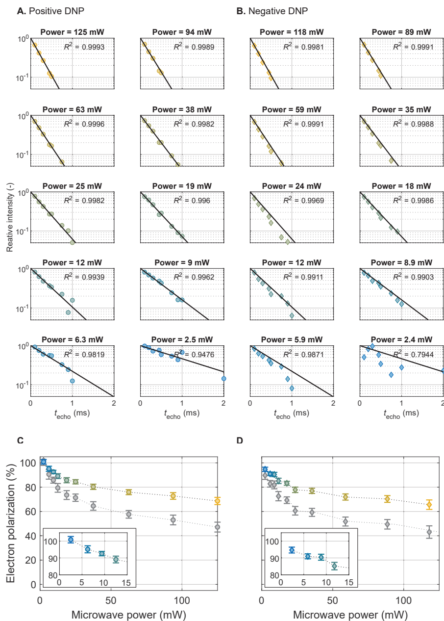
Figure 4.3: A-B. R_2^*(^{13}\text{C}) measurement by solid echo under \mu\text{W} irradiation at the optimal frequency for positive and negative DNP, respectively, after ^1\text{H} DNP and ^1\text{H} \rightarrow ^{13}\text{C} CP, as described on Fig. 4.1B, at various \mu\text{W} powers, fitted with Eq. 4.10, shown as colored dots and black lines, respectively. The curves are normalized by the fitted value of I_0 . C-D. Polarization of the electron under positive and negative DNP, respectively, as a function of \mu\text{W} power inferred from the relaxation rates obtained from the data of Panels A and B. The colored and gray symbol represents polarization values inferred using Eq. 4.8 and Borner et al. 's Eq. 4.9, respectively. Each R_2^* measurement took 10-20 min to record.
