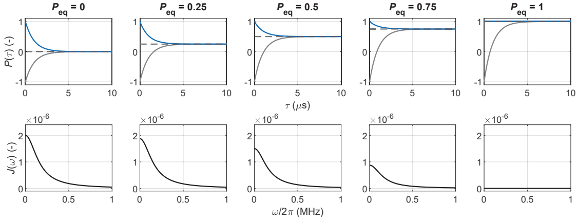
Figure 2.14: Polarization over time P(\tau) used to calculate the autocorrelation function (see Eq. 2.149) and corresponding spectral density functions of the electron spin state for a correlation time constant of 1 \mu s for various equilibrium polarizations P_{eq} . The blue and gray curves represent the polarization of the electron spin state when in |\beta\rangle or |\alpha\rangle state at time t = 0 , respectively. The horizontal dashed lines represent the equilibrium polarizations.
