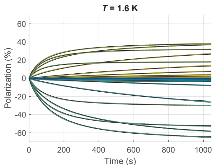
Figure 3.21: Raw results of the \mu w spectrum for 50 mM TEMPOL in DNP juice at 1.6 K, consisting of a series of DNP build-up curves for various \mu w frequencies. The measured polarization along time is fitted with a stretched exponential curve (see Eq. 3.33), represented by colored and black curves, respectively.
