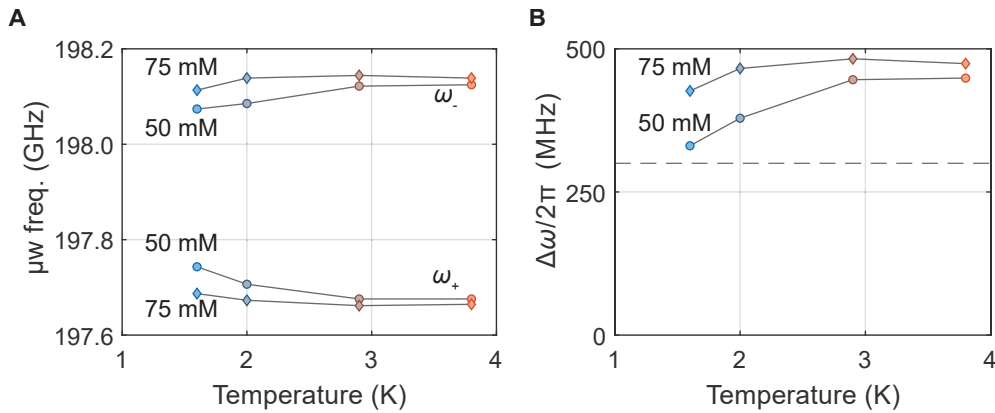
Figure 3.23: A. Optimal frequency for negative and positive DNP as a function of temperature, computed from the spline interpolation in Fig. 3.22A-B. B. Difference between the optima shown in Panel A. The ^1\text{H} Larmor frequency is shown as a horizontal dashed line.
