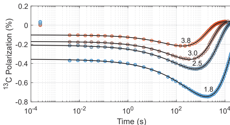
Figure 5.13: ^{13}\text{C} -HypRes experiment in neat [1-^{13}\text{C}] -pyruvic acid doped with 25 mM trityl OX063 detected with 5^\circ pulses at various temperatures (shown next to the curves in K) after DNP in negative mode. Colored dots and black curves represent experimental data and stretched biexponential fits (see Eq. 5.36), respectively.
