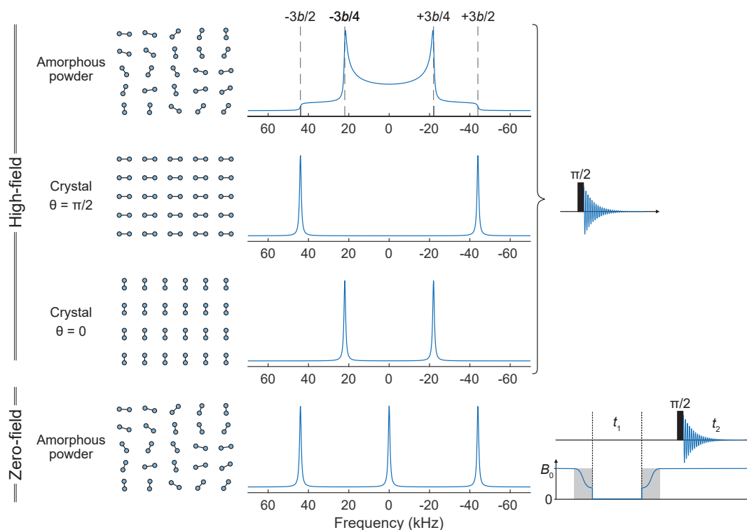
Figure 1.7: Difference between solid-state NMR spectra at high-field and at zero-field. Simulation of spectra for an A_2 pair of ^1\text{H} spins with an internuclear distance of 1.6 \text{ \AA} , corresponding to a dipole coupling constant of b = 29.3 \text{ kHz} . The high-field experiment is a simple pulse-acquire experiment while the zero-field is a field-cycling experiment with prepolarization and detection at high-field and evolution at zero-field. High-field experiments were simulated for three cases: an amorphous powder and two crystalline samples, with the internuclear vector, either orthogonal or colinear with the magnetic field ( \theta = 0 or \pi/2 , respectively). The zero-field experiment was simulated for an amorphous powder. The grey squares on the pulse diagrams of the zero-field experiment indicate the moments where the sample is shuttled up and down. The molecular orientations were averaged over 1000 constant increments of the angle between the molecular vector and the magnetic field, from 0 to \pi . A line broadening of 1 \text{ kHz} was applied to the simulated FID prior to Fourier transform.
