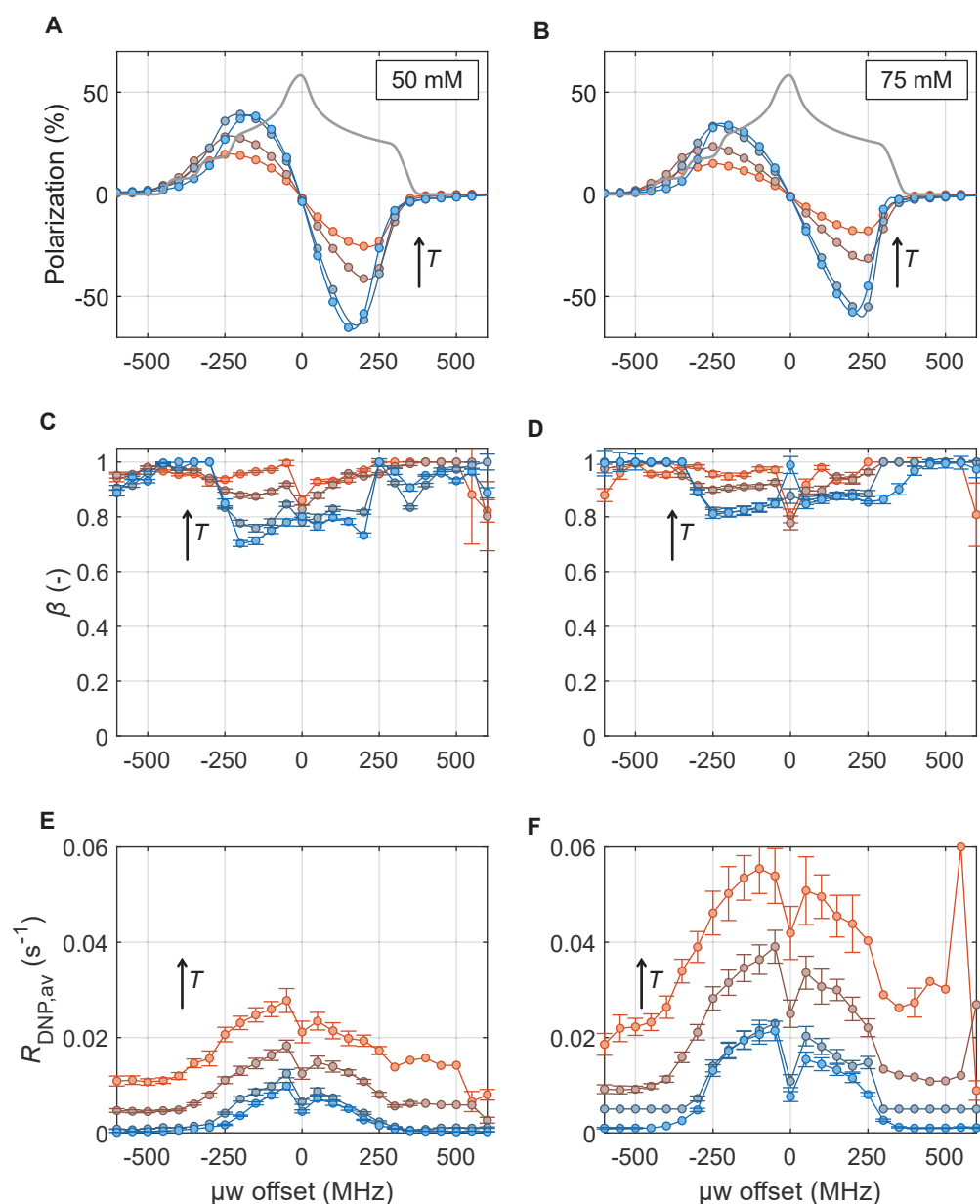
Figure 3.22: A-B. \mu_w spectra at 1.6, 2.9, 3.0, and 3.8 K for DNP juice doped with 50 and 75 mM TEMPOL, respectively. The maximum recorded polarization is shown as colored points together with a spline interpolation (colored lines). The simulated spectrum of TEMPOL is shown for comparison as a gray line, using the same simulation parameters as in Fig. 3.17. C-D. Corresponding fitted values of \beta coefficient E-F. Corresponding values of R_{\text{DNP,av}} obtained from the fitted values using Eq. 3.34.
