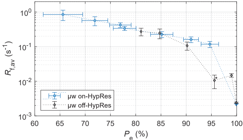
Figure 5.24: Average polarization flow rate R_{f,av} between the hidden and visible ^1\text{H} spins as a function of the electron polarization P_e obtained by fitting the phenomenological model of Eq. 5.36 to \mu\text{w} on- and off-HypRes curves. The data point indicated with a * symbol corresponds to the \mu\text{w} off-HypRes at 2.5 K, for which the phenomenological model gave a poor fit ( R^2 = 0.93 , compared with R^2 > 0.98 for all other curves, see Fig. 5.23). The values of P_e in the case of \mu\text{w} off-HypRes experiments were obtained by conversion from temperature using Boltzmann law (see Eq. 1.3). The values of P_e in the case of \mu\text{w} on-HypRes experiments were obtained by monitoring the change in transverse relaxation rate of ^{13}\text{C} spins R_2^*(^{13}\text{C}) upon switching on \mu\text{w} irradiation (see Sec. 4.2 and Fig. 4.3) on the same sample.
