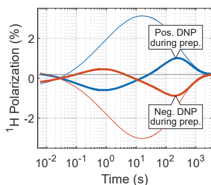
Figure 5.5: A-C. Pulse sequence diagrams of HypRes experiments. D-E. Typical results of experiments of Panels B and C, respectively, on DNP juice doped with 50 mM TEMPOL. The faint lines are the results of experiments of Panel A on the same sample and in the same conditions, shown for comparison.
