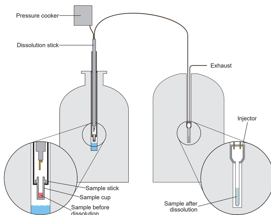
Figure 6.1: Diagram of the main components of the gas-driven dissolution setup from the polarizer to the liquid-state spectrometer (from left to right), represented just before the sample stick is connected to the sample cup when the sample has already been lifted up above the liquid helium bath.
