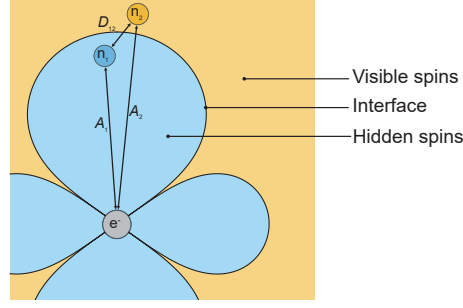
Figure 5.25: Schematic representation of the hidden and visible nuclear spins interacting with the electron spin through the hyperfine interaction with intensities A_{zz1} and A_{zz2} . The two nuclei interact together with the dipole-dipole coupling constant D_{12} .
