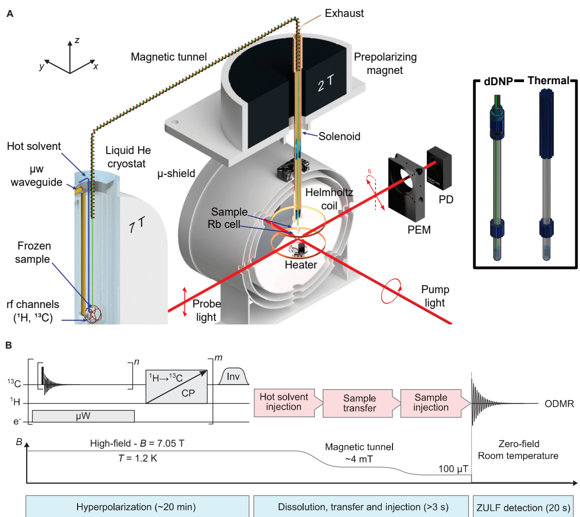
Figure 6.20: A-B Schematic representation of the experimental setup and sequence for dDNP-ZULF experiments, respectively. The inset in Panel A shows the NMR tube in the dDNP injector and that used for pneumatic shuttling in field cycling experiments. Adapted with permission from Ref. [223] (Copyright 2023 American Chemical Society).
