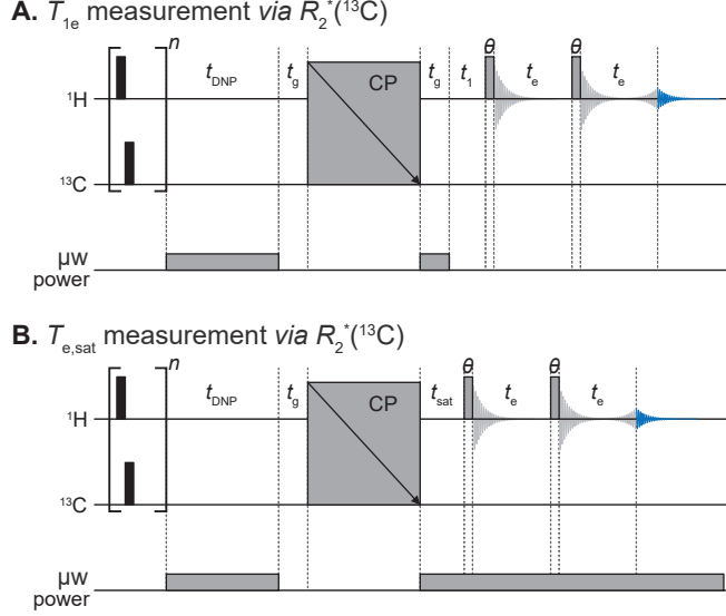
Figure 4.4: A-B. Pulse sequences for the measurement of the time constant of the electron spin-lattice relaxation T_{1e} and the electron saturation T_{e,sat} , respectively. Gating delay t_g is chosen to be five times T_{1e} and T_{e,sat} . The measurement is repeated n_1 \times n_e times and n_1 \times n_{sat} times for sequence A and B, respectively, where n_1 , n_e and n_{sat} are the numbers of increments of t_1 , t_e and t_{sat} , respectively. All other symbols have the same meaning as those in Fig. 4.1. A single R_2^* measurement typically takes \approx 2 min to record.
