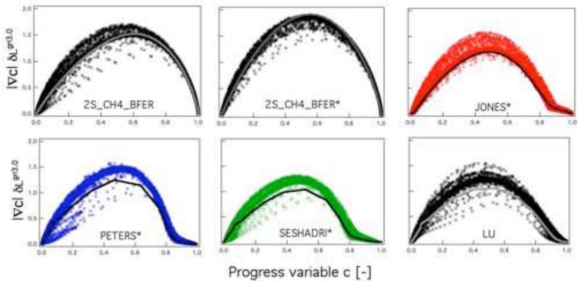
Figure 4.7 - Instantaneous magnitude of progress variable gradient normalized by the laminar flame speed \delta_L^{GRI3.0} of the detailed GRI3.0 mechanism for the flame/vortex configuration at t = 0.55 ms. Comparison between the reduced mechanisms. Lines correspond to results for an unstrained laminar flame. (Section 3.2.2)
