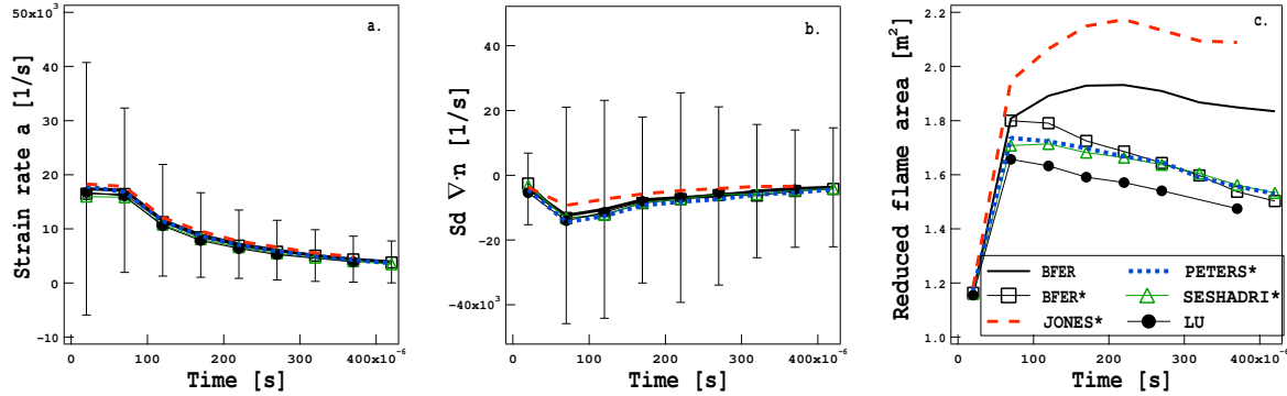
Figure 4.19 - Temporal evolution of mean strain rate (a.), mean curvature Sd \nabla \cdot \mathbf{n} (b.) and reduced area of the flame surface (c.) for different chemical mechanisms. Error-bars indicate the RMS values.
