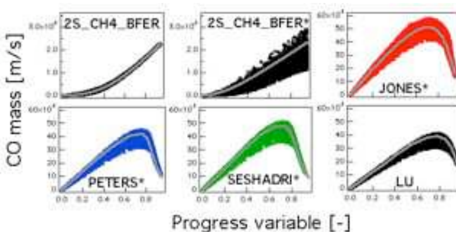
Figure 4.27 - Instantaneous CO mass fraction as a function of progress variable at t = 0.07 ms. Comparison between the six reduced mechanisms. Solid lines correspond to results for an unstrained laminar flame.
