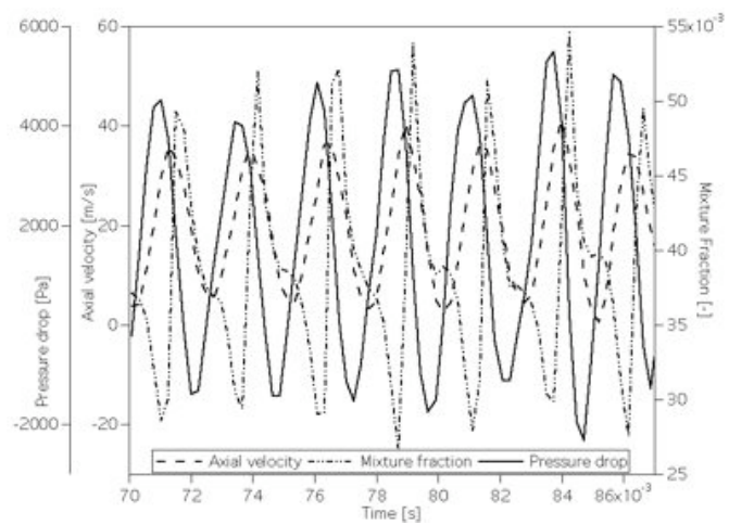
Figure 6.20 - Temporal evolution of the pressure drop (solid line), axial velocity (dashed line) and mixture fraction (dotted-dashed line) in the swirler (probe I) for the 'pulsating' flame ( \phi = 0.7 , case D).
