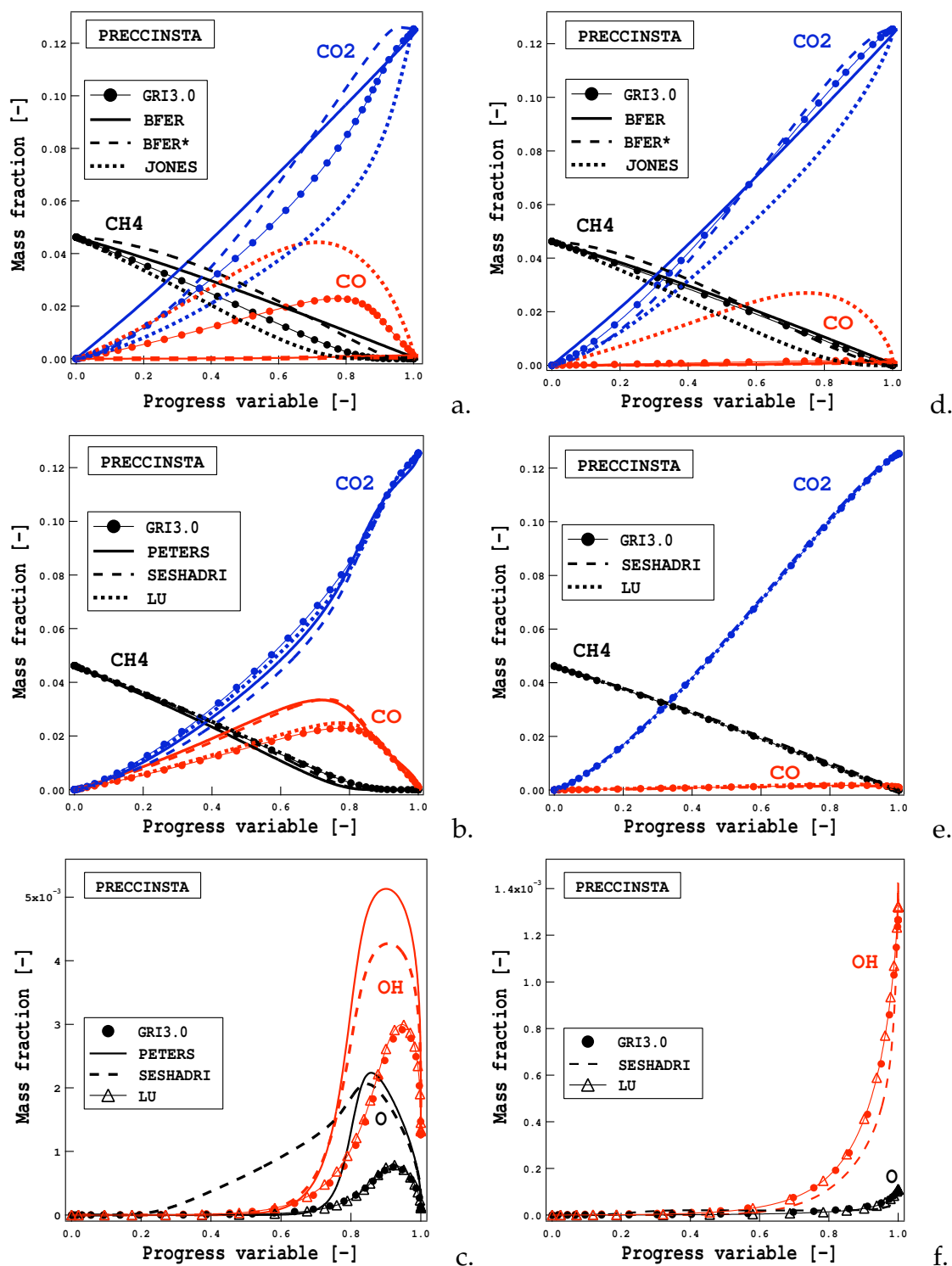
Figure 3.21 - Species profiles for a premixed strained methane/air flame at \phi = 0.83 , T_f = 320 K and P = 1 atm for (a-c) a = 2000 s ^{-1} and (d-f) a = 20000 s ^{-1} . Comparison between the reduced mechanisms and the GRI3.0 detailed scheme. Profiles of radical species are provided for the analytical mechanisms only.
