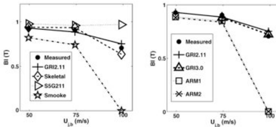
Figure 6 - Burning indices of temperature versus jet velocity for the Barlow and Frank flames D, E and F [12] calculated by Cao and Pope [34]. Comparison between experimental data and seven chemical mechanisms.
