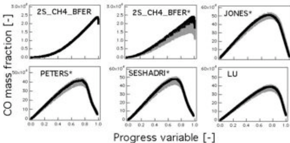
Figure 4.13 - CO mass fraction as function of the progress variable. Instantaneous results at the initial time t = 0 s (black) and the time t = 55 \mu s (grey).
