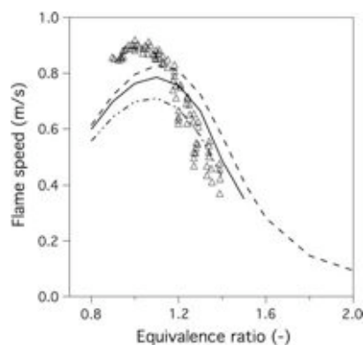
Fig. 2. Flame speed versus equivalence ratio at fresh gas temperature T_f = 473 K and pressure P = 1 atm. Comparison between the DAGAUT detailed mechanism [41] (---), the EL-BAKALI_RISTORI detailed mechanism [57] (—), the LUCHE skeletal mechanism [40] (---), and the experimental results [39] ( \Delta ).
