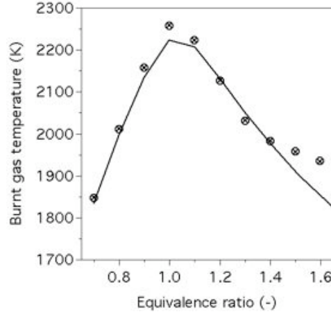
Figure 6.4 - Burnt gas temperature versus equivalence ratio. Comparison between GRI3.0 mechanism (—), equilibrium results (×) and 2S_CH4_BFER scheme (○) at pressure P = 1 \text{ atm} and fresh gas temperature T_f = 300 \text{ K} .
