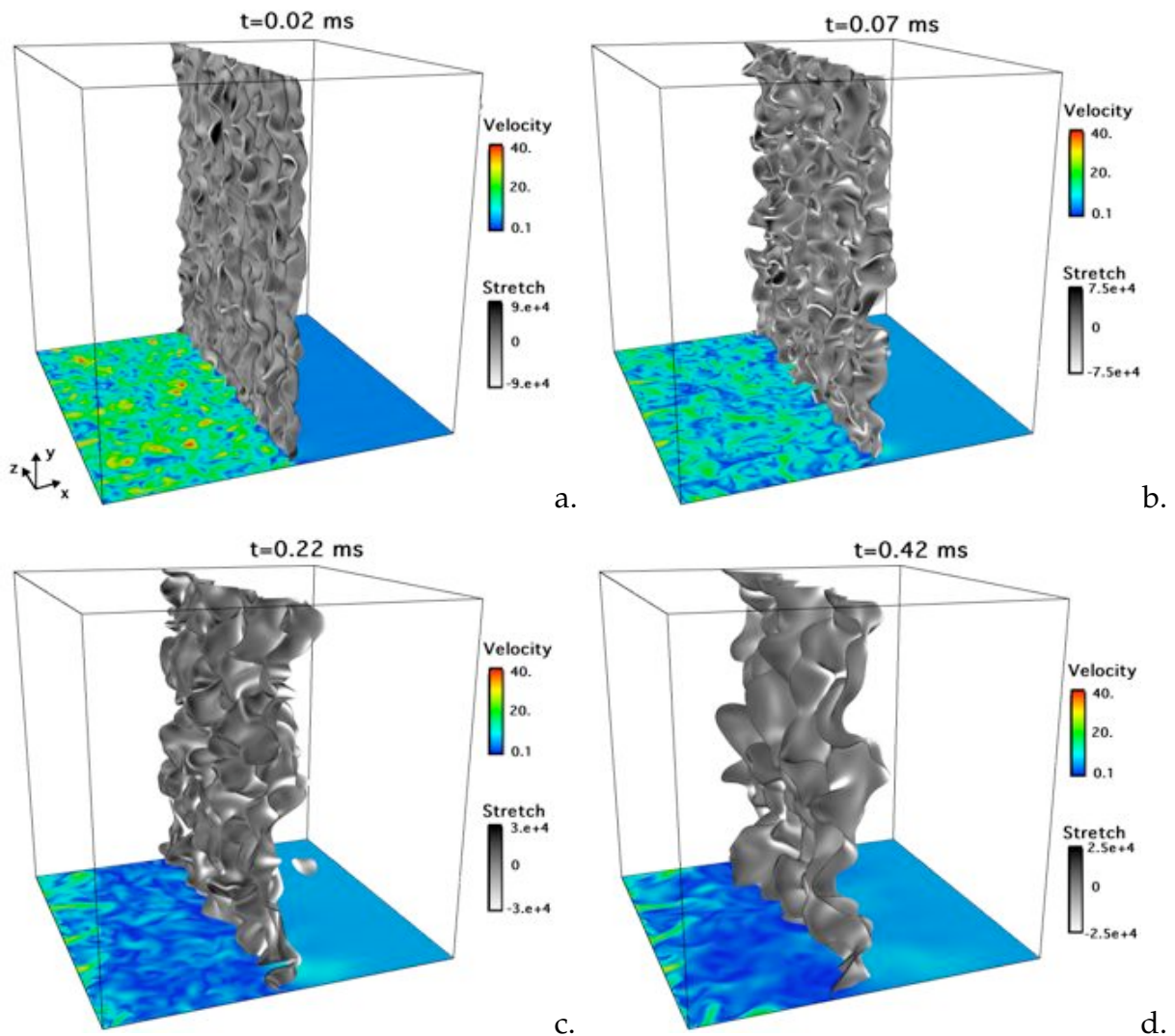
Figure 4.18 - DNS of a premixed flame interacting with a three-dimensional HIT using the 2S_CH4_BFER mechanism at four increasing times: a) t = 0.020 ms, a) t = 0.070 ms, a) t = 0.220 ms and a) t = 0.420 ms. The isosurface of progress variable c = 0.65 identifying the flame surface is colored by stretch. The velocity field is displayed in the bottom plane.
