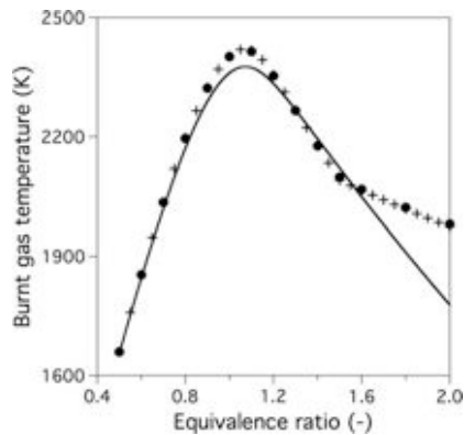
Fig. 9. Burnt gas temperature versus equivalence ratio. Comparison between LUCHE skeletal mechanism (—), equilibrium results (×) and 2S_KERO_BFER scheme (●) scheme at pressure P = 1 atm and fresh gas temperature T_f = 473 K.
