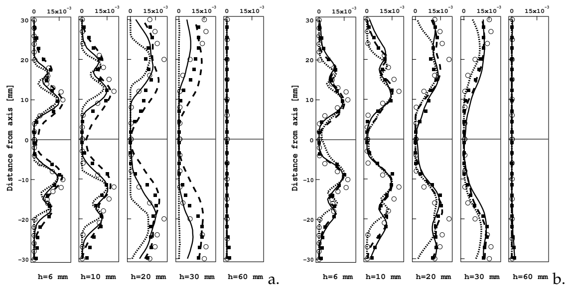
Figure 5.15 - Fluctuating CH_4 profiles at five sections in the chamber. The experimental ( \circ ) and LU ( \blacksquare ) results are compared to numerical data for the other mechanisms: a) 2S\_CH4\_BFER (—), 2S\_CH4\_BFER^* (---) and JONES (.....) b) PETERS (—), SESHADRI (---) and FPI_TTC* (.....).
