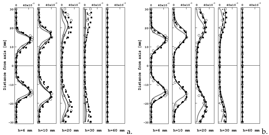
Figure 5.14 - Mean CH_4 profiles at five sections in the chamber. The experimental ( \circ ) and LU ( \blacksquare ) results are compared to numerical data for the other mechanisms: a) 2S\_CH4\_BFER (—), 2S\_CH4\_BFER^* (---) and JONES (.....) b) PETERS (—), SESHADRI (---) and FPI_TTC* (.....).
