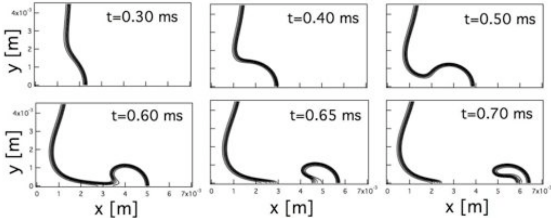
Figure 4.2 - Time series of temperature isocontours for the flame/vortex interaction obtained with the 2S_CH4_BFER mechanism. Contour lines are plotted every 200 K from 1000 K to 2000 K.
