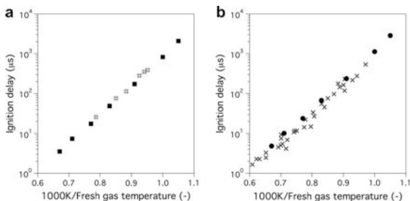
Fig. 10. Ignition delay versus inverse of fresh gas temperature for a stoichiometric flame at pressure P = 10 atm (a) and P = 20 atm (b). Comparison between experimental data [41] (# and \times respectively) and 2S_KERO_BFER scheme predictions (■ and ●).
