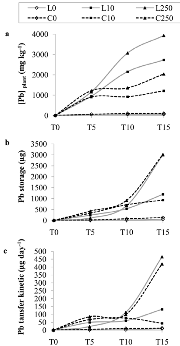
Fig. 2 (a) Pb concentration ( [Pb]_{plant} , \text{mg kg}^{-1} ), (b) Pb storage ( \mu\text{g} ) and (c) Pb transfer kinetic ( \mu\text{g day}^{-1} ) in lettuces and cabbages exposed to PbO by foliar way (L0, L10 and L250 (and C0, C10 and C250) correspond to respectively 0, 10 and 250 mg of PbO deposited on lettuce (cabbage)) to various exposure durations (T0, T5, T10 and T15). Values are expressed as the mean of 4 replicates for each treatment.
