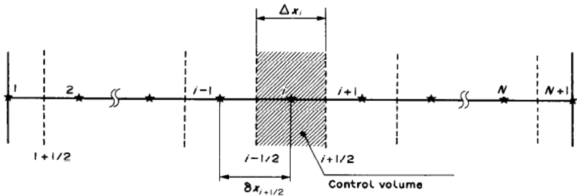
Figure 3.6 Discretization of the calculation domain
