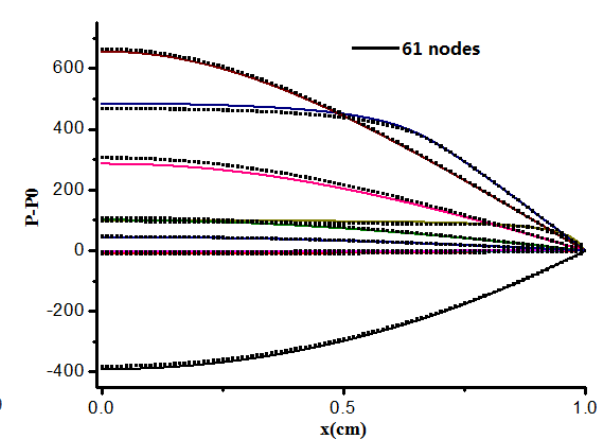
Figure 3.11 Pressures of 61 nodes vs 101 nodes
