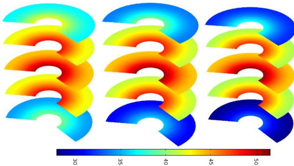
Figure 6.12 Comparison of temperature distributions of different slices of samples heated by different values of h_m : 0.004 (left), 0.008 (middle), 0.012 (right).
