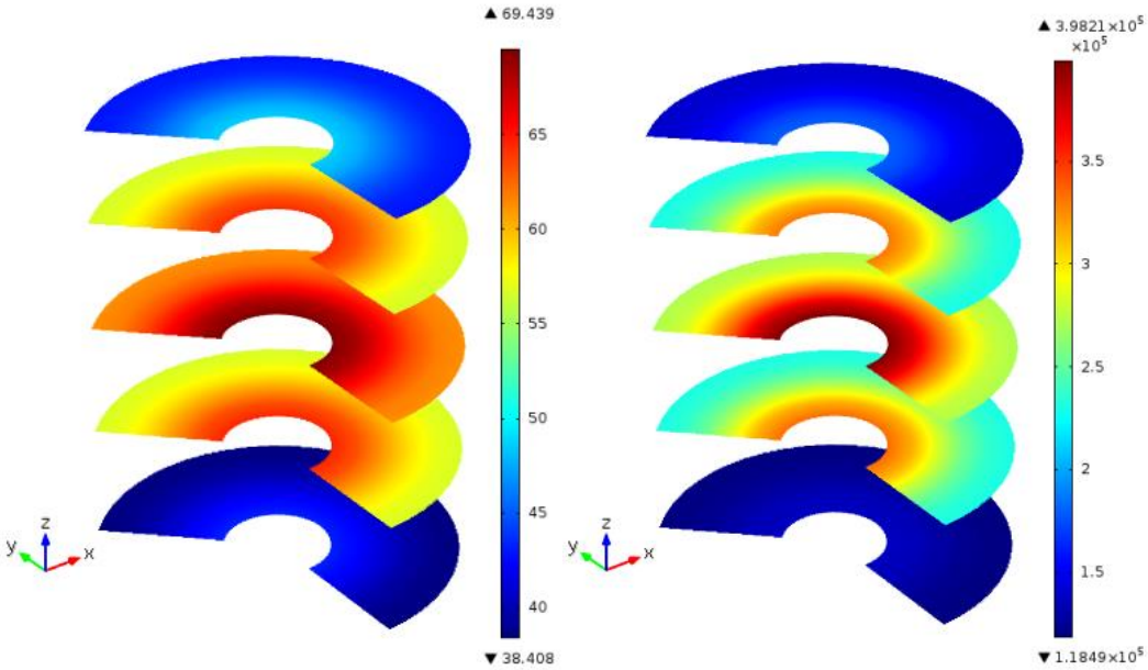
Figure 5.34 Cross-sectional distribution of temperature (left) and pressure (right) after processing 16 cycles
