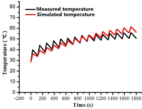
Figure 5.11 Temperature changes of point 1
