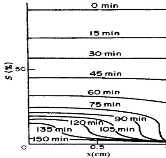
Figure 3.23 Saturations in reference paper
