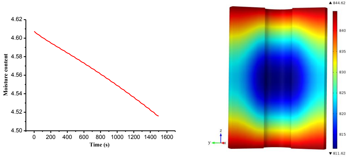
Figure 5.37 Average moisture content (left) and distribution (right) after processing 25 cycles
