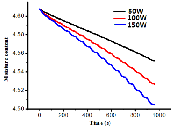
Figure 6.2 Comparison of moisture contents
