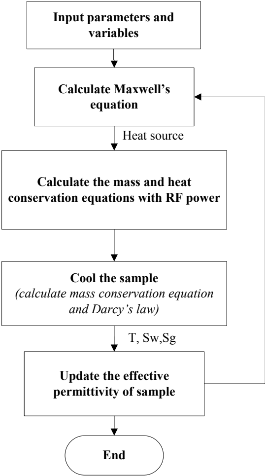
Figure 5.2 Simple flow chart of simulation
