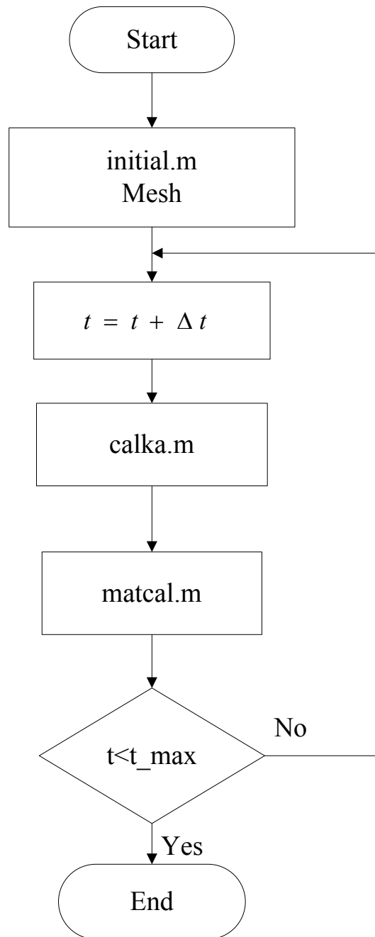
Figure 3.7 Flow chart of calculation
