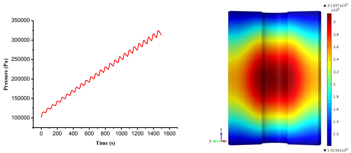
Figure 5.29 Pressure change of point 1(left) and distribution (right) after processing 25 cycles
