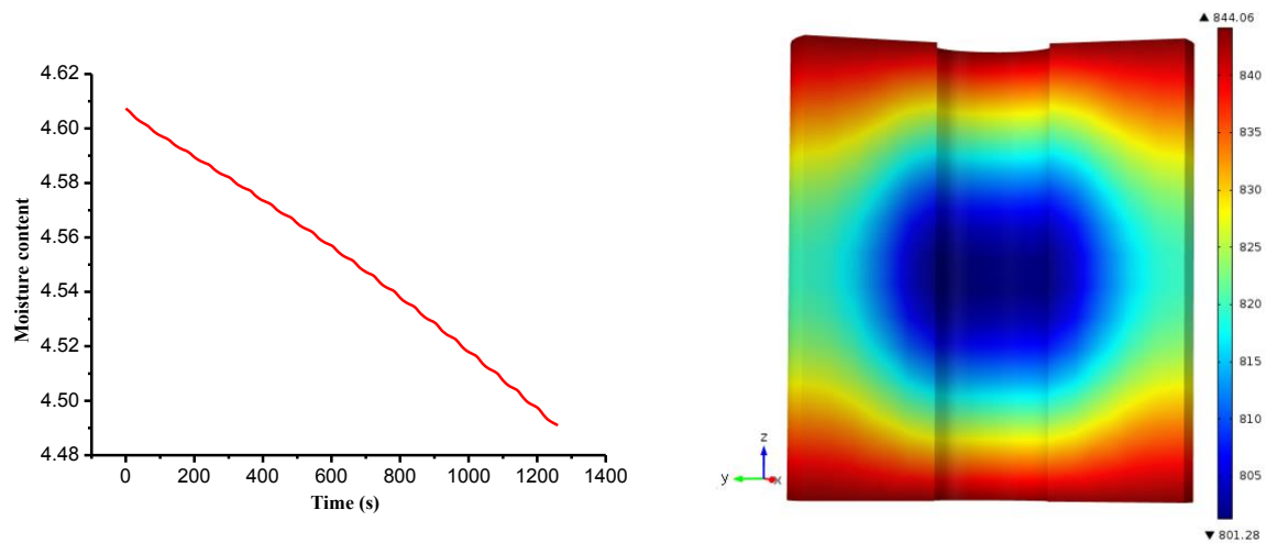
Figure 5.39 Average moisture content (left) and distribution (right) after processing 20 cycles
