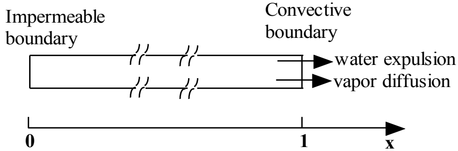
Figure 3.3 Schematic of 1D brick
