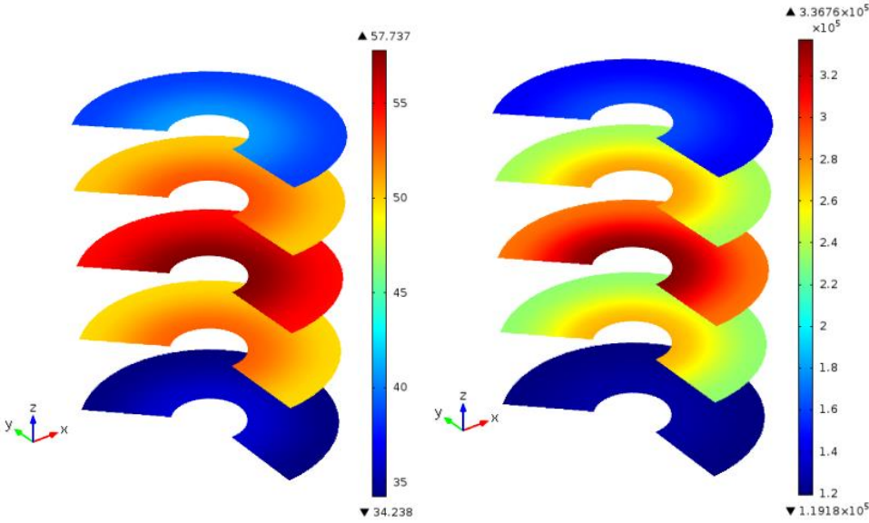
Figure 5.32 Cross-sectional distribution of temperature (left) and pressure (right) after processing 15 cycles
