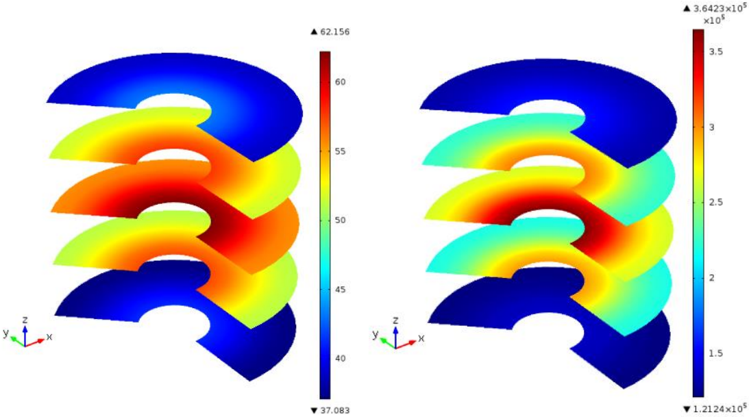
Figure 5.35 Cross-sectional distribution of temperature (left) and pressure (right) after processing 20 cycles
