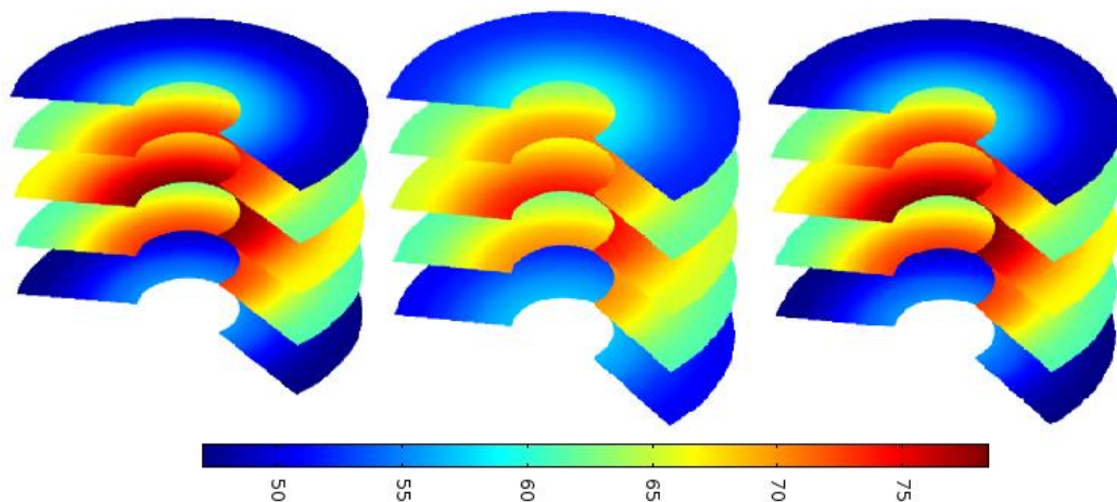
Figure 6.50 Comparison of temperature distributions of different slices of samples heated by different values of positions: 20mm (left), 40mm (middle), 60mm (right)
