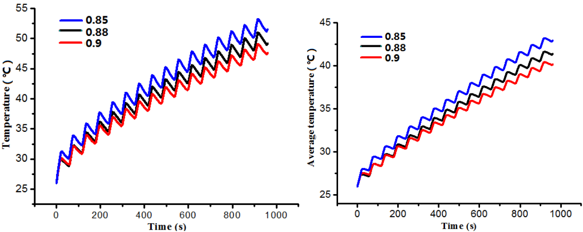
Figure 6.30 Comparison of temperatures of point 1 Figure6.31 Comparison of average temperatures
