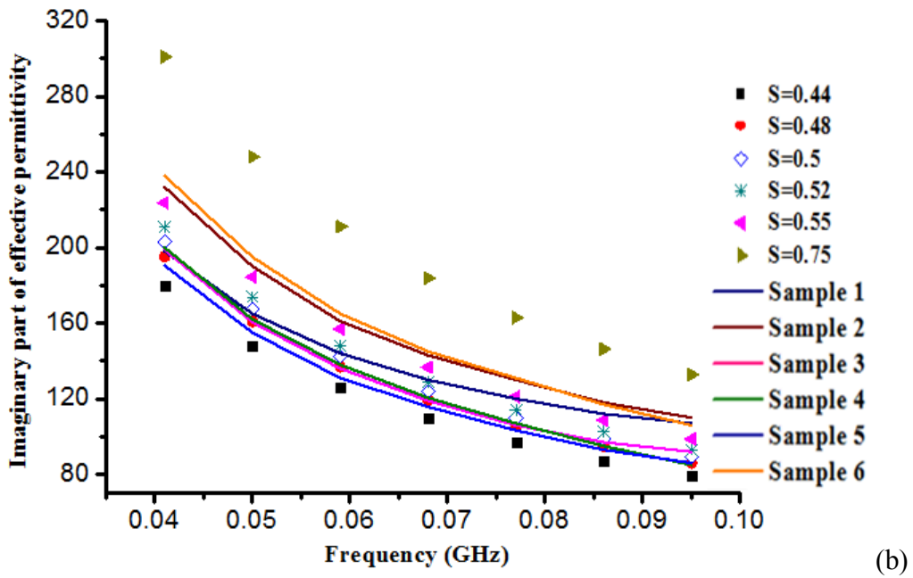
Figure 4.20 Comparison of measured and simulated effective permittivity: (a) real part, (b) imaginary part
