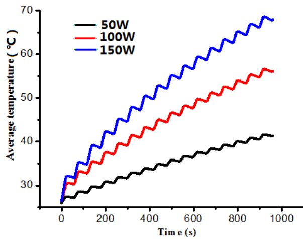
Figure 6.3 Comparison of average temperatures
