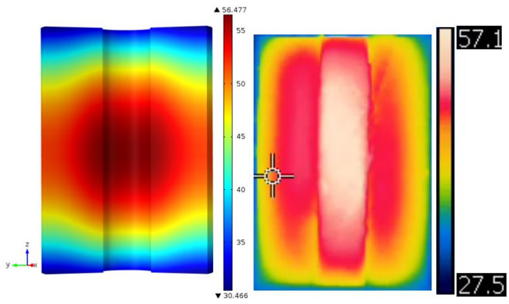
Figure 5.17 Comparison of temperatures of sample after processing 25 cycles (inside)
