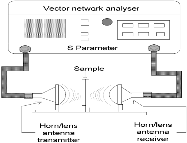
Figure 4.3 Schematic of free space measurement system
