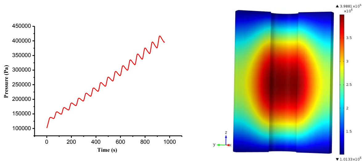
Figure 5.30 Pressure change of point 1(left) and distribution (right) after processing 16 cycles
