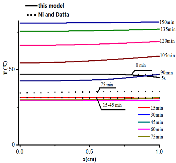
Figure 3.20 Calculated temperatures by Matlab
