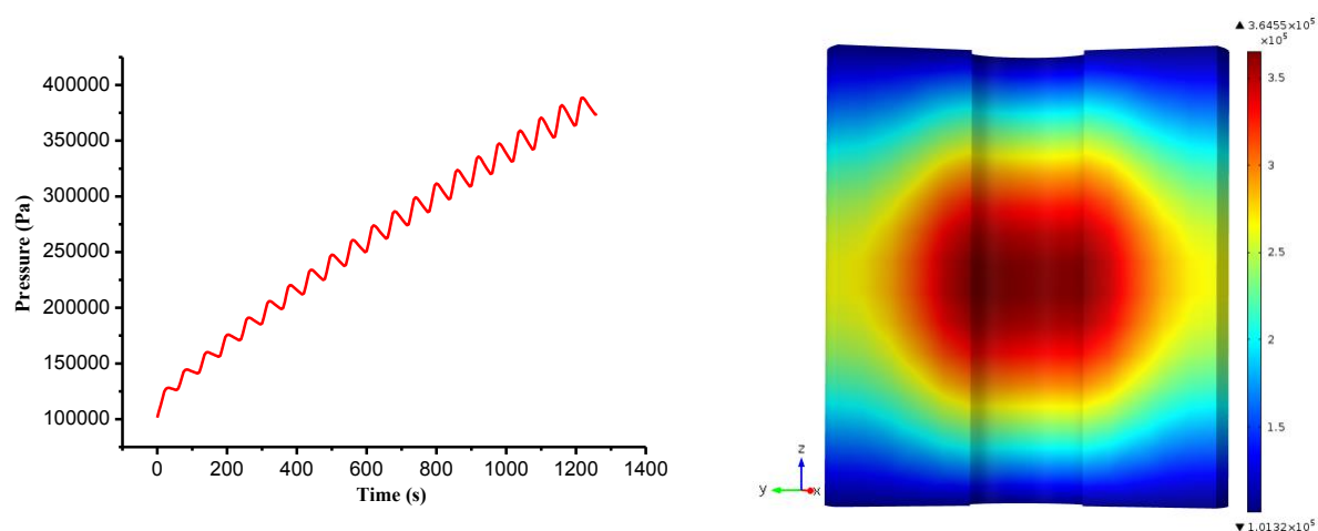
Figure 5.31 Pressure change of point 1(left) and distribution (right) after processing 20 cycles
