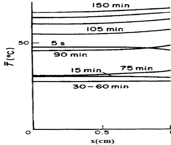
Figure 3.21 Temperatures in reference paper
