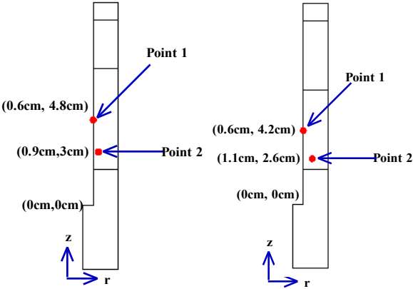
Figure 5.10 Positions of two points for measuring temperature: height of sample is 57mm (left); height of sample is 45mm (right)
