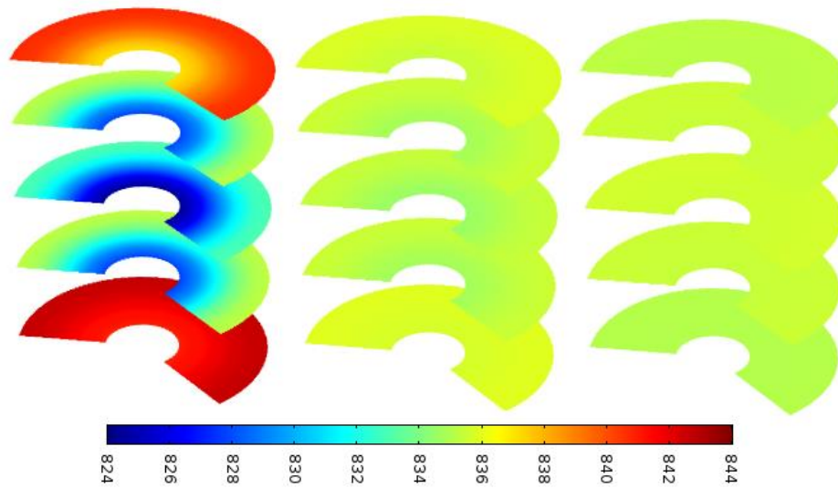
Figure 6.23 Comparison of water concentration distributions of different slices of samples heated by different values of k_{in,w} : 1e-15 (left), 1e-16 (middle), 1e-17 (right).
