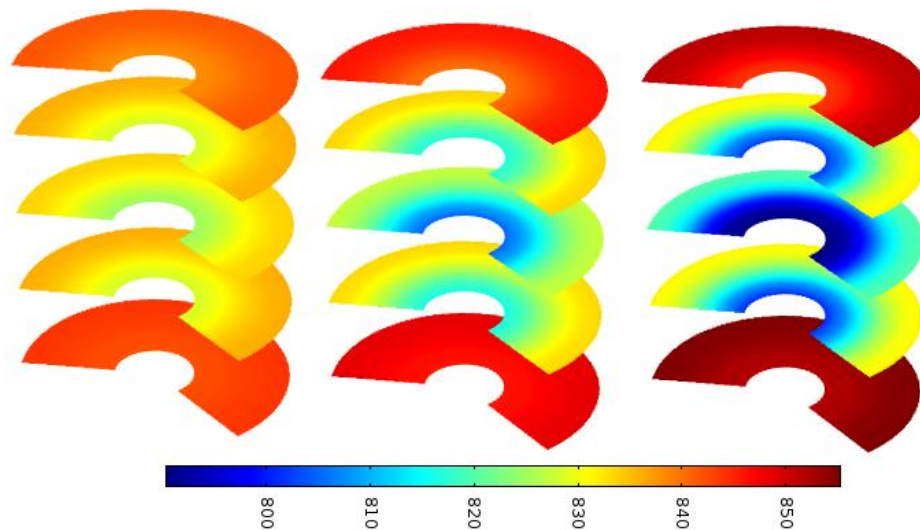
Figure 6.5 Comparison of water concentration distributions of different slices of samples heated by different powers: 50W (left), 100W (middle), 150W (right).
