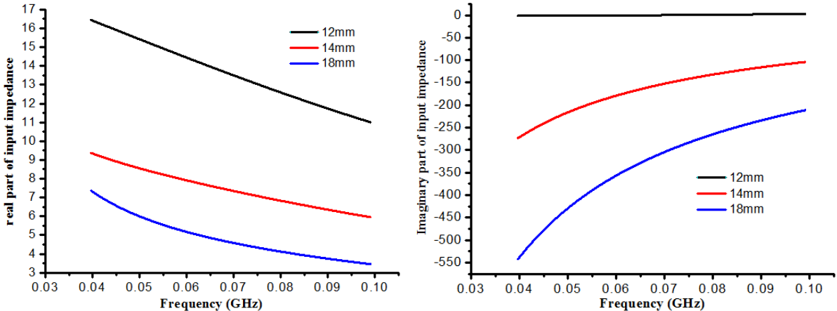
Figure 4.15 Simulated input impedances with different inner diameter of annular samples
