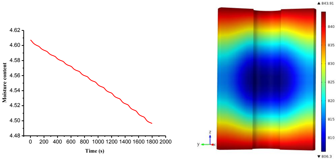
Figure 5.36 Average moisture content (left) and distribution (right) after processing 15 cycles
