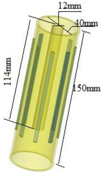
Figure 4.5 Schematic of coaxial cell
