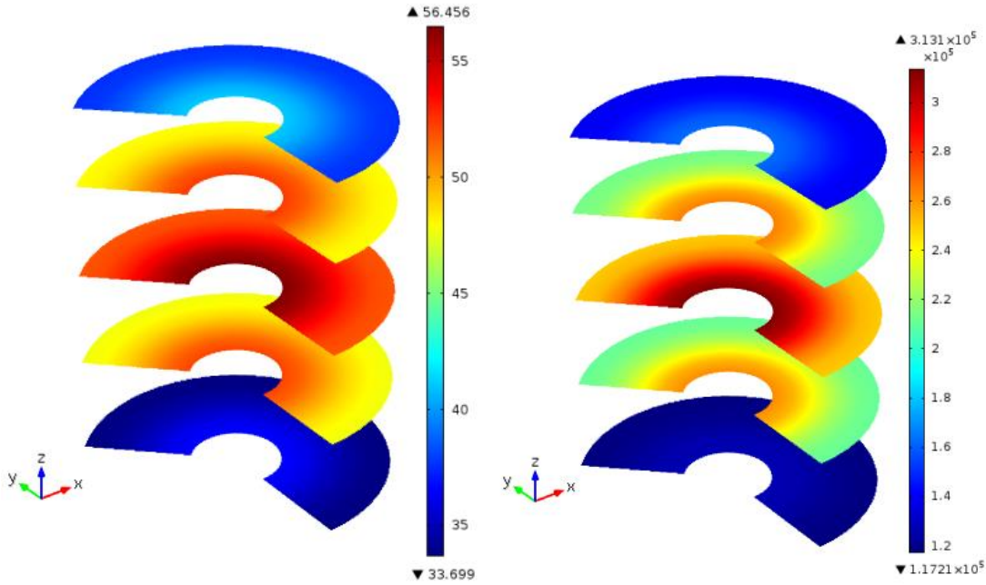
Figure 5.33 Cross-sectional distribution of temperature (left) and pressure (right) after processing 25 cycles
