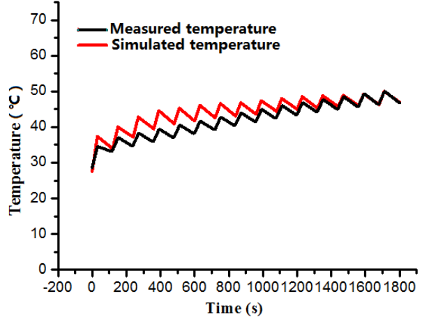
Figure 5.12 Temperature changes of point 2
