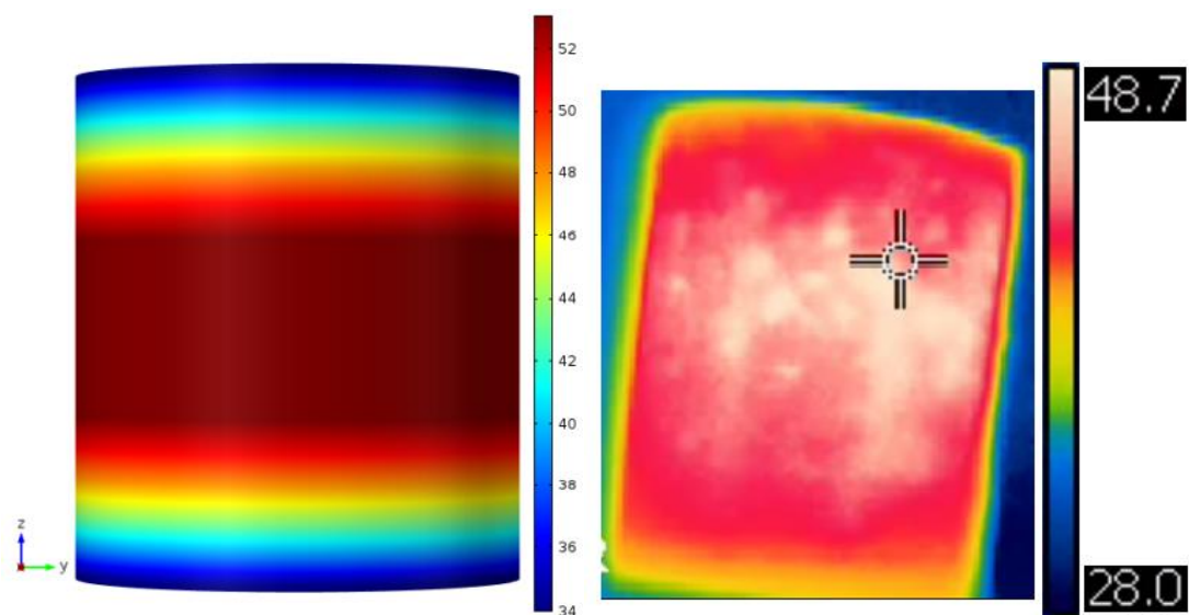
Figure 5.27 Comparison of temperatures of sample after processing 20 cycles (side surface)
