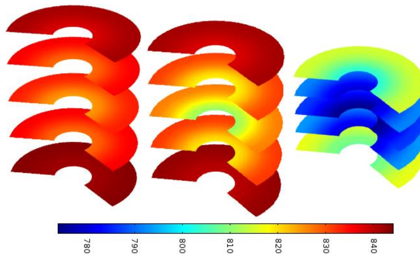
Figure 6.40 Comparison of water concentration distributions of different slices of samples heated by different values of heights: 57mm (left), 45mm (middle), 28.5mm (right).
