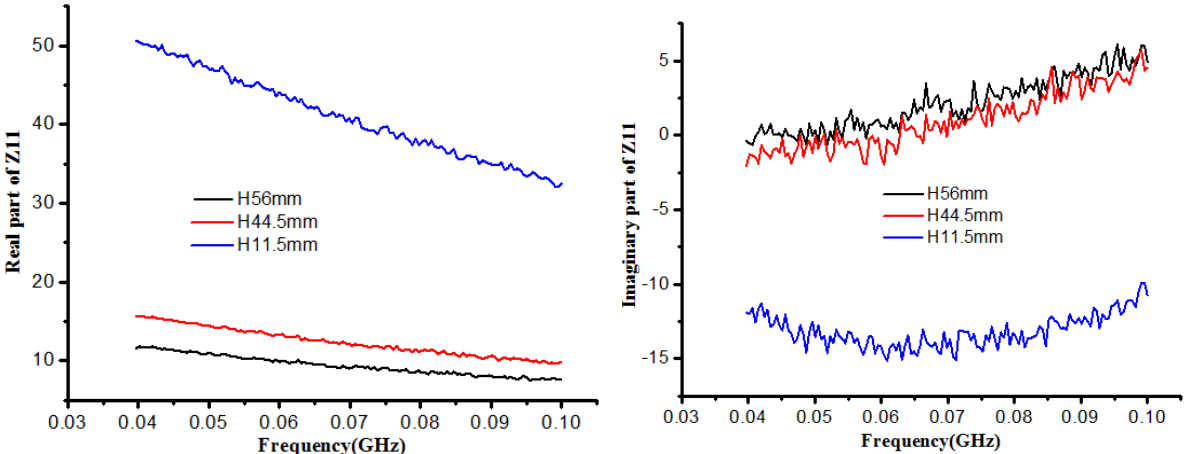
Figure 4.14 Comparison of measured data of potato samples with different height
