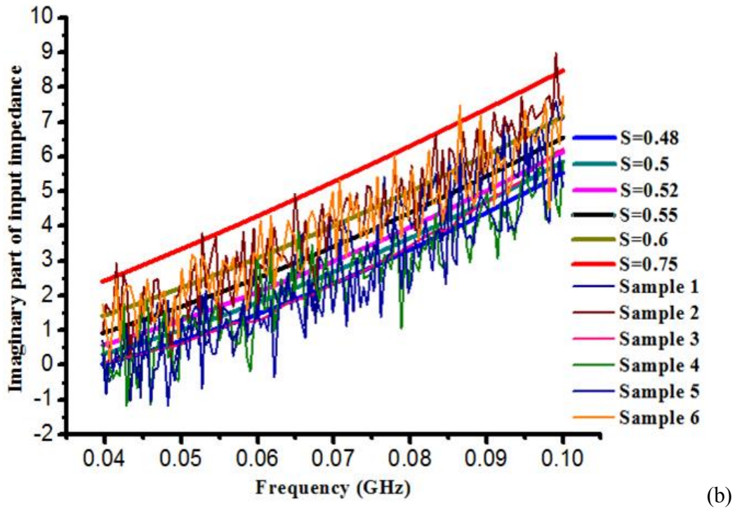
Figure 4.19 Comparison of measured and simulated input impedance: (a) real part, (b) imaginary part
