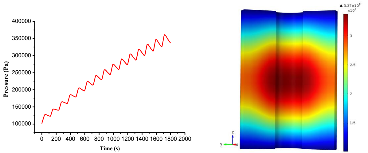
Figure 5.28 Pressure change of point 1(left) and distribution (right) after processing 15 cycles
