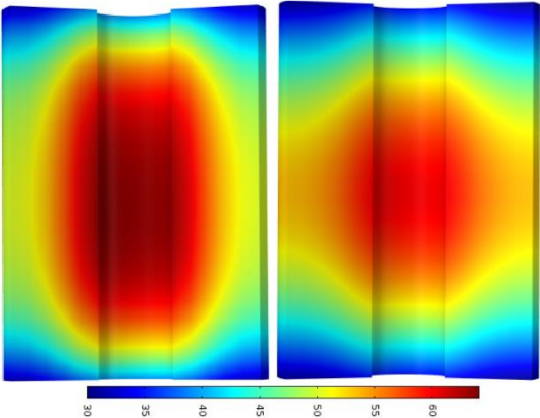
Figure 5.8 Temperature ( ^{\circ}\text{C} ) distributions of inner surface after processing with the same energy: (left) continuous heating; (right) intermittent heating
