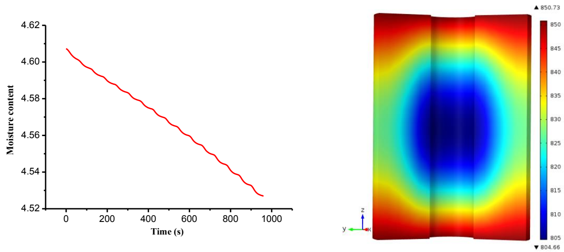
Figure 5.38 Average moisture content (left) and distribution (right) after processing 16 cycles
