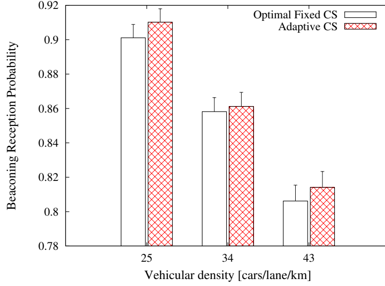
Figure 5.7: Beacons reception probability for the best fixed carrier sense threshold and the proposed adaptive mechanism for three different vehicular densities. The 95% confidence intervals are also shown
