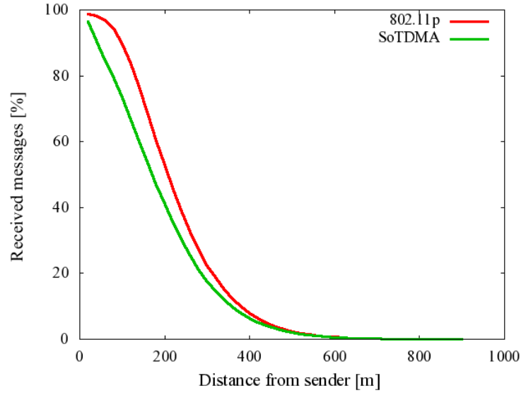
Figure 2.7: Beaconing reception probability at different distances from the sender in a high density scenario
