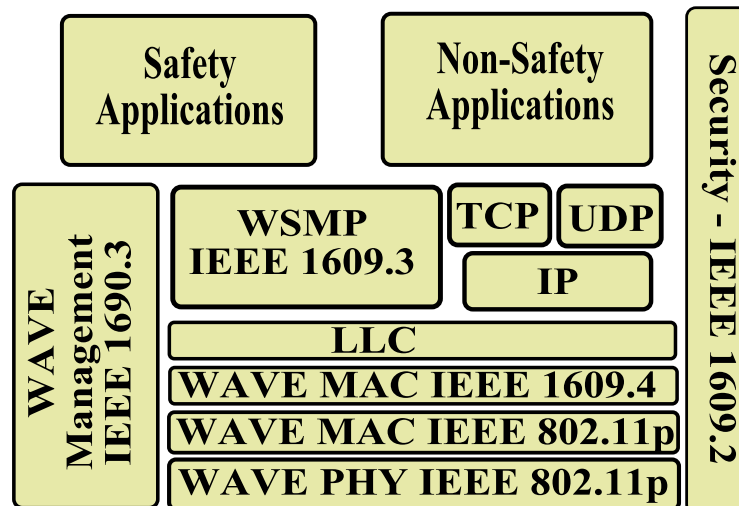
Figure 2.2: IEEE WAVE Architecture
