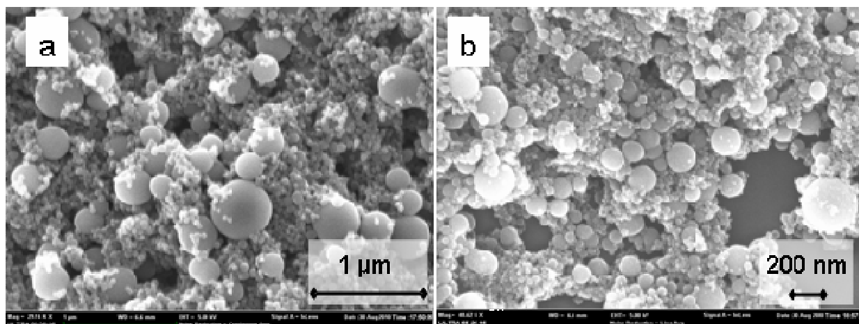
Figure 61. SEM observations of soot samples from the 0.80 mm particles thermal decomposition at 1200°C (a) and 1400°C (b), after 4 s of residence time
