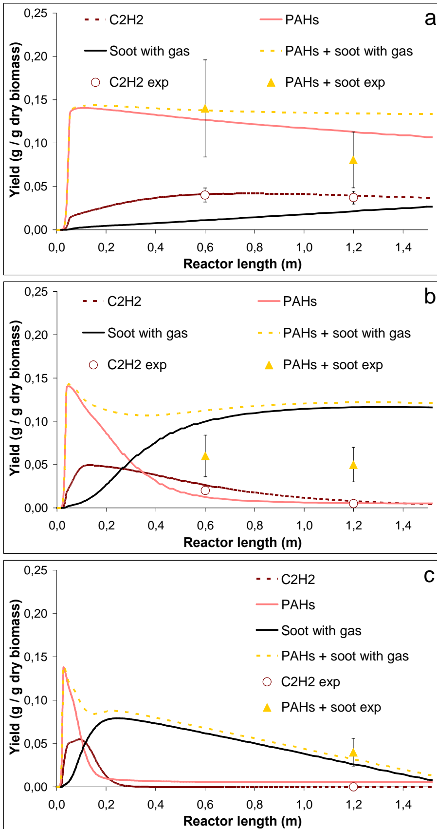
Figure 82. Experimental and simulated (by considering soot gasification) mass yields of \text{C}_2\text{H}_2 , PAHs and soot from the particles thermal decomposition under a wet atmosphere at 1000°C (a), 1200°C (b) and 1400°C (c), versus reactor length
