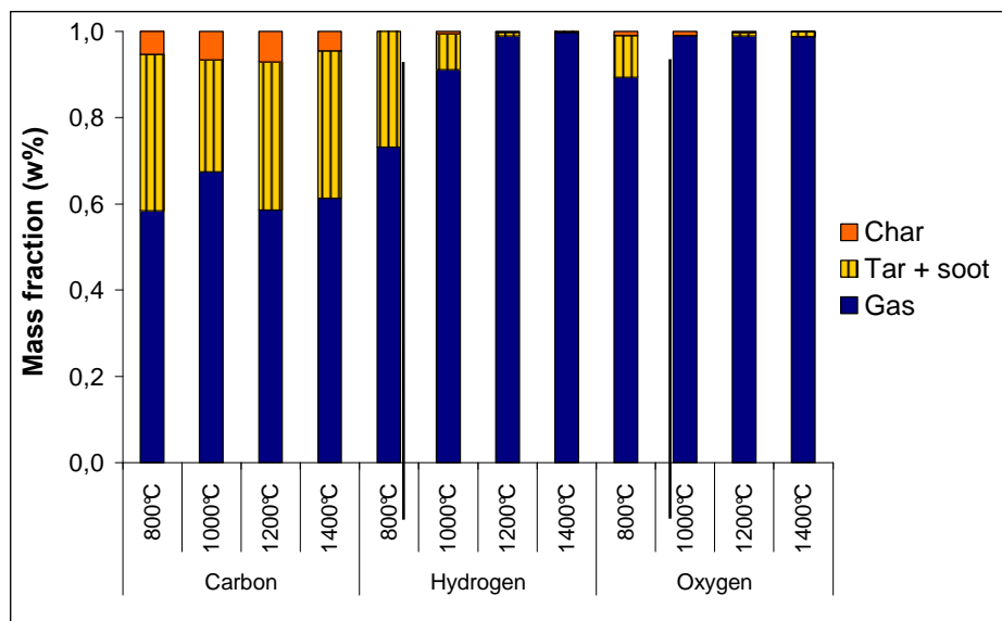
Figure 50. Mass fraction of C, H and O in the products from the 0.35 mm particles thermal decomposition under an inert atmosphere at 800°C, 1000°C, 1200°C and 1400°C
