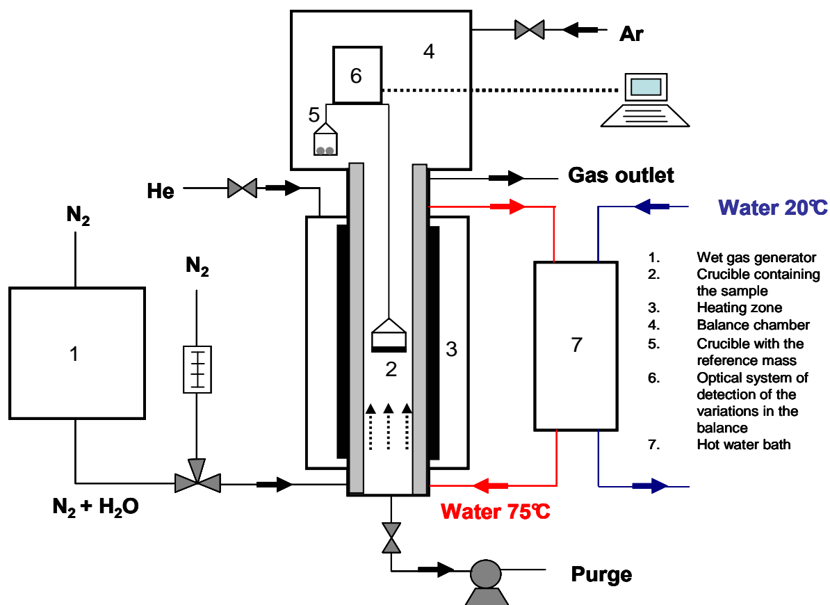
Figure 45. Scheme of the TGA facility
