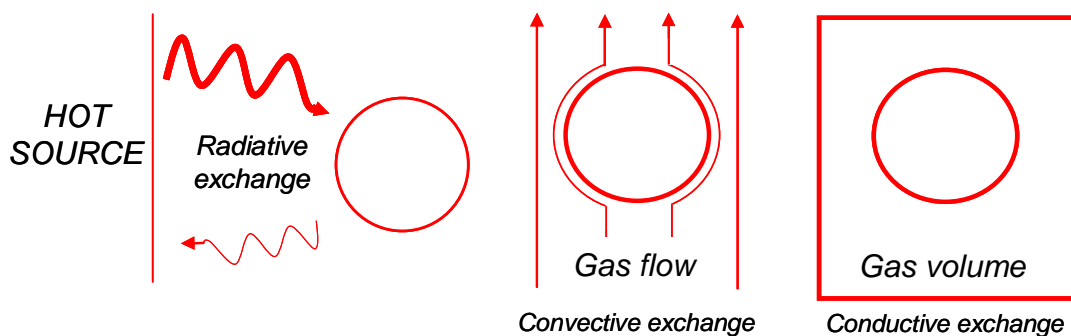
Figure 8. External radiative, convective and convective transfer modes for a wood particle
