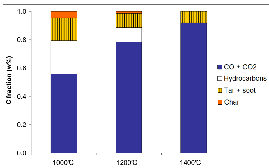
Figure 54. Carbon repartition in the products from the 0.35 mm particles thermal decomposition under a wet atmosphere at 1000°C, 1200°C and 1400°C
