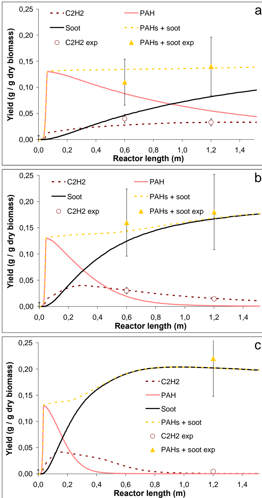
Figure 80. Experimental and simulated mass yields of C_2H_2 , PAHs and soot from the particles thermal decomposition under an inert atmosphere at 1000°C (a), 1200°C (b) and 1400°C (c), versus reactor length
