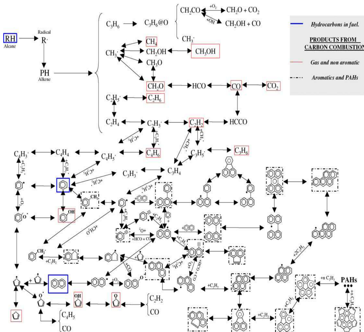
Figure 32. Kinetic scheme of the main reactions used in a model for the combustion of hydrocarbons and PAHs formation (Durán et al., 2004)
