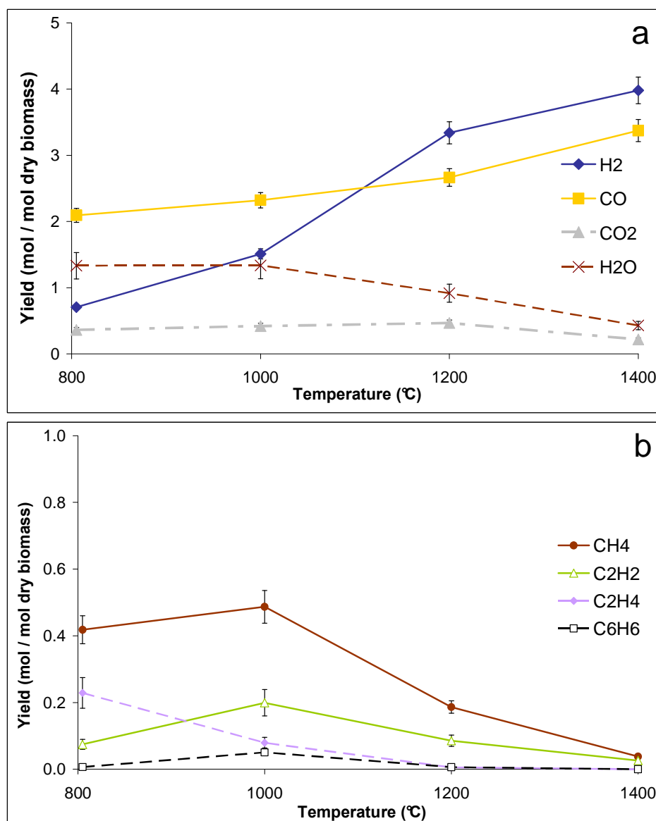
Figure 51. Molar yields of non hydrocarbon gas (a) and light hydrocarbons (b) from the 0.35 mm particles thermal decomposition under an inert atmosphere at 800°C, 1000°C, 1200°C and 1400°C
