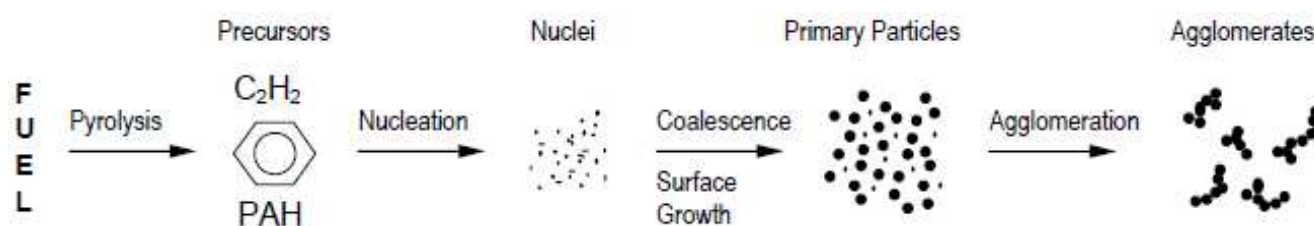
Figure 15. Scheme of soot formation (Svensson, 2005)
