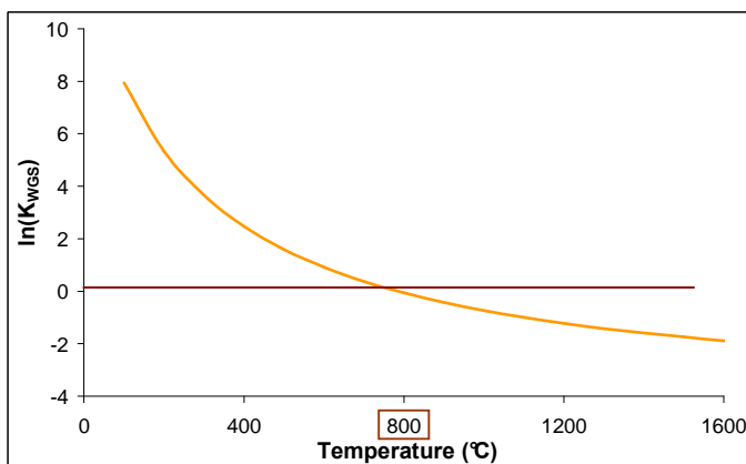
Figure 16. Logarithmic value of water gas shift equilibrium constant versus temperature
