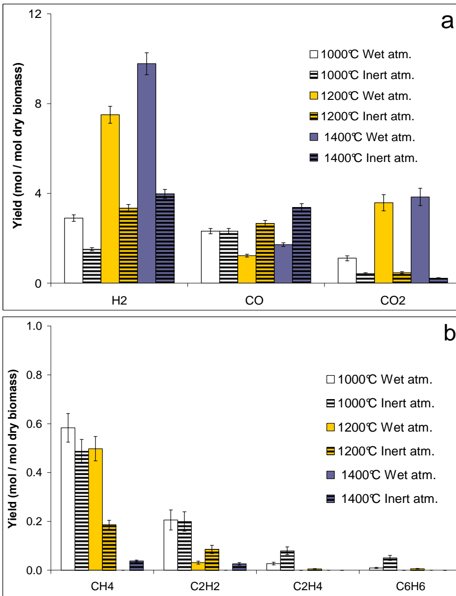
Figure 53. Molar yields of non hydrocarbon gas (a) and light hydrocarbons (b) for the 0.35 mm particles thermal decomposition under inert and wet atmospheres at 1000°C, 1200°C and 1400°C
