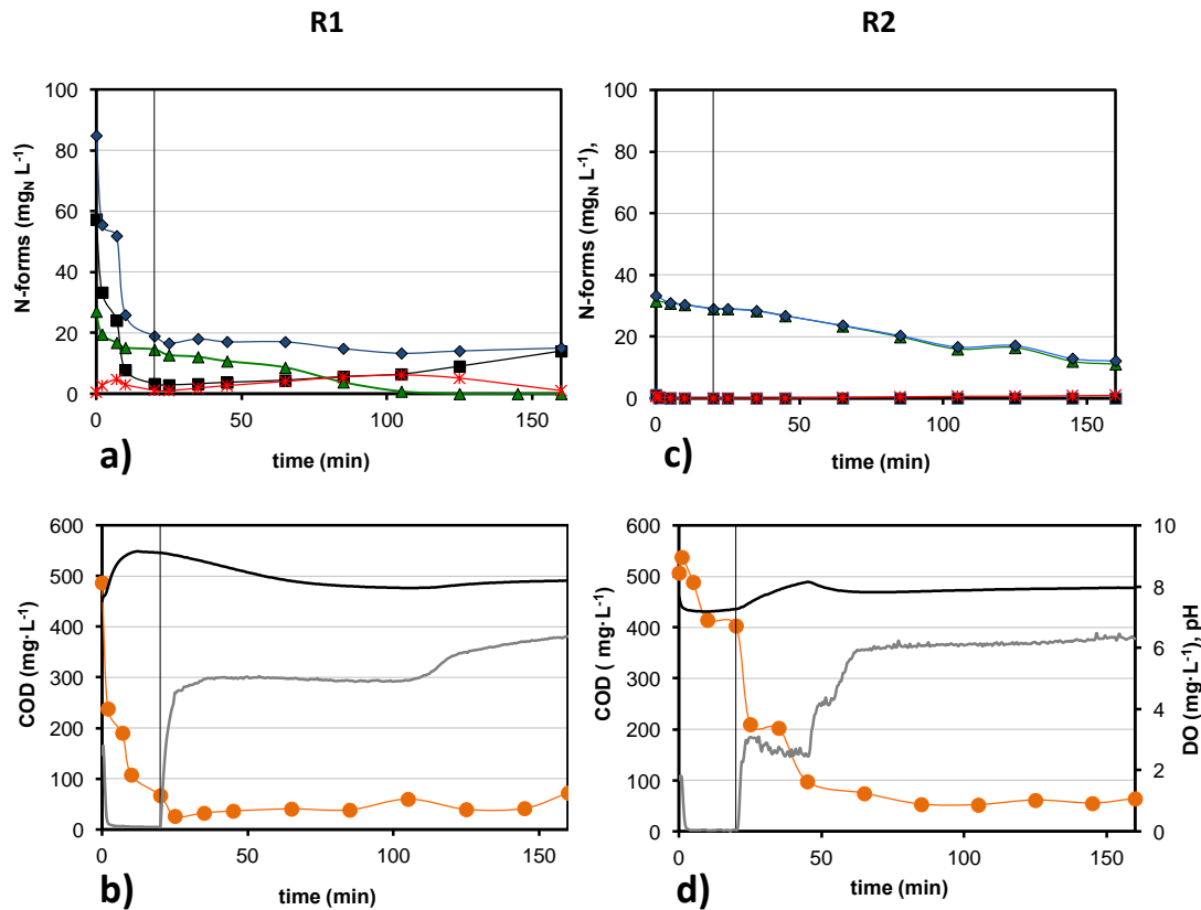
Figure III.7. Evolution of NO_3^- (■), NO_2^- (*), NH_4^+ (▲), COD (●), TN (◆), pH (—) and DO (—) during a kinetics cycle for R1 (a,b) et R2 (c,d) on day 167 th .
