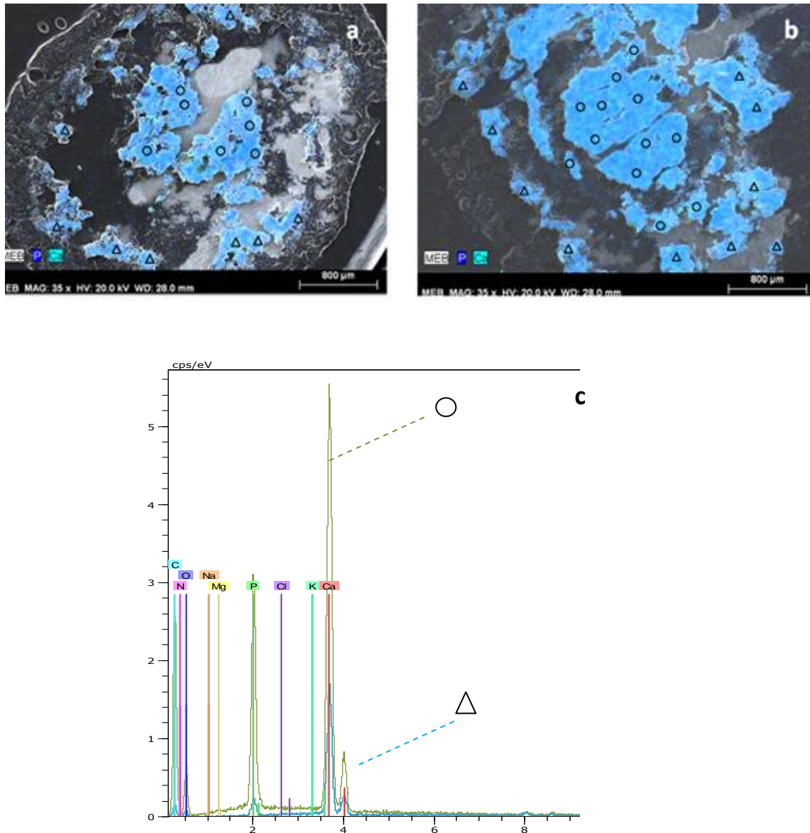
Figure IV.5: EDX analysis of the mineral layers in granules from the GSBRs. a) granule from GSBR_1; b) granule from GSBR_2; c) Inner and outer layer-patterns with EDX analysis from fig.5.a. The different “Δ” and “O” marks represent the probe pointing at the outer and inner parts respectively.
