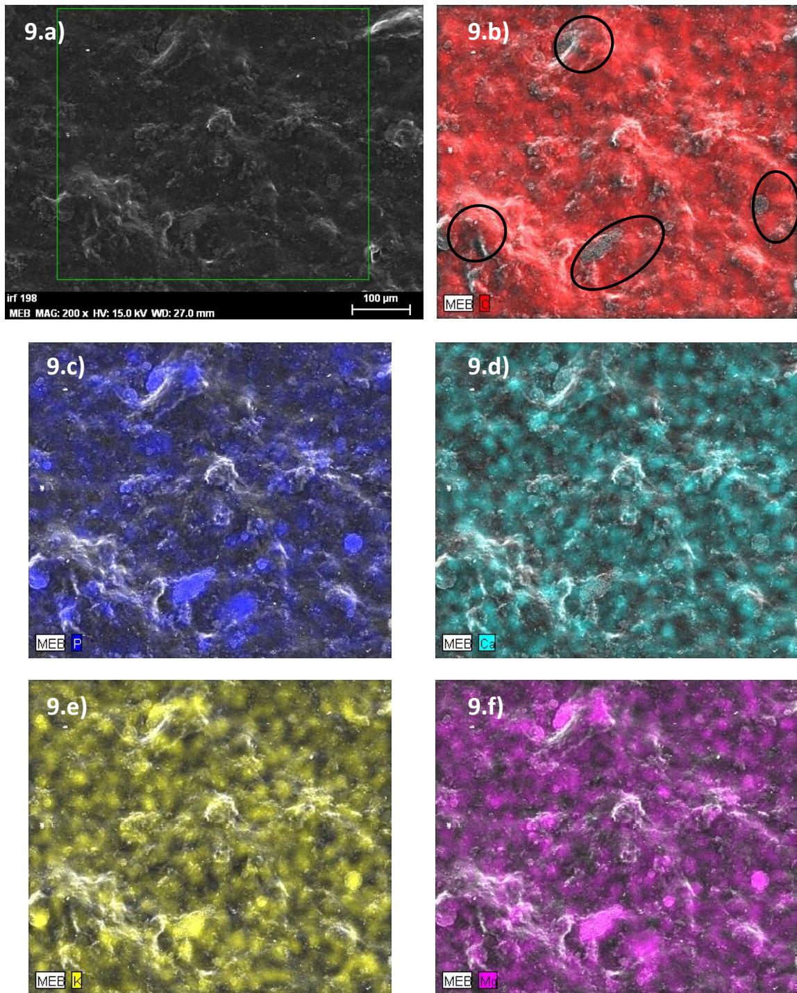
Figure II. 9: a) SEM image of flocs from the GSBR; b) carbon (red) scanning with EDX; c) phosphorus scanning (dark blue) with EDX; d) calcium scanning with EDX probe; e) potassium scanning with EDX; f) magnesium scanning with EDX
