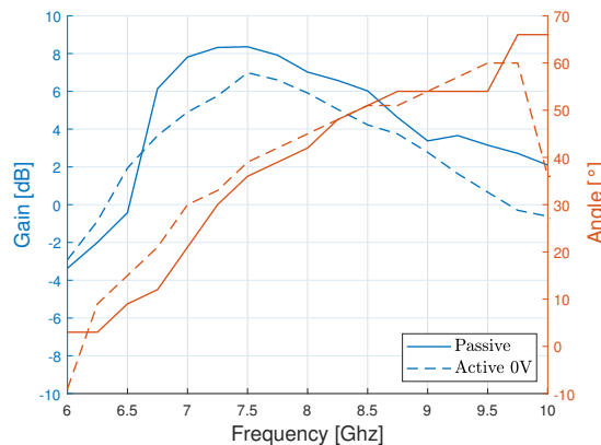
Figure 3.17 – Measure gain and main beam angle
