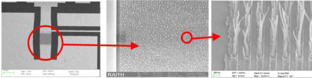
Figure 1.9 – IDC and VACNTs [9]
