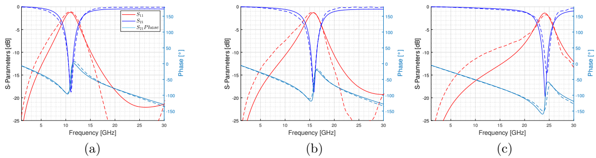
Figure 2.19 – Comparison between full wave simulation (dashed line) and equivalent model (solid line) of the UC, for (a) C = 1.1 pF, (b) C = 0.4 pF and (c) C = 0.14 pF
