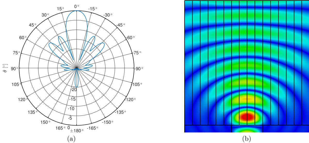
Figure 4.25 – Center law at 25 GHz: (a) Normalized radiation pattern and (b) Electric field
