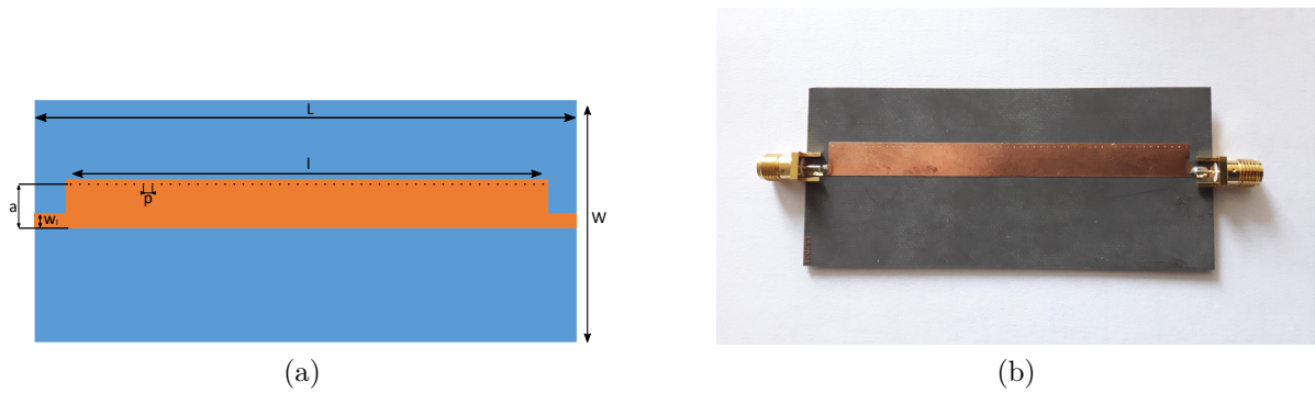
Figure 3.1 – Antenna prototype
