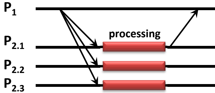
Figure 6.3: Semi-active replication.
