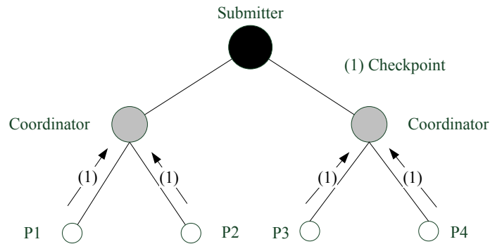
Figure 6.6: Uncoordinated checkpointing process for asynchronous iterative schemes.
