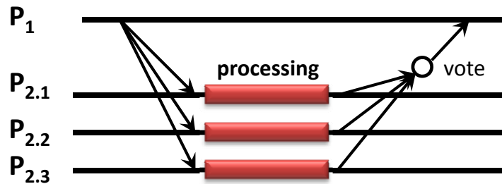
Figure 6.2: Active replication.
