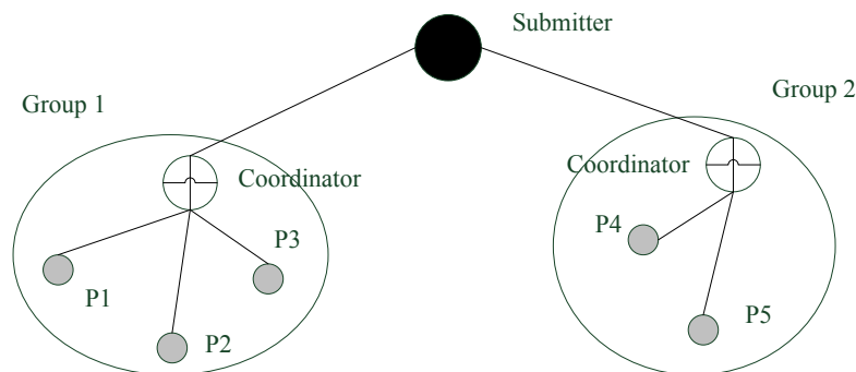
Figure 5.5: Allocation graph.
