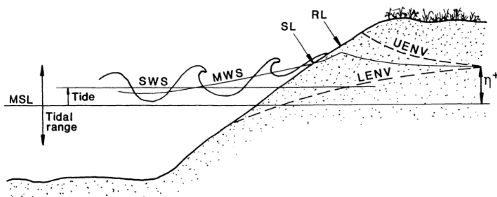
Fig. 2.1: Schematic of the forcing at a coastal boundary (Nielsen, 1999).
