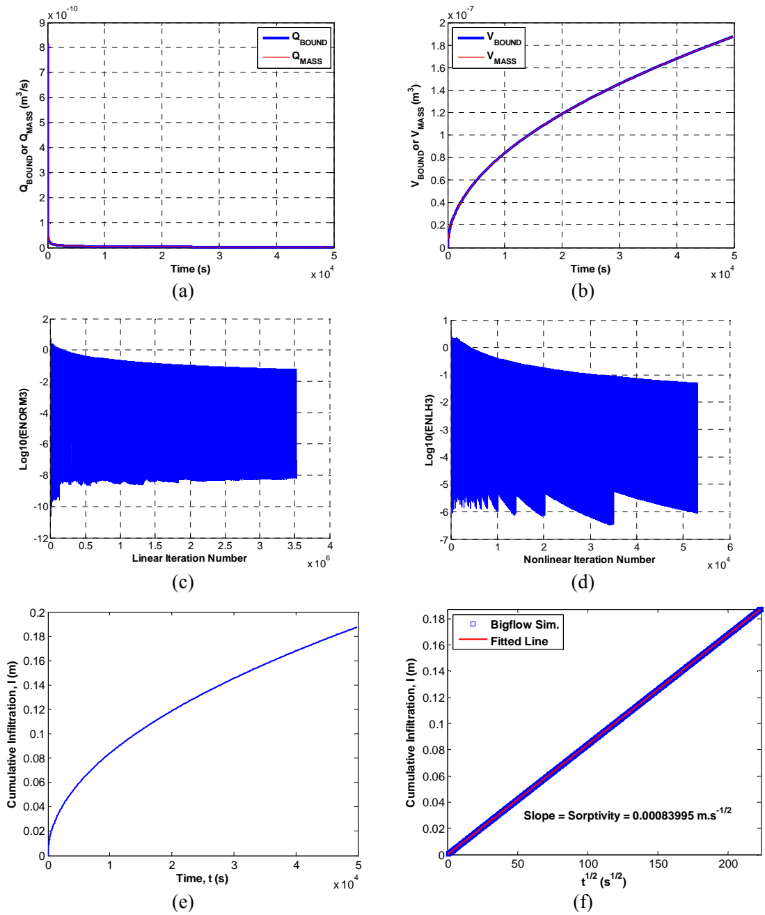
Fig. 4.8: BIGFLOW simulation results for horizontal infiltration case into Guelph loam (PM3): (a) Local mass balance: evolution of Q_{BOUND} and Q_{MASS} . (b) Global volume balance: evolution of V_{BOUND} and V_{MASS} . (c) Linear iteration convergence. (d) Nonlinear iteration convergence. (e) Evolution of the cumulative infiltration. (f) Sorptivity determination by fitting a linear regression line to I versus \sqrt{t} data points.
