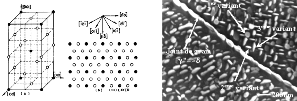
Figure II. 1 : Unit cell of DO_{22} structure ( \gamma'' - Ni_3Nb ) structure and arrangement of atoms in the (111) plane (a) [Sundararaman et al.,1994], various variants of \gamma'' phases detected in Inconel 718 microstructure (b) [Alexandre,2004].
