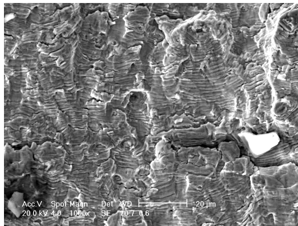
Figure IV. 20 : Scanning electron micrographs of fracture surfaces after LCF tests at 550°C using a triangular signal at 1Hz.
