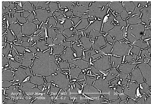
Figure III. 3 : Microstructure of Inconel 718 after conventional heat treatment [Taina et al.,2010].
