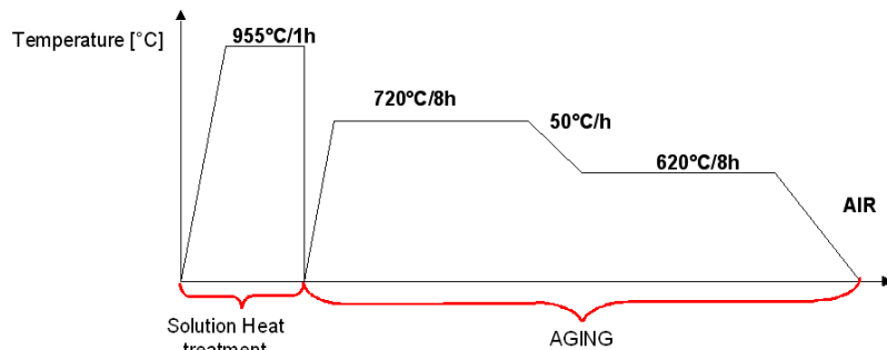
Figure III. 2 : Standard thermal treatment for Inconel 718 following ASTM B637 specification.
