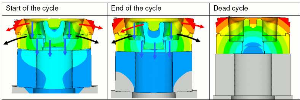
Figure I. 5 : Deformation behaviour during Extrusion cycle. [Dossin,2010]
