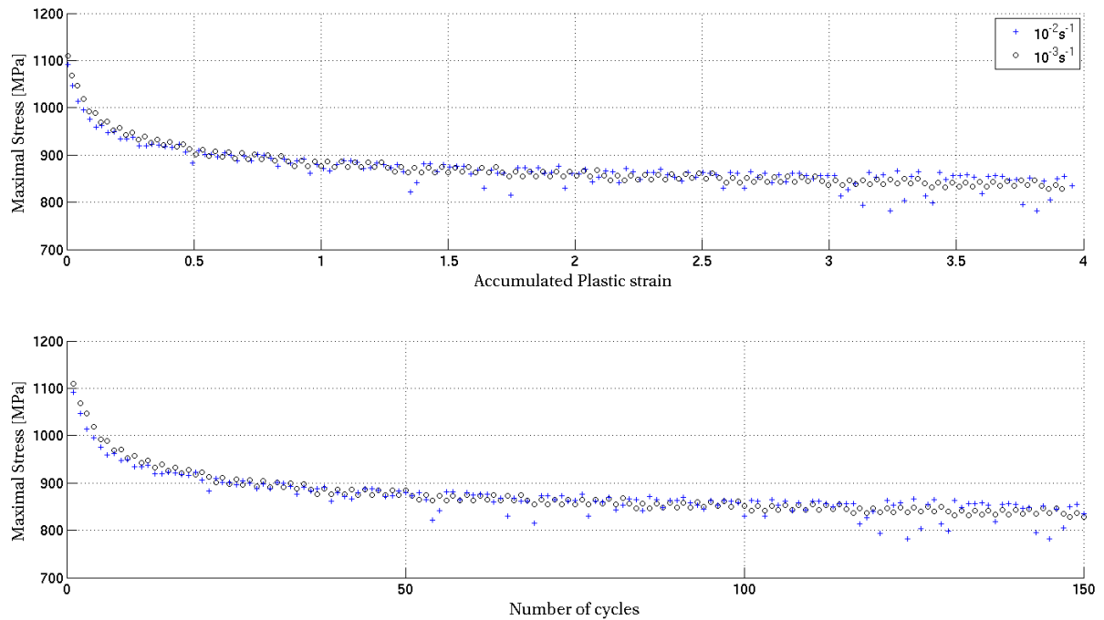
Figure IV. 3 : Strain controlled fatigue tests with a total strain amplitude of \pm 1.2\% ( T=550^\circ\text{C} ).
