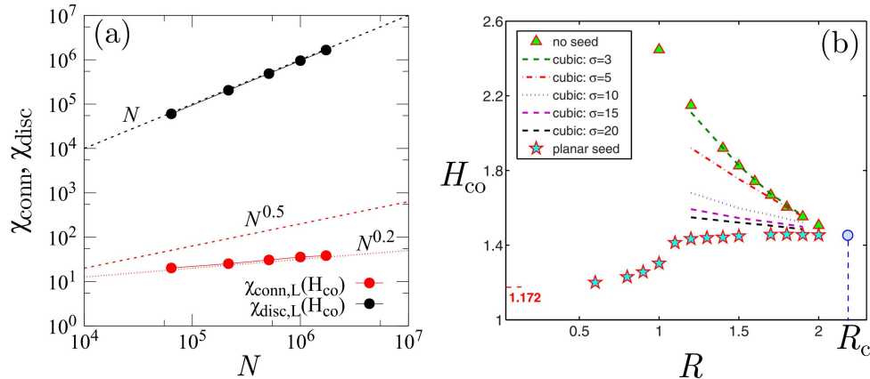
Figure I.13: Results from computer simulations of the 3D AQS driven random-field Ising model in the R < R_c regime. (a) Scaling of the peak (at H = H_{\text{co}} ) of the connected and disconnected susceptibility with the system size, for R = 1.8 . The disconnected one follows the expected scaling \chi_{\text{disc,L}} \sim N , while the connected one increases much slower than the expected \sqrt{N} . (b) Value of the coercive field for a 3D RFIM with R < R_c where a seed of up-spins has been inserted at the beginning of the dynamics. Such seed would be present in the thermodynamic limit, but is absent in finite-size simulations. Dashed lines are for a cubic seed of linear size \sigma . Stars are for a planar seed, which seems to give the correct limit as R \rightarrow 0 . Adapted from [133].
