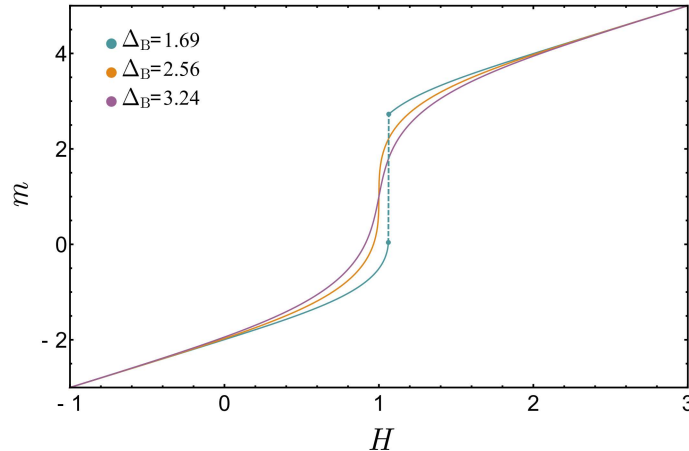
Figure 3.2: Quasi-statically driven mean-field RFIM (described by Eq. (3.22)) at zero temperature: average magnetization m = \bar{m} versus applied field H for the ascending branch of the hysteresis loop and for different values of the disorder strength \Delta_B . For these curves, k = 2 and J = 1 .
