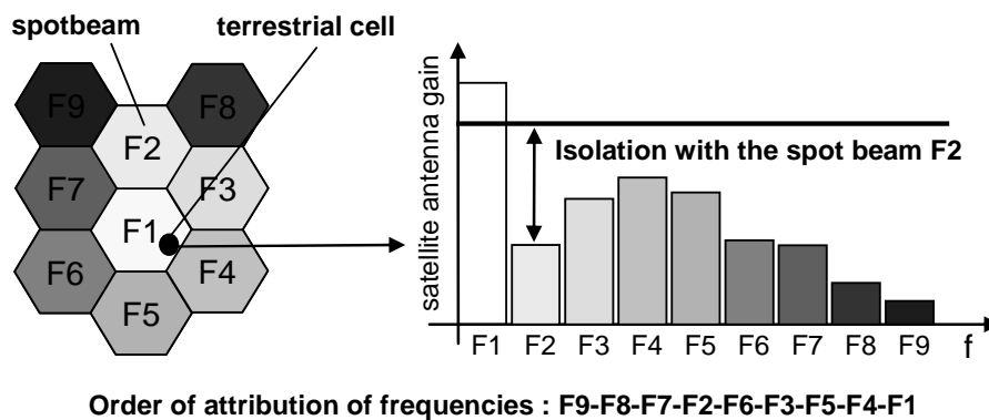
Figure 4-1 : Principe d'allocation "Position Aware"
