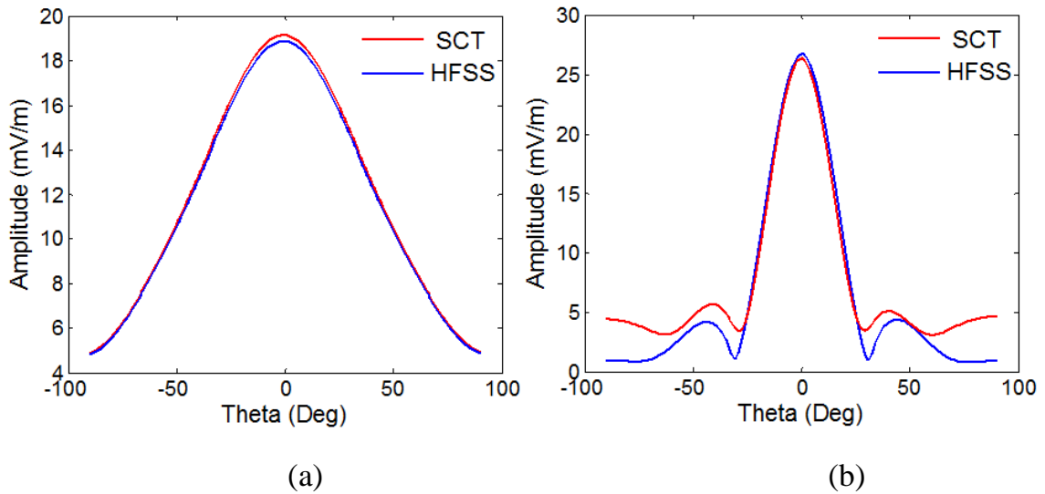
Figure 6.25: Radiation patterns of 4×1 uniform reflectarray of Figure 18 keeping the electronic configuration (i.e., the switching states (ON/OFF) for the twelve RF-MEMS switches of four phase shifter cells) of the four phase shifter cells identical and hence obtaining both E and H plane patterns symmetrical (a) E- plane pattern (b) H-plane pattern
