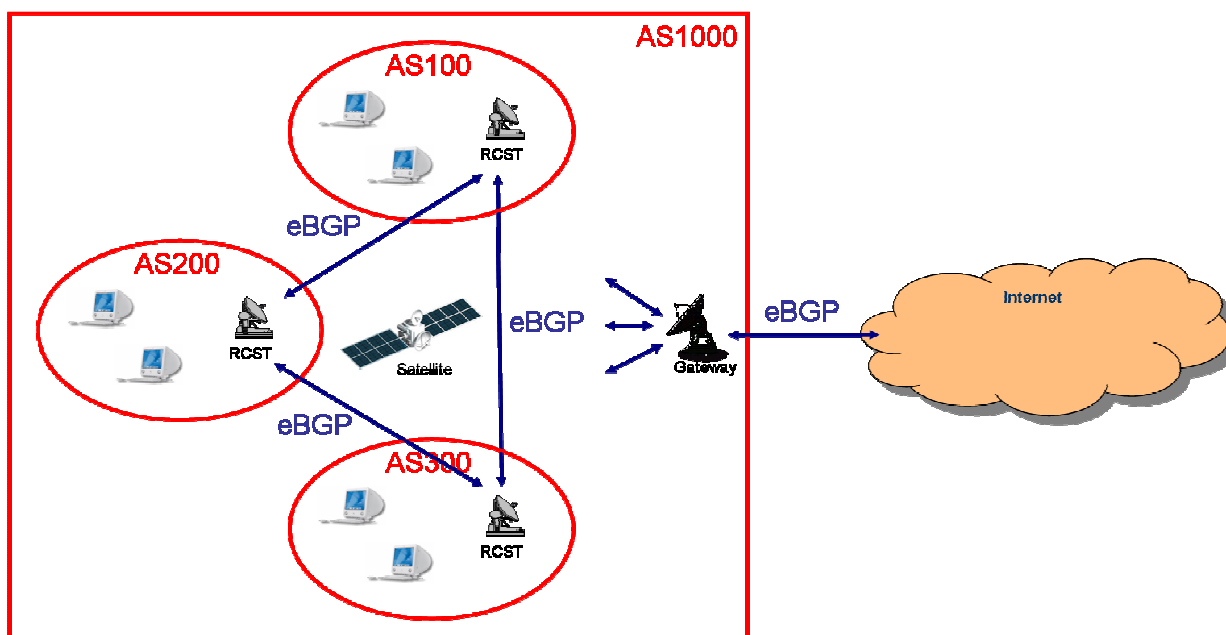
Figure 4-8: BGP confederations
