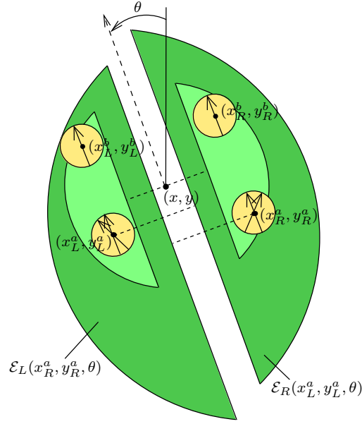
Fig. 6.9: There always exists a sequence of feasible steps from ((x_L^a, y_L^a, \theta_L^a), (x_R^a, y_R^a, \theta_R^a)) to ((x_L^b, y_L^b, \theta), (x_R^b, y_R^b, \theta)) .
