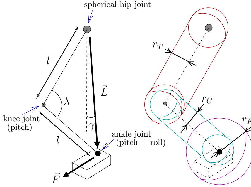
Fig. 4.8: A simple 6-DOF robot leg.
