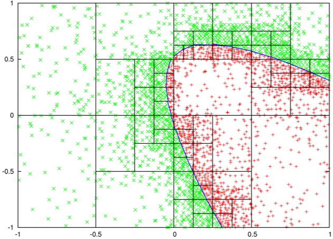
Fig. 3.4: An example run of our approximation algorithm on a continuous function from \mathbb{R}^2 to \mathbb{R} .
