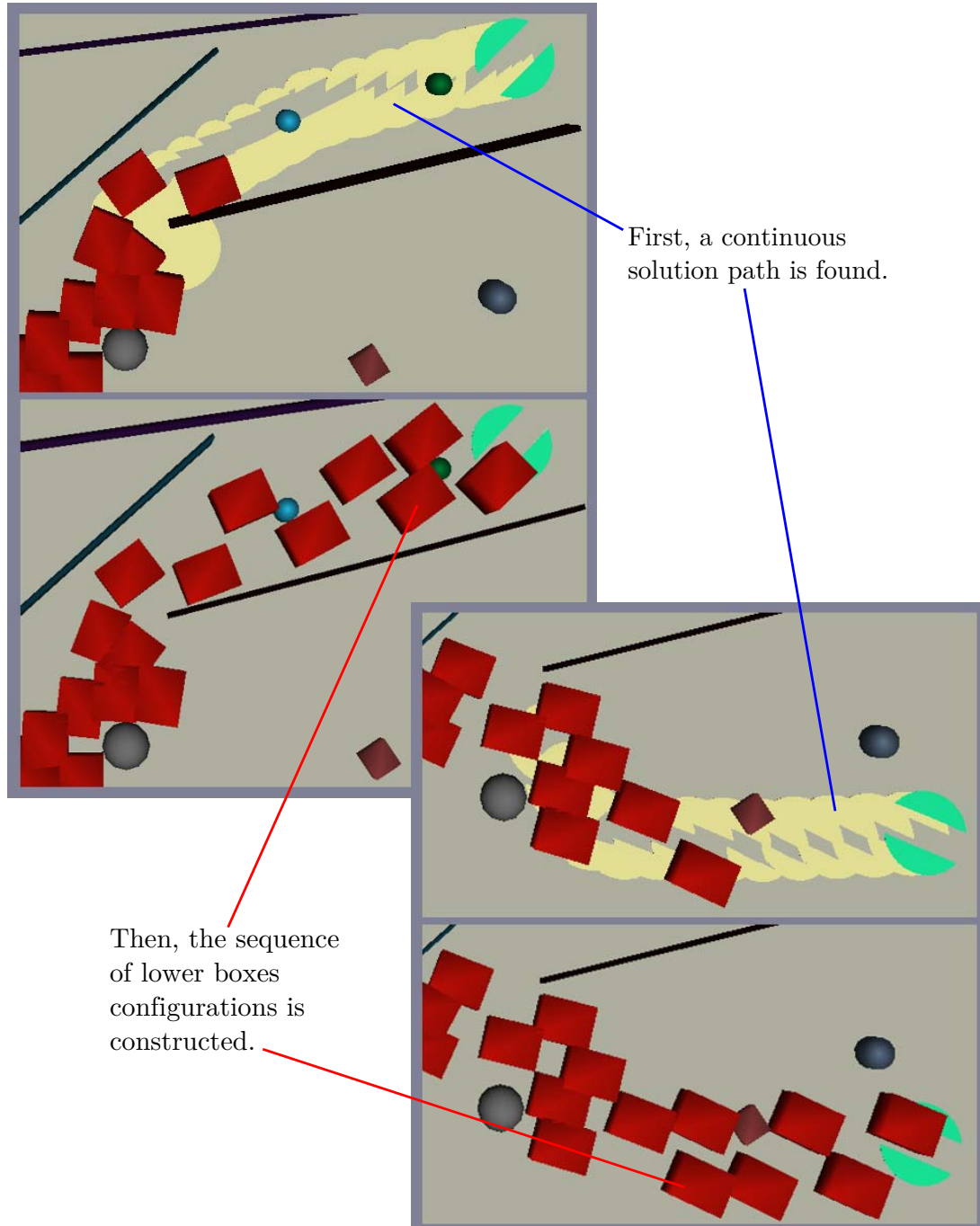
Fig. 6.16: Phases 1) and 2) of the algorithm: two examples. The initial walking trajectory (before smoothing) is such that below height h_m no point outside the lower boxes is touched by the robot (see Fig. 6.14).
