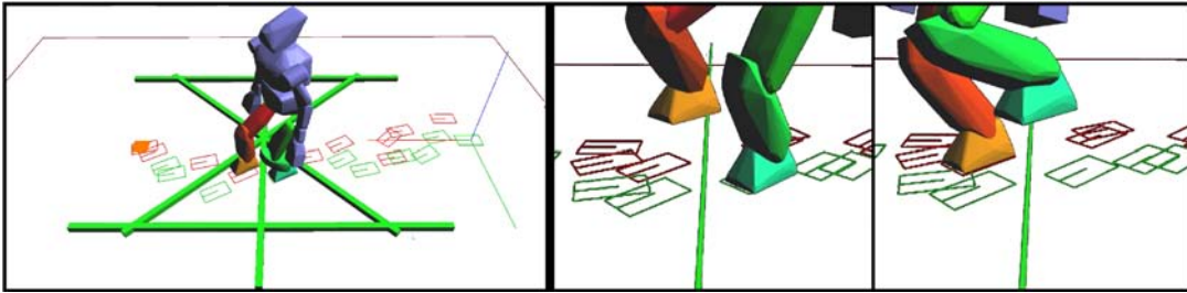
Fig. 5.8: On the left: in simulation, HRP-2 stepping over bars of section 8\text{cm} \times 8\text{cm} . On the right: HRP-2 stepping over an horizontal cable 10\text{cm} above the ground.
