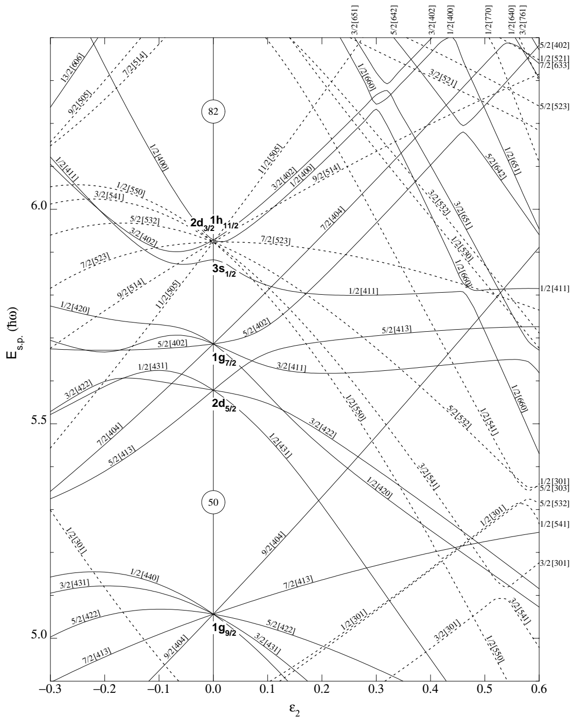
Figure 2.5: Nilsson diagram for neutrons in the 50 \leq N \leq 80 region showing the single-particle energies as a function of the deformation parameter \epsilon_2 . The \epsilon_2 > 0 , \epsilon_2 = 0 , and \epsilon_2 < 0 correspond to the prolate shape, the spherical shape and the prolate shape, respectively.
