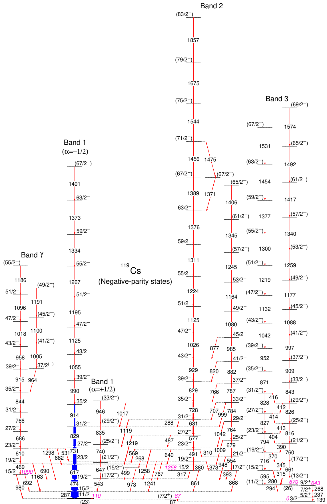
Figure 5.1: Partial level scheme of ^{119}\text{Cs} showing the negative-parity bands. The new transitions are indicated in red. The isomeric levels are indicated with thick line. Energies of levels with some relevance are shown in pink italicized figures.
