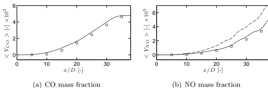
Figure 8.10: Sandia flame D: Axial profiles along the centerline of a) mean CO mass fraction for ARC_22s (—) and b) NO mass fraction for ARC_22_GRI211 (—) and ARC_22_GRI30 (---). Experimental data \circ .
