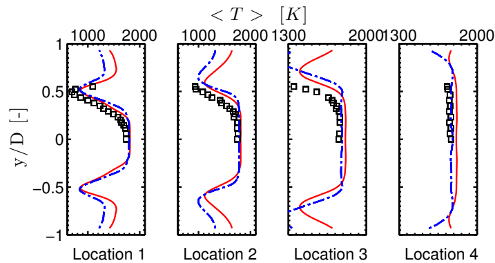
Figure 9.51: SGT-100/Case A: transverse profiles of mean temperature at the four measurement locations. Comparison between adiabatic walls case (baseline), isothermal walls case (· - ·) and experiments ( \square ).
