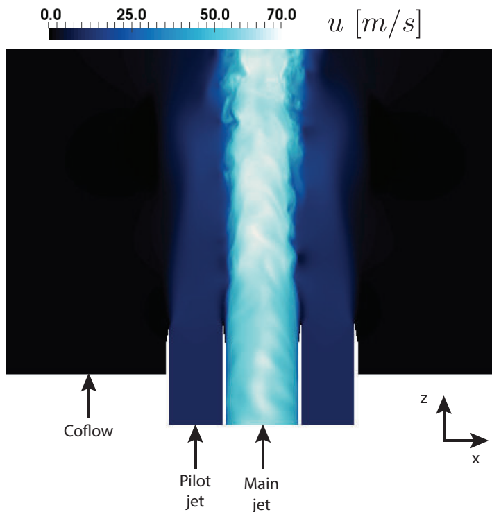
Figure 8.1: View of the three coaxial jets of the Sandia flame D configuration with instantaneous LES axial velocity field.
