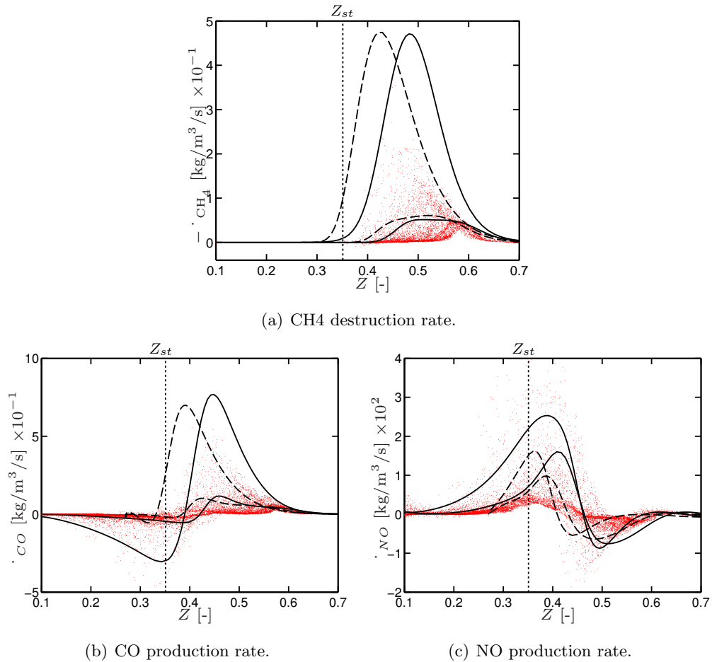
Figure 8.18: Sandia flame D: Scatter plot of \text{CH}_4 , CO and NO source terms vs mixture fraction at axial location z = 30D . Comparison of coflow (—) and pilot (---) counterflow flames at strain rates a = 35 \text{ s}^{-1} and 270 \text{ s}^{-1} .
