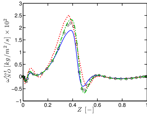
(c) NO source term ( a = 40 \ 80 \ 160 \text{ s}^{-1} ).
