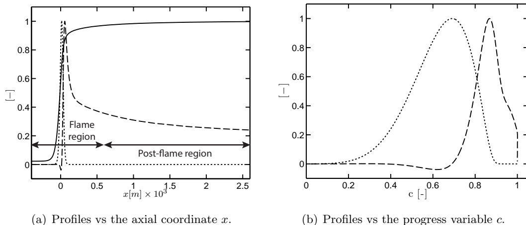
Figure 5.1: One-dimensional methane-air premixed flame at \phi = 1.0 ( T = 680 K and P = 3 bars - SGT-100 conditions). Profiles of progress variable (—) (for a only), NO source term (--) and \text{CH}_4 consumption term ( \cdots ) vs a) axial coordinate and b) progress variable. Quantities are normalised by their maximum value.
