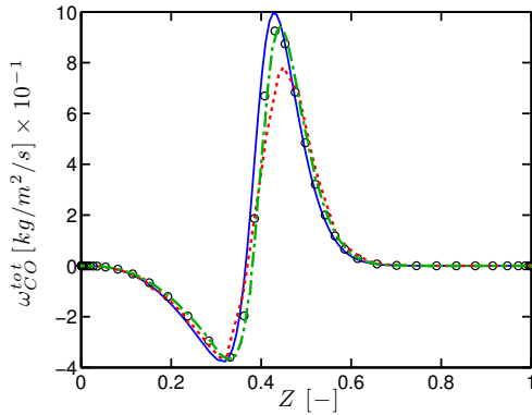
(b) CO source term.
