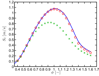
(a) Laminar flame speed.
