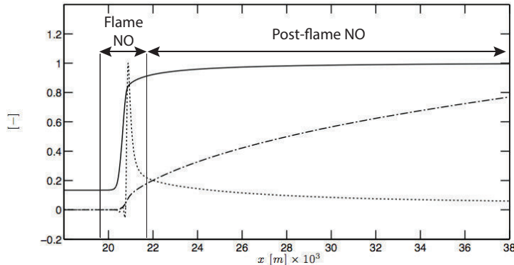
Figure 1.3: One-dimensional premixed methane-air flame at atmospheric conditions and equivalence ratio \phi = 1.15 with GRI 2.11. Normalised temperature (—), NO mass fraction ( \cdot - \cdot - ) and NO source term ( \cdot \cdot \cdot ).
