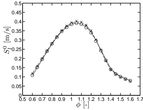
(a) Laminar flame speed.
