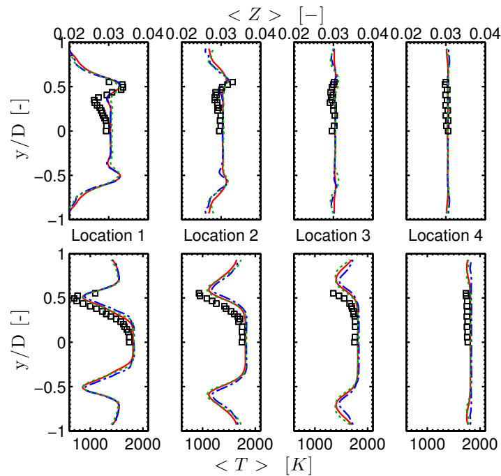
Figure 9.46: SGT-100/Case A: Transverse profiles of mean mixture fraction (top) and temperature (bottom). Comparison between LES with n_{\mathcal{F}} = 5 (—), LES with n_{\mathcal{F}} = 2.5 (---), LES with n_{\mathcal{F}} = 10 (···) and experiments ( \square ).
