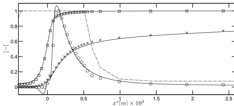
Figure 5.7: Comparison of the NOMAGT model with detailed chemistry on a one-dimensional methane-air premixed flame at \phi = 0.6 : normalised profiles of thickening factor (---), progress variable c^* ( \square ), NO mass fraction from NOMAGT ( \times ) and NO source term from NOMAGT ( \circ ). The continuous lines corresponds to the results obtained for the detailed mechanism with Cantera.
