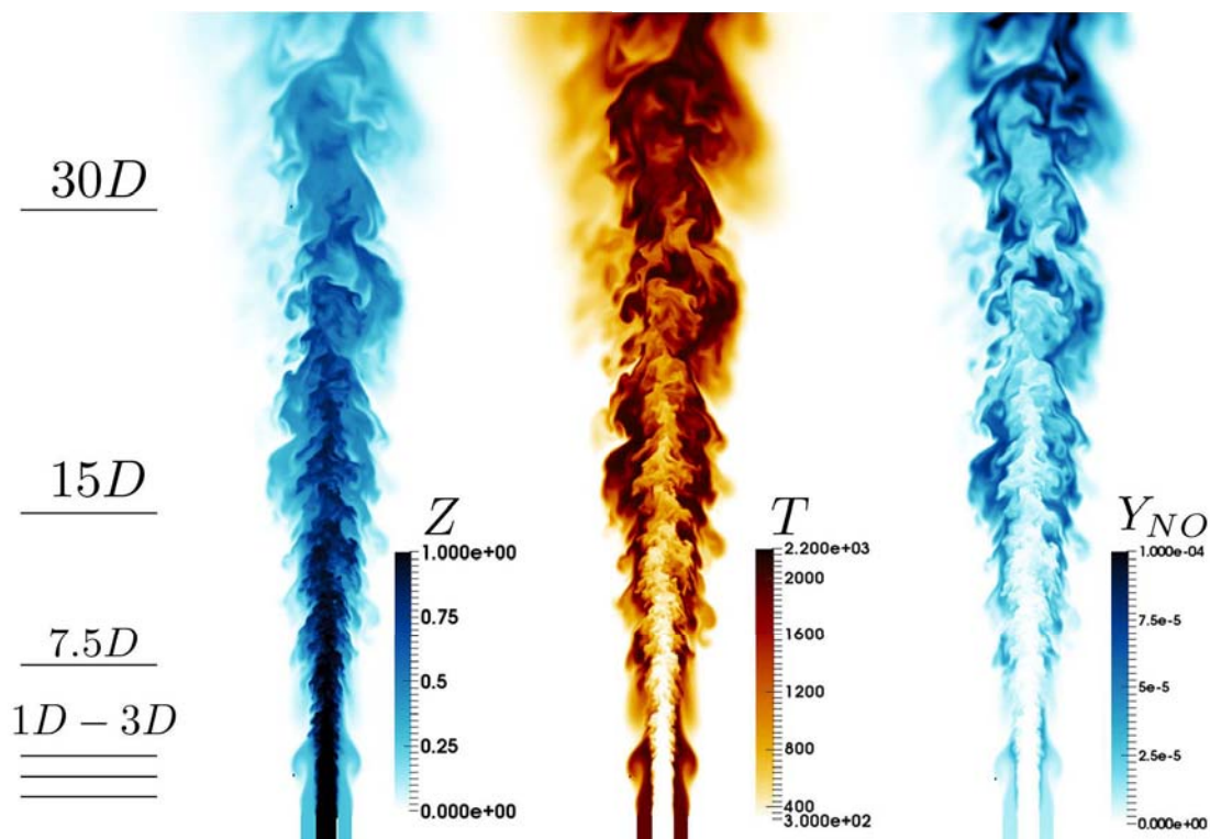
Figure 8.2: Sandia flame D: Instantaneous fields in the mid-plane of mixture fraction (left), temperature (middle) and NO mass fraction (right) for ARC_22_GRI211. The measurement axial locations are indicated on the left side.
