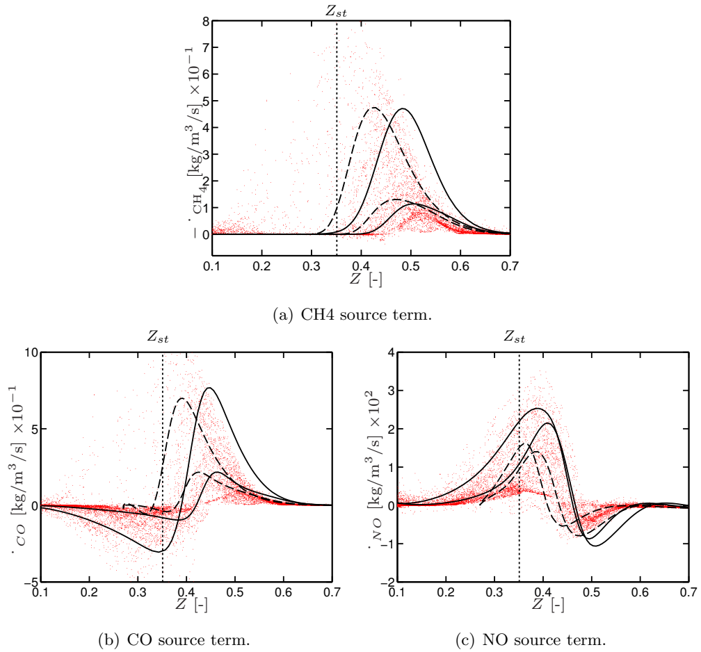
Figure 8.16: Sandia flame D: Scatter plot of CH 4 , CO and NO source terms vs mixture fraction at axial location z = 7.5D . Comparison of coflow (—) and pilot (---) counterflow flames at strain rates a = 60\text{ s}^{-1} and 270\text{ s}^{-1} .
