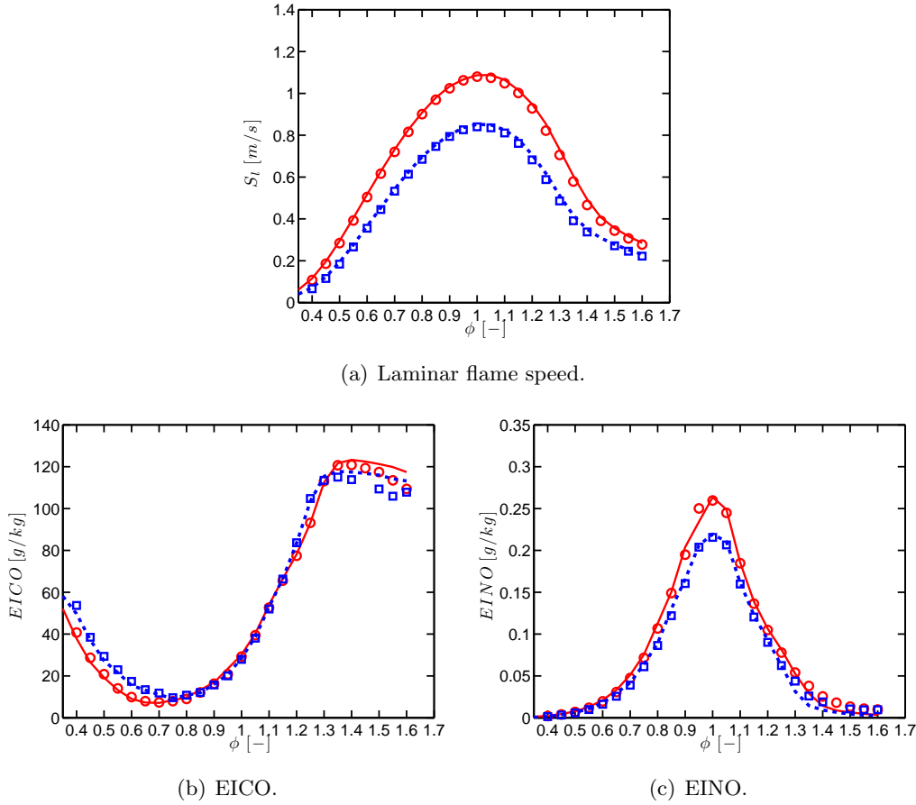
Figure 9.34: One-dimensional unstrained premixed laminar flames in SGT-100 conditions. Comparison between Case A: GRI 2.11 (—), ARC_22_GRI211 (○) and Case B: GRI 2.11 (---), ARC_22_GRI211 (□) of a) laminar flame speed, b) EICO and c) EINO.
