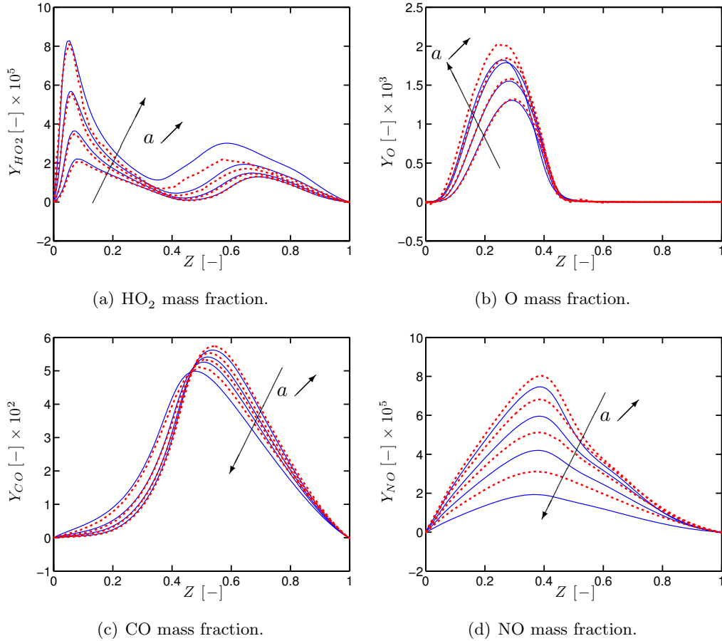
Figure 7.18: Counterflow computations in Sandia flame D conditions at global strain rates a = 40, 80, 160, 320 s^{-1} . Comparison of species mass fractions from Cantera (—) and AVBP (···) in Z -space.
