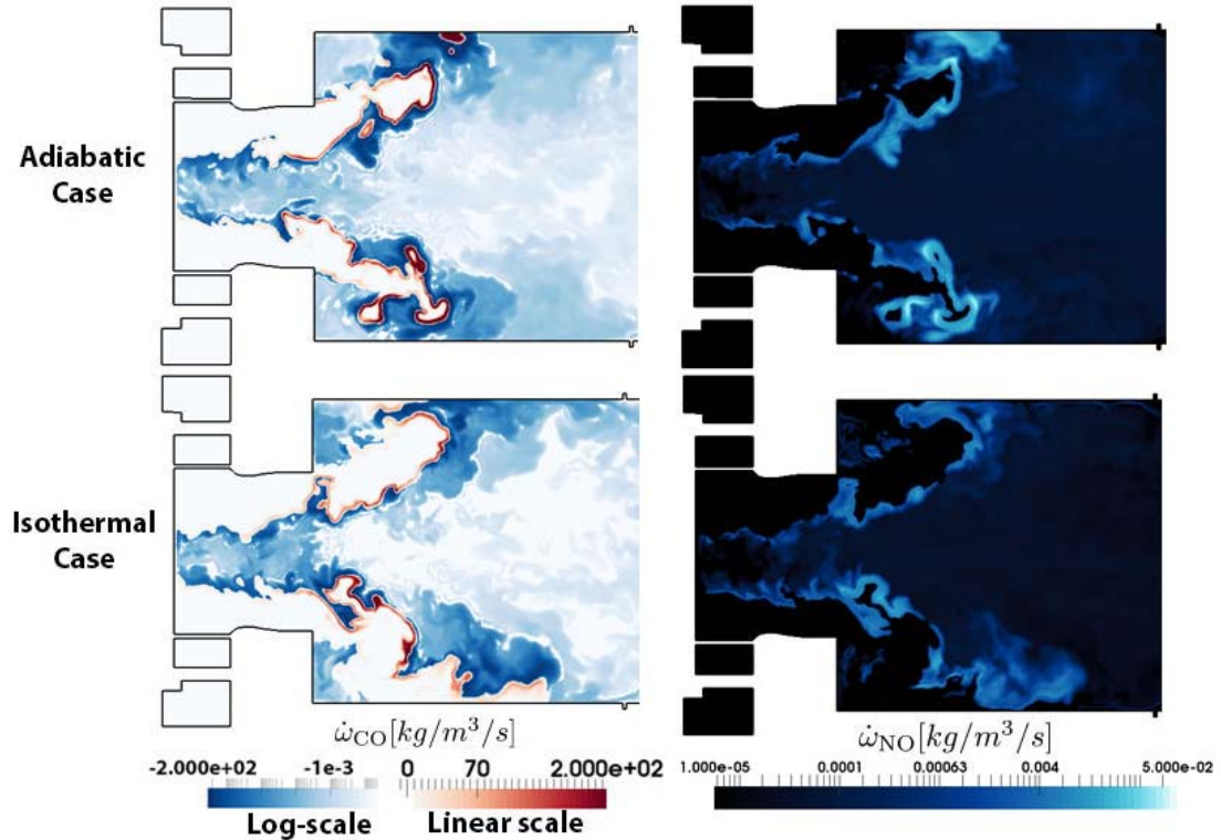
Figure 9.53: SGT-100/Case A: Instantaneous fields of CO source term (left: log-scale for negative values, linear scale for positive values) and NO source term (right - log-scale) from LES in the mid-plane of the combustor. Comparison between adiabatic case (top) and isothermal case (bottom).
