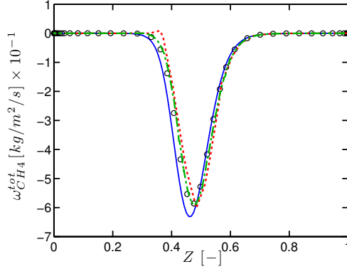
(a) CH 4 source term.
