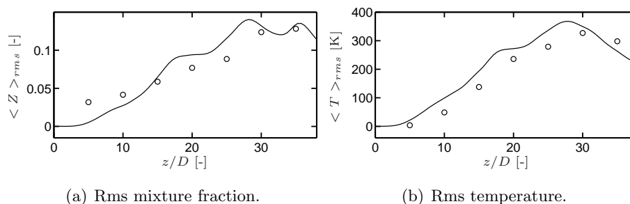
Figure 8.7: Sandia flame D: Axial profiles of a) rms mixture fraction and b) rms temperature fluctuations. – ARC_22, \circ Experimental data.
