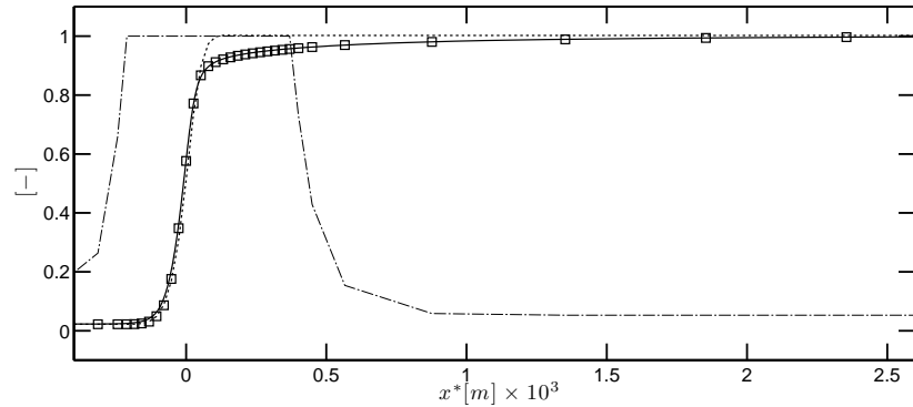
Figure 5.5: Comparison of the NOMAGT model with detailed chemistry on a one-dimensional methane-air premixed flame at \phi = 1.0 : normalised profiles of thickening factor (---), progress variable c_{2s} (···), progress variable c^* ( \square ) and progress variable obtained with Cantera (—).
