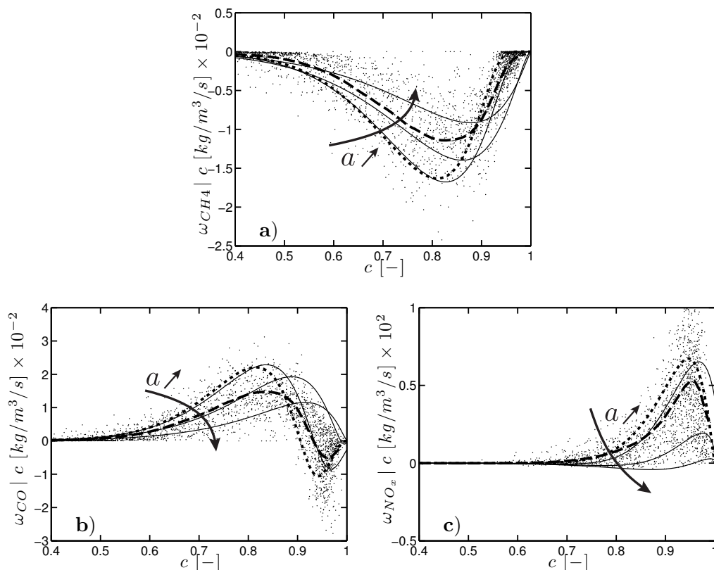
Figure 9.19: SGT-100/Case A: Scatter plot ( \cdot ) and conditional mean ( \text{---} ) of a) \text{CH}_4 , b) \text{CO} and c) \text{NO}_x instantaneous source terms conditionally averaged on progress variable and mixture fraction Z_{glob} . The unstrained laminar premixed flame response ( \text{---} ) and strained laminar premixed flame cases ( \text{---} ) at strain rate a = 1000, 6000, 11000 \text{ s}^{-1} are also shown for comparison.
