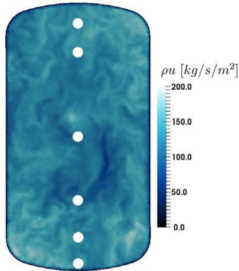
Figure 10.23: LEMCOTEC: Experimental probe locations for exhaust concentration measurements. Color scale: mass flux on an instantaneous snapshot from LES.
