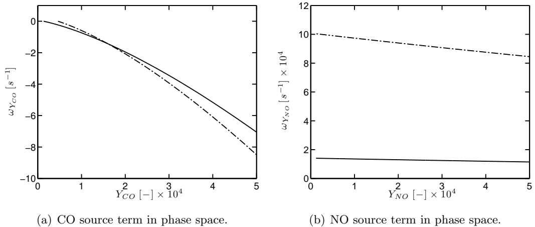
Figure 9.36: Evolution of PSRs in phase space after an initial perturbation of equilibrium composition for Case B , with an equivalence ratio \phi = 0.52 ( - ) and \phi = 0.59 ( \cdot - \cdot - ) using ARC_22_GRI211 .
