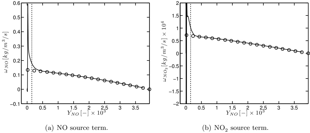
Figure 5.3: a) NO source term and b) \text{NO}_2 source term vs NO mass fraction. Comparison between the NOMANI methodology based on premixed flames (—) and the NORA methodology based on PSRs ( \circ ), for a methane-air mixture at \phi = 1.0 ( T = 680\text{ K} and P = 3\text{ bars} - SGT-100 Case A conditions). The vertical line corresponds to c = 0.98 .
