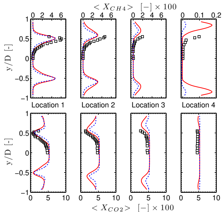
Figure 9.25: SGT-100/Case A - NOMAGT: Transverse profiles of CH_4 mole fraction (top) and CO_2 mole fraction (bottom). Comparison between LES with ARC (—), LES with GRC (---) and experiments ( \square ).
