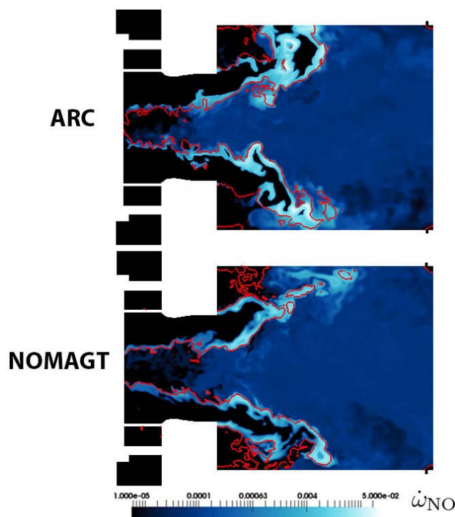
Figure 9.30: SGT-100/Case A - NOMAGT: comparison of instantaneous fields of NO source term ( \text{kg}/\text{m}^3/\text{s} ) between ARC (baseline case) and NOMAGT case in the mid-plane of the combustor. Isocontour of progress variable c = 0.98 for the ARC case, and c^* = 0.98 for the NOMAGT case.
