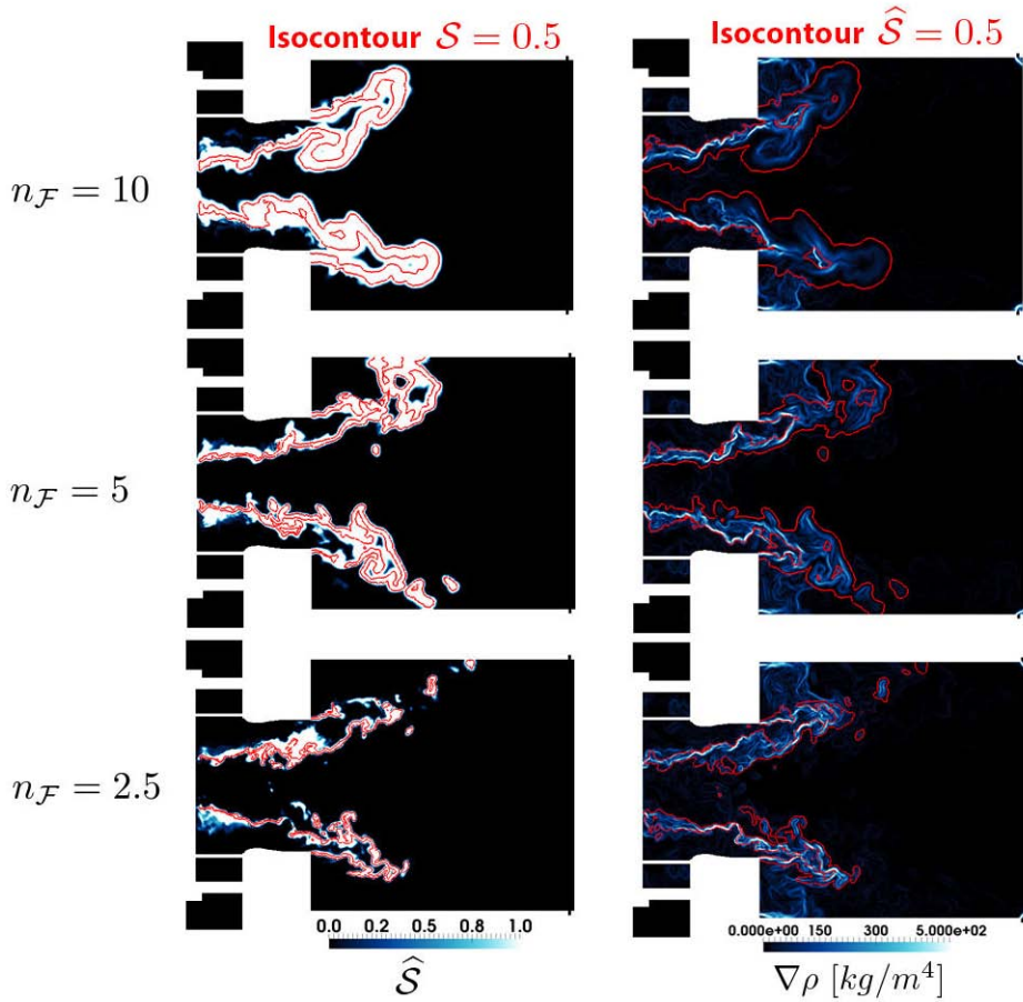
Figure 9.44: SGT-100/Case A: Instantaneous fields from LES in the mid-plane of the combustor, focused on the first half of the combustor. Left: Filtered thickening sensor \widehat{\mathcal{S}} . Right: density gradient. Comparison between n_{\mathcal{F}} = 2.5 (bottom), n_{\mathcal{F}} = 5 (middle, baseline case) and n_{\mathcal{F}} = 10 (top).
