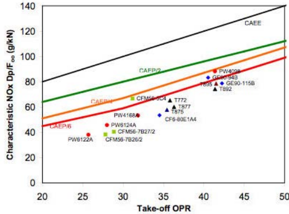
Figure 1.2: \text{NO}_x vs OPR for various engines and comparison with regulatory levels from CAEP. From [1].
