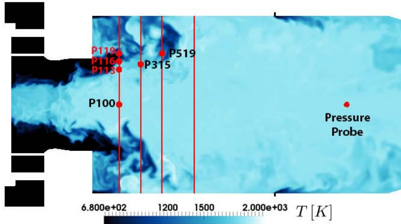
Figure 9.10: SGT-100: location of probes for point data comparison.
