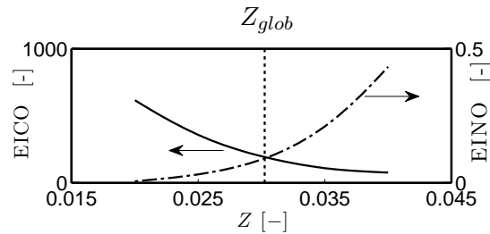
Figure 9.14: SGT-100/Case A: CO (—) and NO (·-·-) flame emission indices of unstrained premixed laminar flames vs mixture fraction. The vertical line corresponds to the global mixture fraction.
