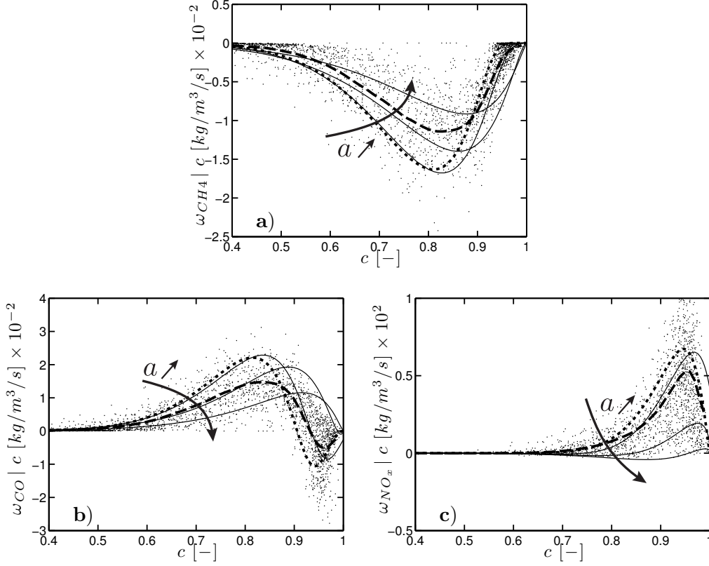
Figure 9.19: SGT-100/Case A: Scatter plot (·) and conditional mean (—) of a) \text{CH}_4 , b) \text{CO} and c) \text{NO}_x instantaneous source terms conditionally averaged on progress variable and mixture fraction Z_{glob} . The unstrained laminar premixed flame response (▪▪) and strained laminar premixed flame cases (—) at strain rate a = 1000, 6000, 11000 \text{ s}^{-1} are also shown for comparison.
