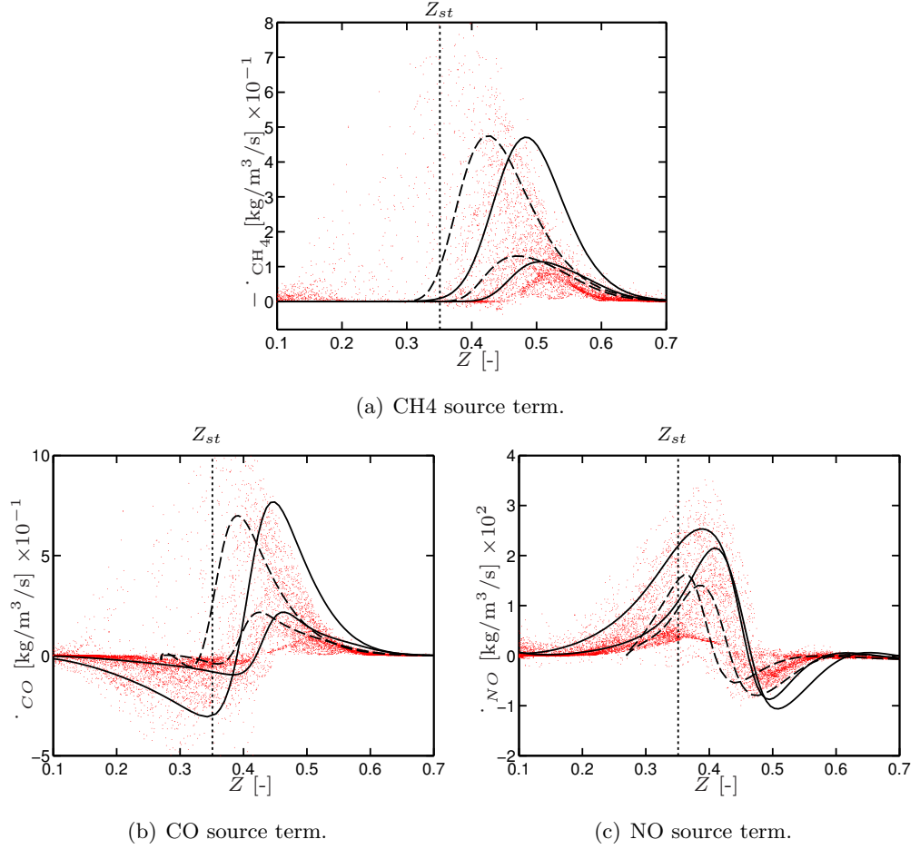
Figure 8.16: Sandia flame D: Scatter plot of CH 4 , CO and NO source terms vs mixture fraction at axial location z = 7.5D . Comparison of coflow (—) and pilot (---) counterflow flames at strain rates a = 60 \text{ s}^{-1} and 270 \text{ s}^{-1} .
