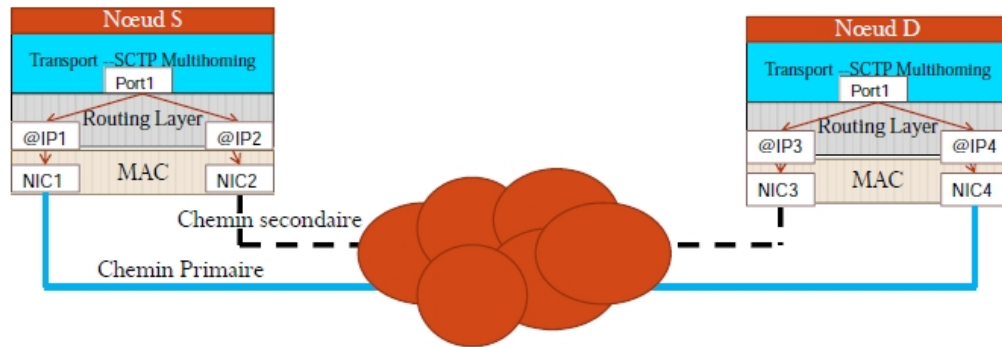
FIGURE 1.5 – Exemple de multidomiciliation SCTP
