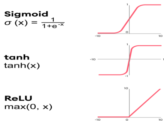
Figure 3.5: Activation Functions.
