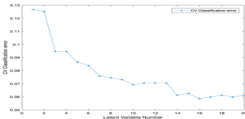
Figure 5.3: Classification Error of the PLSDA model.
