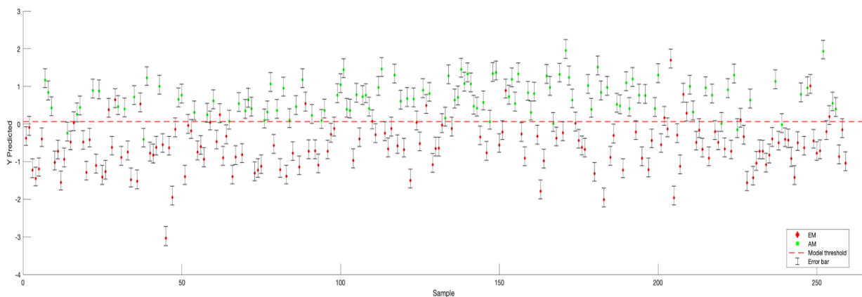
Figure 5.6: Samples predictions and confidence intervals on the validation dataset.
