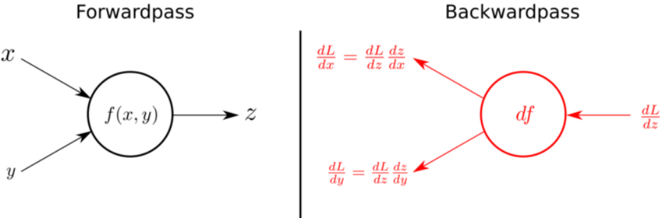
Figure 3.6: back-propagation vs forward--propagation.
