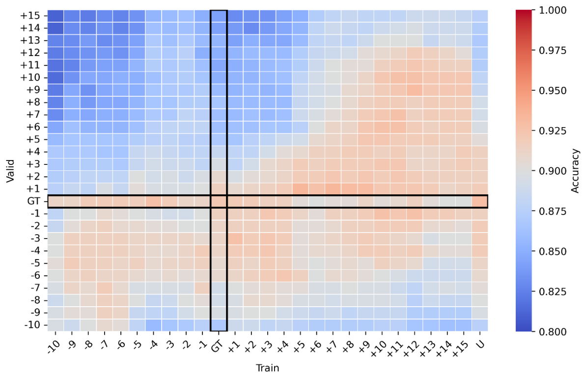
Figure 5.12: Effect of segmentation accuracy on classification performance.
