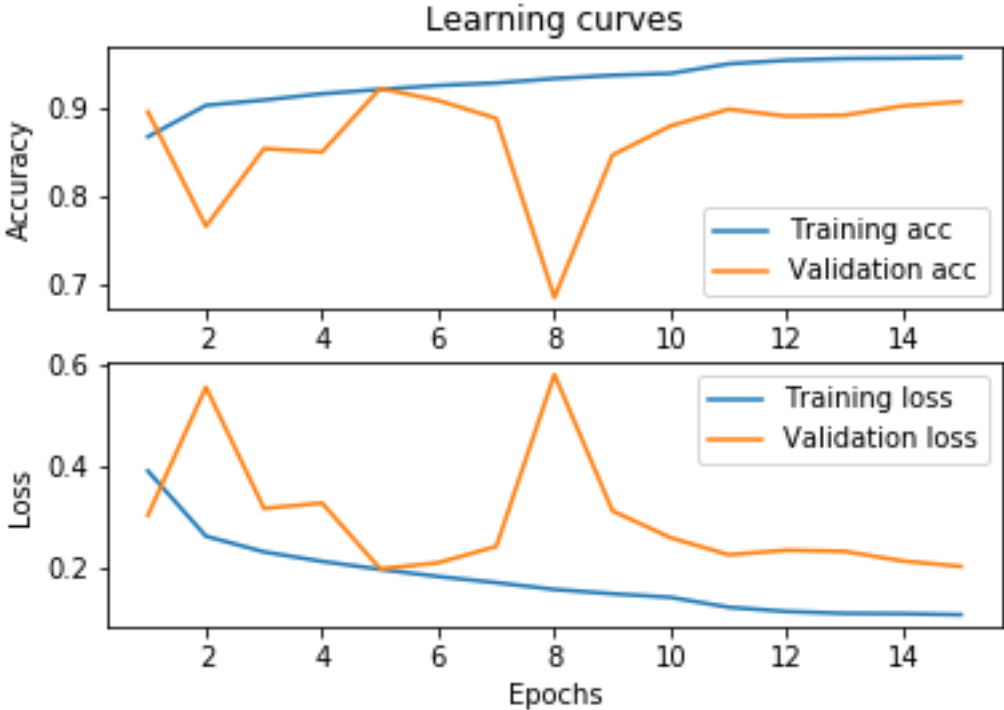
Figure 6.7: Classical Unet training curve with mycetoma database.
