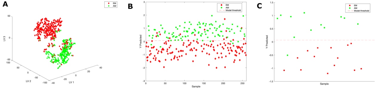
Figure 5.4: (A): 3D projection of mycetoma validation data on the first three latent variables. (B): Class predictions on a primary validation set. (C): Class predictions on the secondary dataset.
