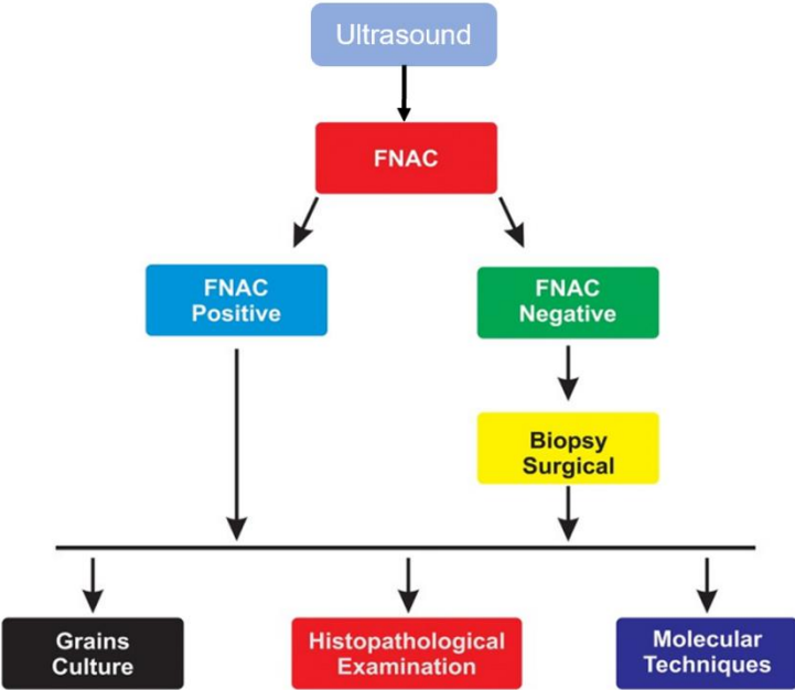
Figure 2.9: Mycetoma Diagnosis Flowchart.
