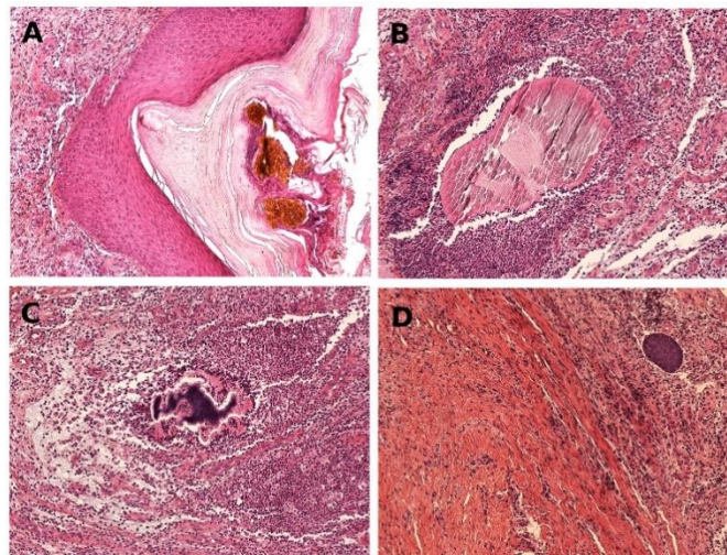
Figure 2.7: Histopathological appearance of mycetoma grains in H&E stain, magnified X10. (A): M. mycetomatis . (B): S. somaliensis . (C): A. madurae . (D): A. pelletieri .
