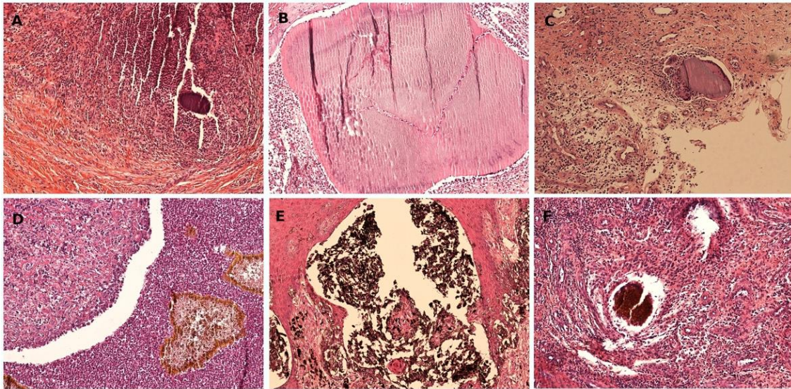
Figure 5.10: Grains which score greatest and smallest score for selected VIPs. Actinomycetoma grains (lowest score) are depicted in the top row and eumycetoma in the bottom row (highest score). (A, D): Difference variance, (B, E): Small dependence low-grey-level emphasis (peak feature), and (C, F): Grey-level variance.
