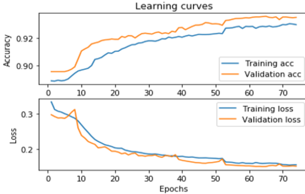
Figure 6.5: Training curves of GrUnet on mycetoma database.
