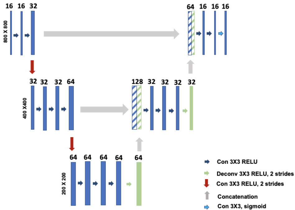
Figure 6.4: Proposed GrUNet Architecture.
