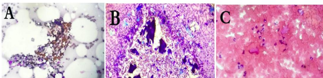
Figure 2.8: FNA of some mycetoma causative agents stained with H&E. (A): M. mycetomatis . (B): A. pelletieri . (C): S. somaliensis .
