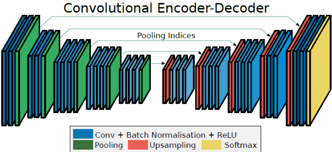
Figure 6.1: SegNet Architecture
