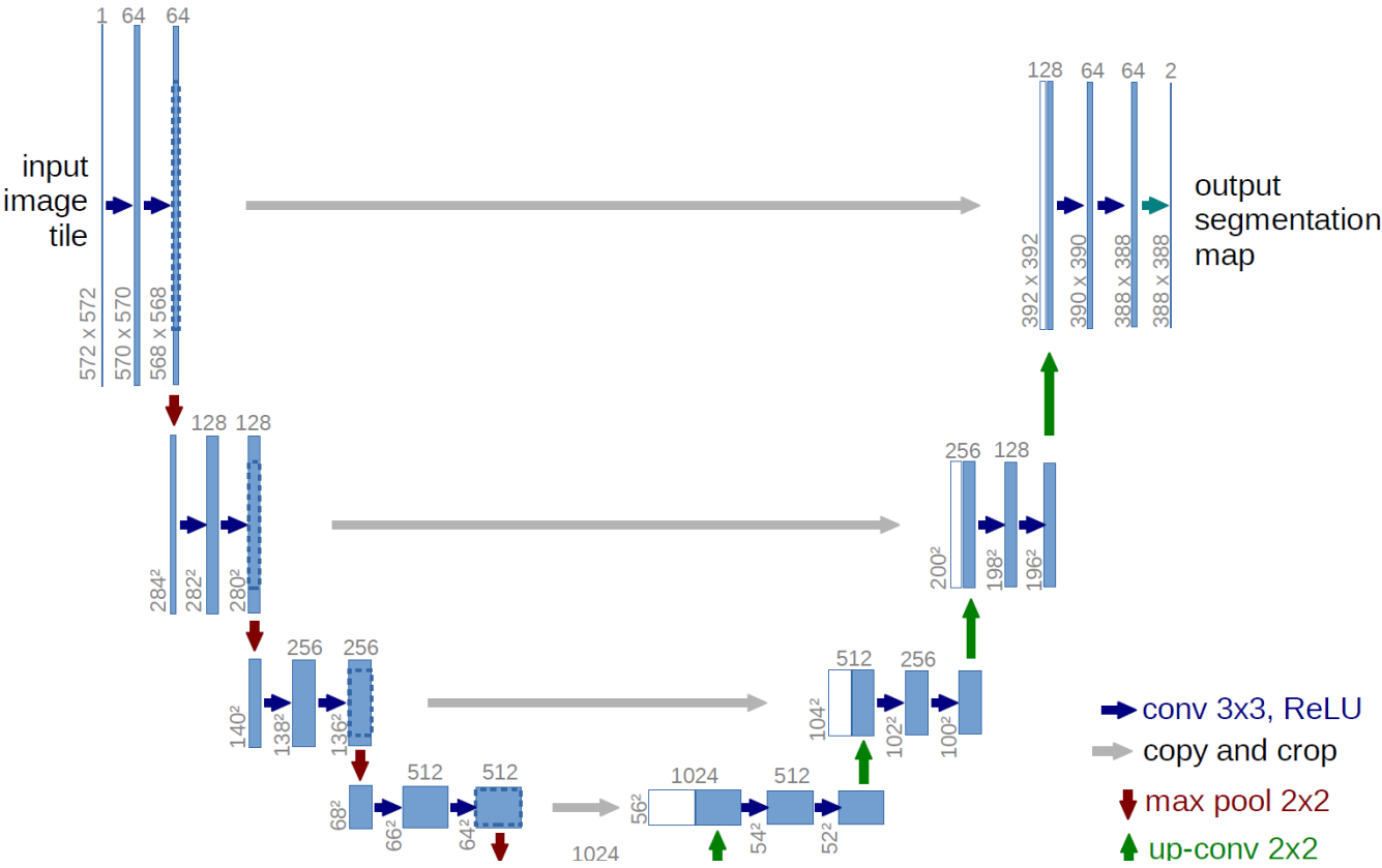
Figure 6.2: U-Net architecture [85].
