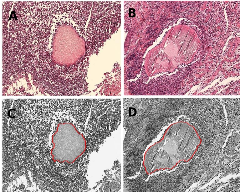
Figure 5.2: Sample grains of Eumycetoma (left) and Actinomycetoma (right). (A, B): tissue sections stained with H&E; (C, D): manual segmentation of the grains.
