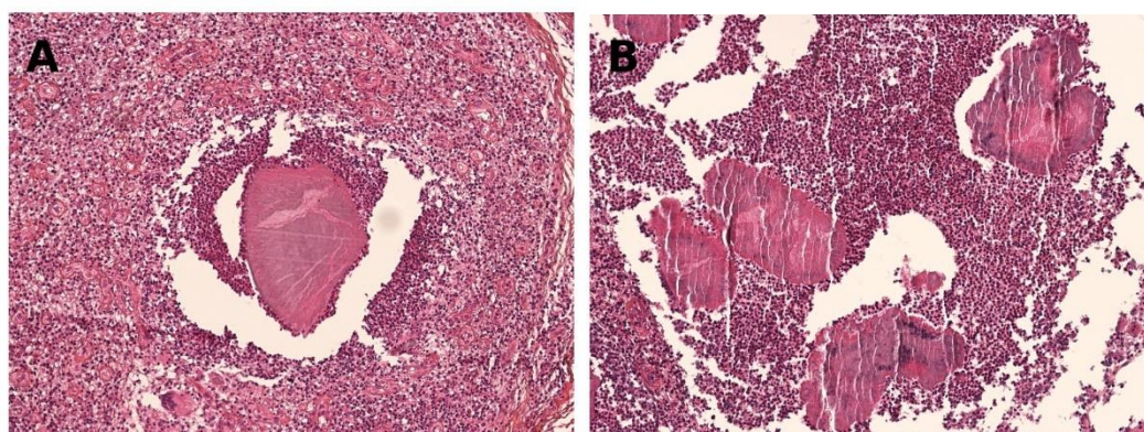
Figure 4.5: Mycetoma Microscopic Images. (A): Single grain. (B): Multiple grains.
