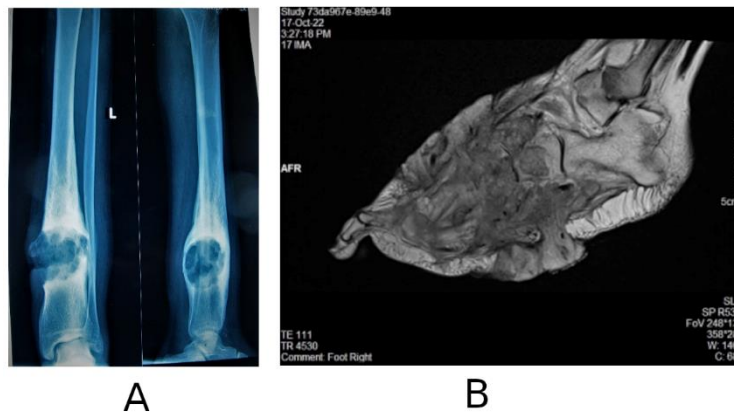
Figure 2.4: Some of mycetoma imaging techniques. (A): X-Ray of the leg shows a massive eumycetoma cavity. (B): MRI showing massive actinomycetoma affected soft tissues and bones.
