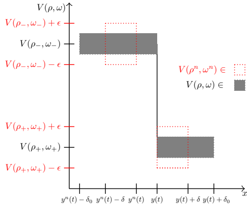
Case 1: V(\rho_-, w_-) < V_b - \epsilon and V(\rho_+, w_+) < V_b - \epsilon
