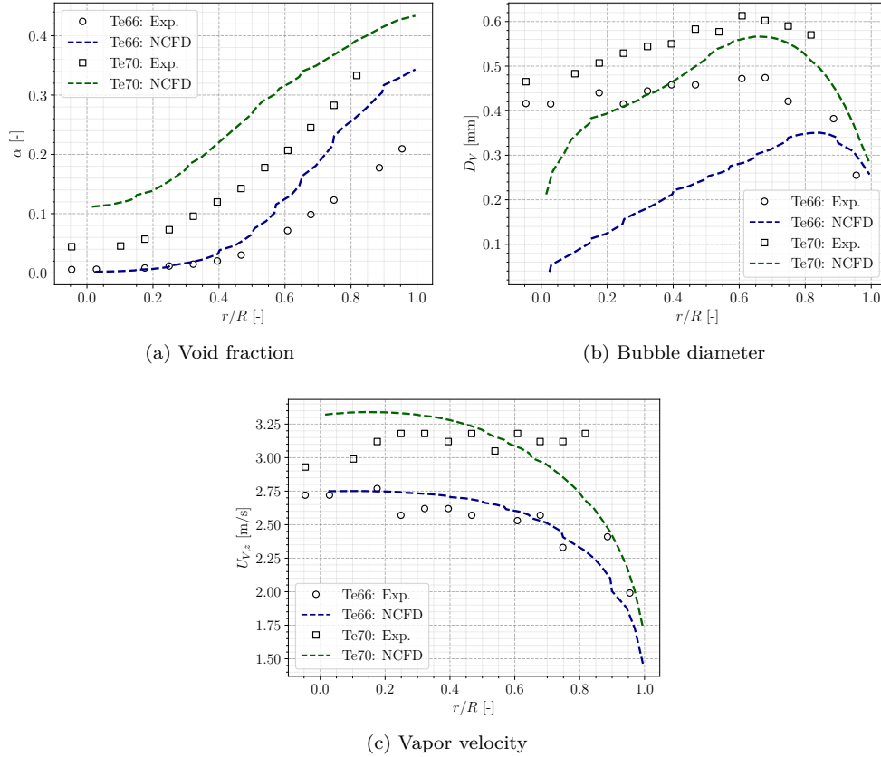
Figure 4.8: Simulation results for cases 30G2P26W16Te66 &amp; Te70
