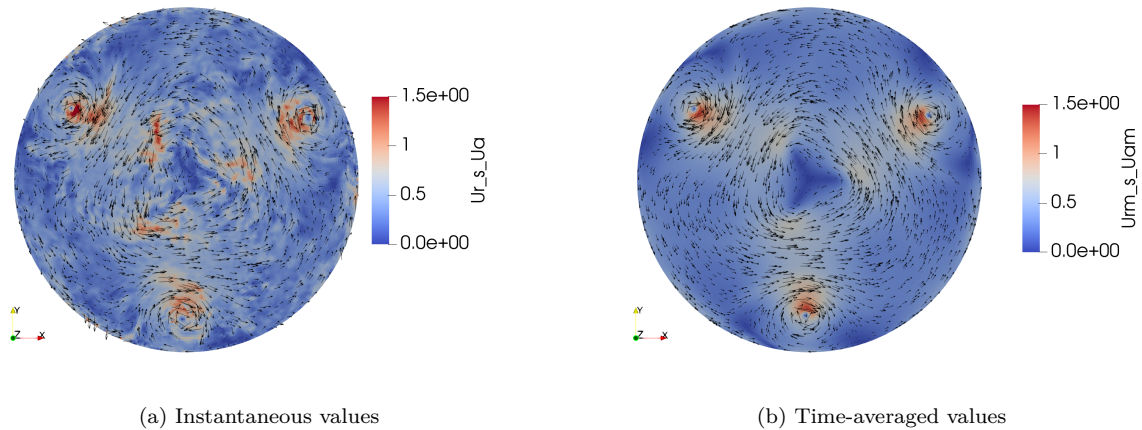
Figure 11.6: Visualization of the radial velocity field and ratio between radial and axial velocity obtained with the LES, z = 1 D_h downstream the MV.
