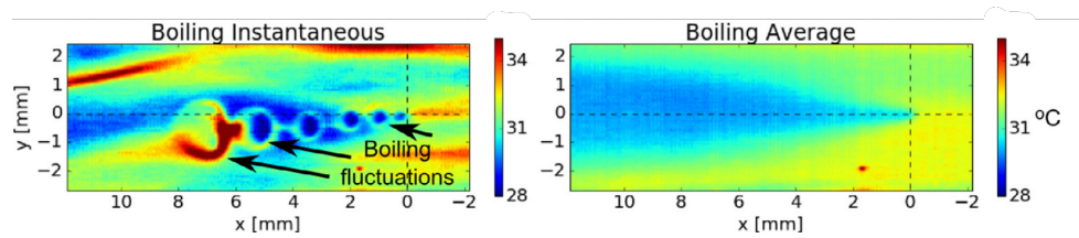
(a) Instantaneous and time-averaged wall temperature in boiling regime visualized and adapted from Estrada-Pérez et al. [43].
