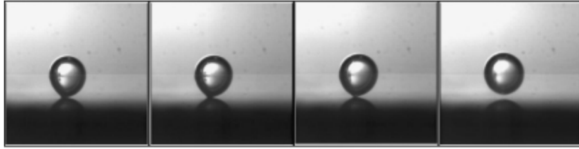
Figure 6.27: Visualization of bubble lift-off in horizontal boiling conducted by and adapted from Maity [108]. The detachment the the bubble base from the surface is clear in the last frame.
