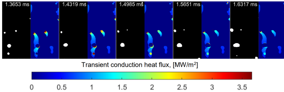
(b) Transient conduction induced by sliding bubbles visualized and adapted from Kossolapov [90].
