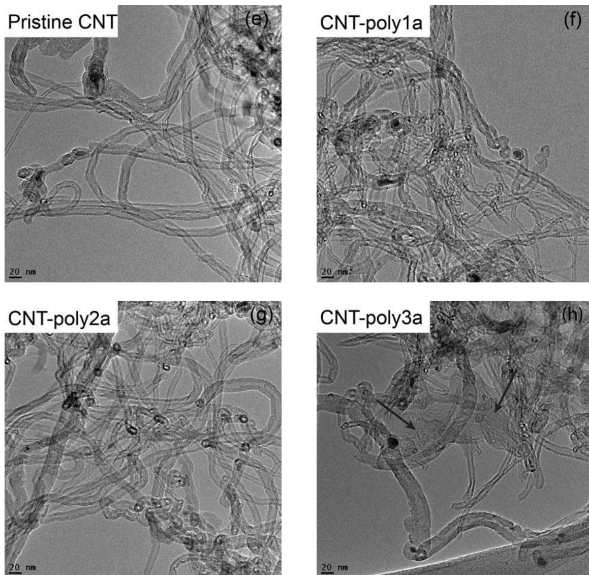
Figure II.24. TEM images of pristine CNT, CNT– poly1a , CNT– poly2a and CNT– poly3a at (a-d) high magnification (scale bar = 5 nm) and (e-h) low magnification (scale bar = 20 nm).
