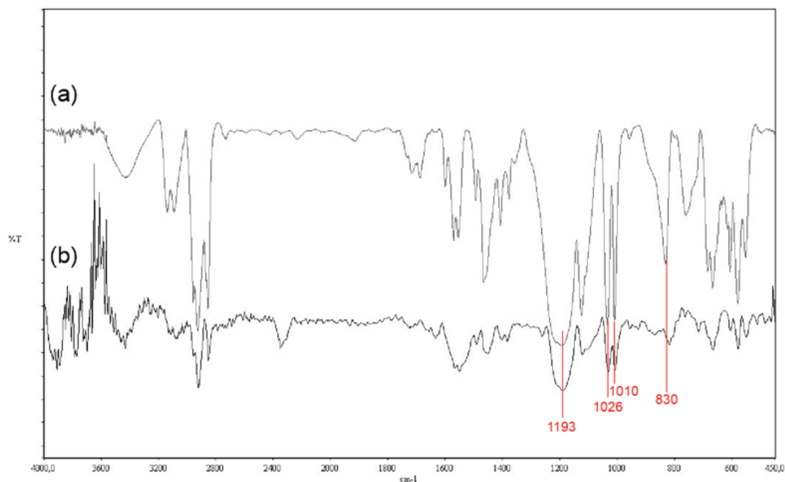
Figure III.5. FTIR spectra of (a) poly[VEIM]DBS (b) CNT-poly[VEIM]DBS.
