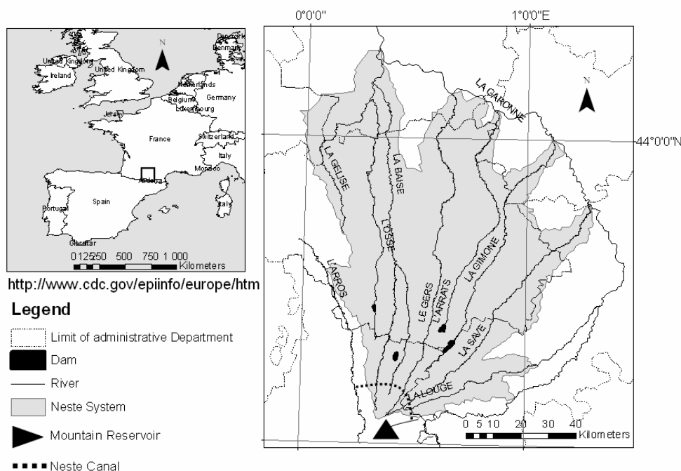
Figure 15: The Neste System (from Clavel et al., 2009, in review)
