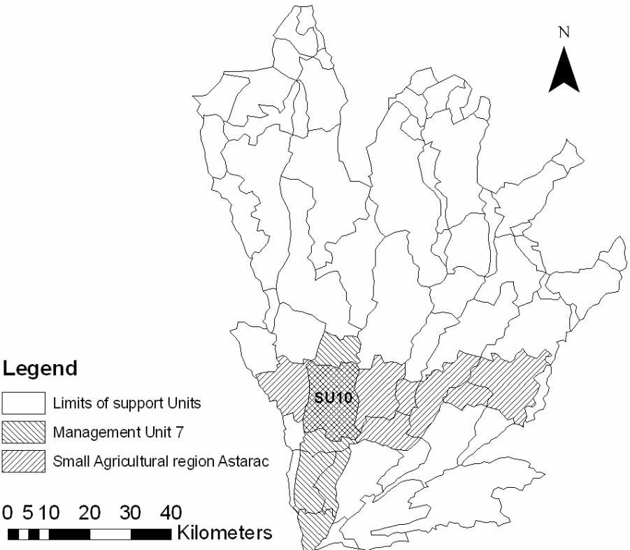
Figure 17: Division into support units of the Neste system. Support unit 10 (SU10) belongs to management unit 7 and to Astarac small agricultural region
