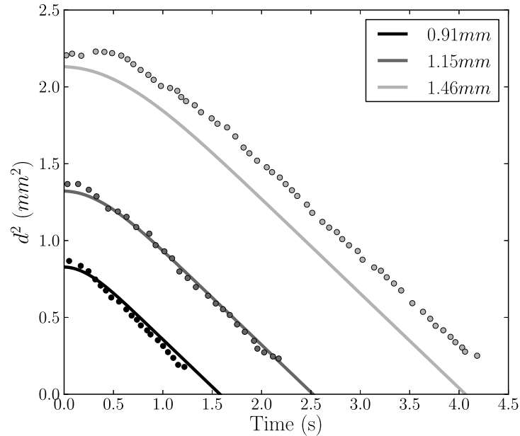
Figure 8.22 : Comparison with experiment : evolution of n -decane burning droplets in atmospheric conditions. Experiments from Xu et al. [226].
