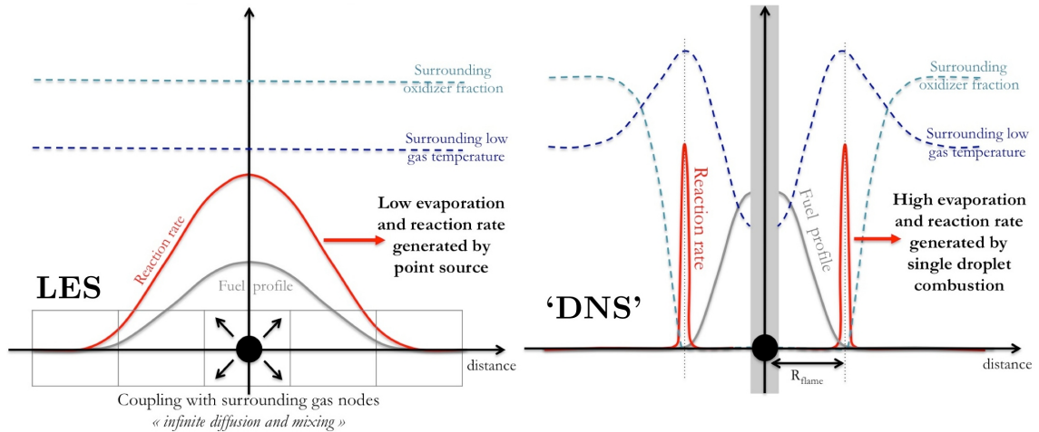
Figure 8.13 : Combustion around an evaporating droplet using the classical evaporation model on a LES mesh (left) compared to the real physical situation of a single droplet combustion.
