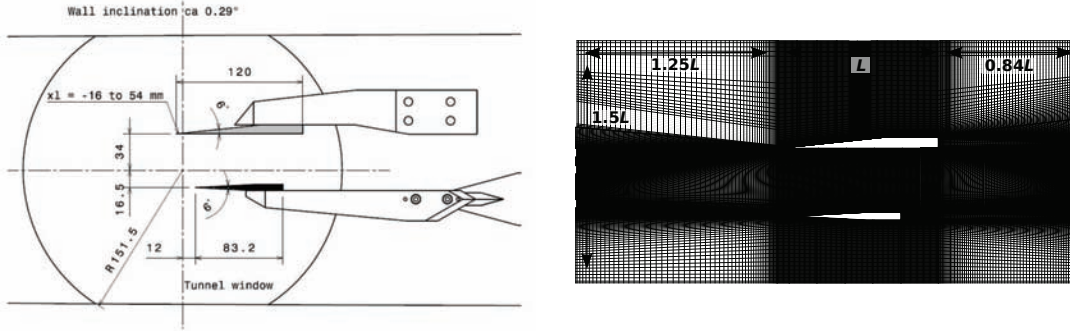
FIGURE 1. Left: Side view of the experimental geometry; right: computational grid for the DDES (mid-span plane) and main dimensions
