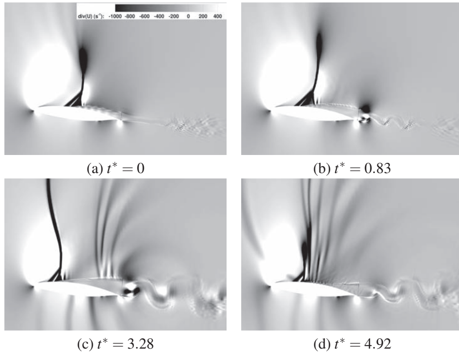
Figure 17: Divergence of velocity field - OES- k - \varepsilon
