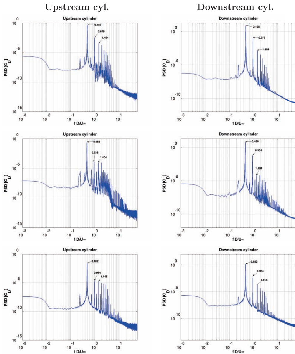
Figure 2.11: PSD of the drag coefficient time evolution for the two cylinders. Top: SA, middle: k\text{-}\omega\text{-SST} , bottom: k\text{-}\omega\text{-BSL} .
