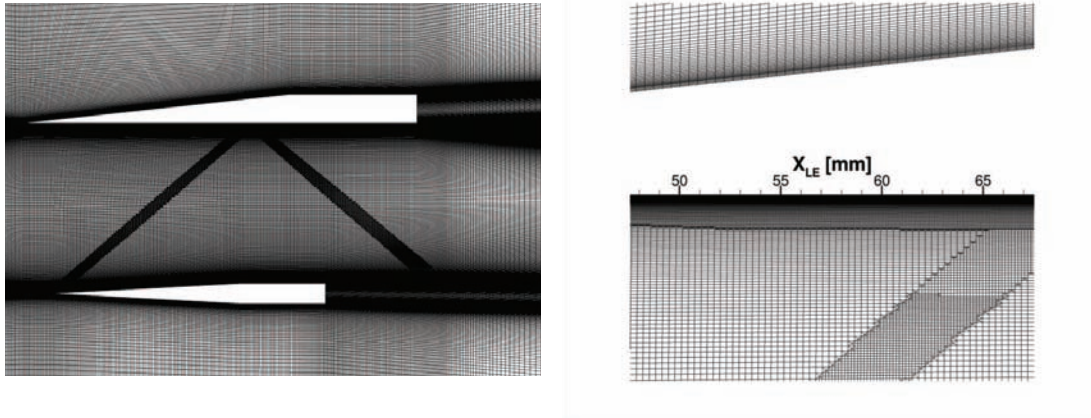
FIGURE 2. WM-LES mesh: (left) computational grids near flat-plate and shock-generator models; (right) enlarged image in the middle of the flat plate
