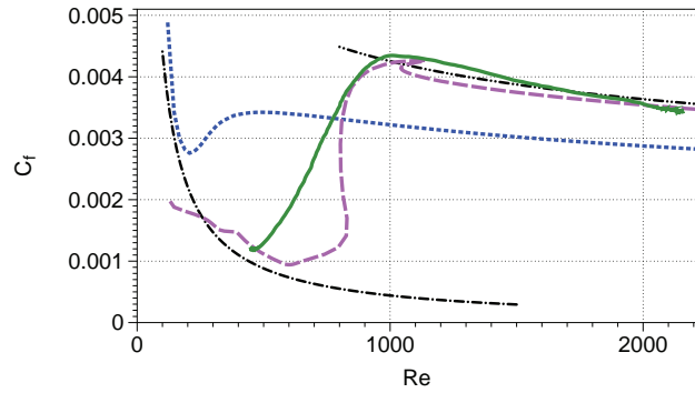
FIGURE 3. Upstream skin-friction coefficient distribution: - - - Blasius, - - - von Kármán & Schoenherr, ····· DDES, - - - DDES (transitional), — WM-LES
