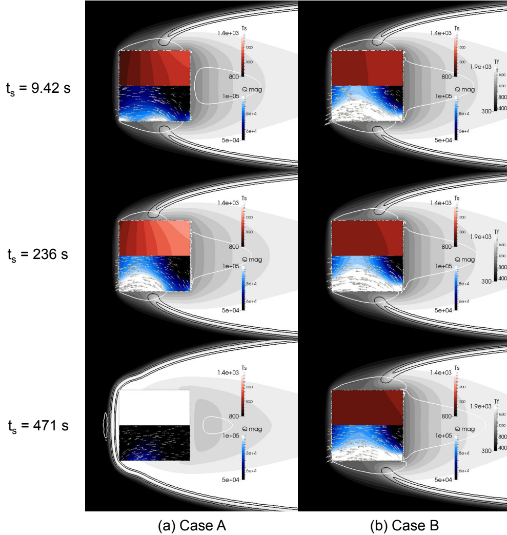
Figure 6.14: Instantaneous temperature fields of two cases for which T_{init} = 1000 K and the solid conductivity equals either \lambda_A^s or \lambda_B^s in both fluid and solid domains with heat release contours at HR = 10^8 J.m^{-3}.s^{-1} (outer flame contour) and HR = 10^9 J.m^{-3}.s^{-1} (inner most flame contour) in black and zero velocity contour in white. The solid domain is indicated with the white square. For both computations, results are given from top to bottom at nit_{cpl} = 2000, 50000 and 100000 corresponding respectively in the solid time scale to t_s = 9.42, 236 and 471 s.
