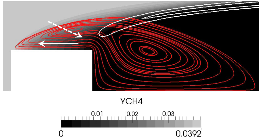
Figure 5.6: CH_4 mass fraction field with heat release contours at HR = 10^8 \text{ J.m}^{-3}.\text{s}^{-1} (outer flame contour) and HR = 10^9 \text{ J.m}^{-3}.\text{s}^{-1} (inner most flame contour) in white and streamlines in the recirculation zone (red) in the vicinity of the flame holder on the top half of the domain for the baseline case ( T_w = 700 \text{ K} ).
