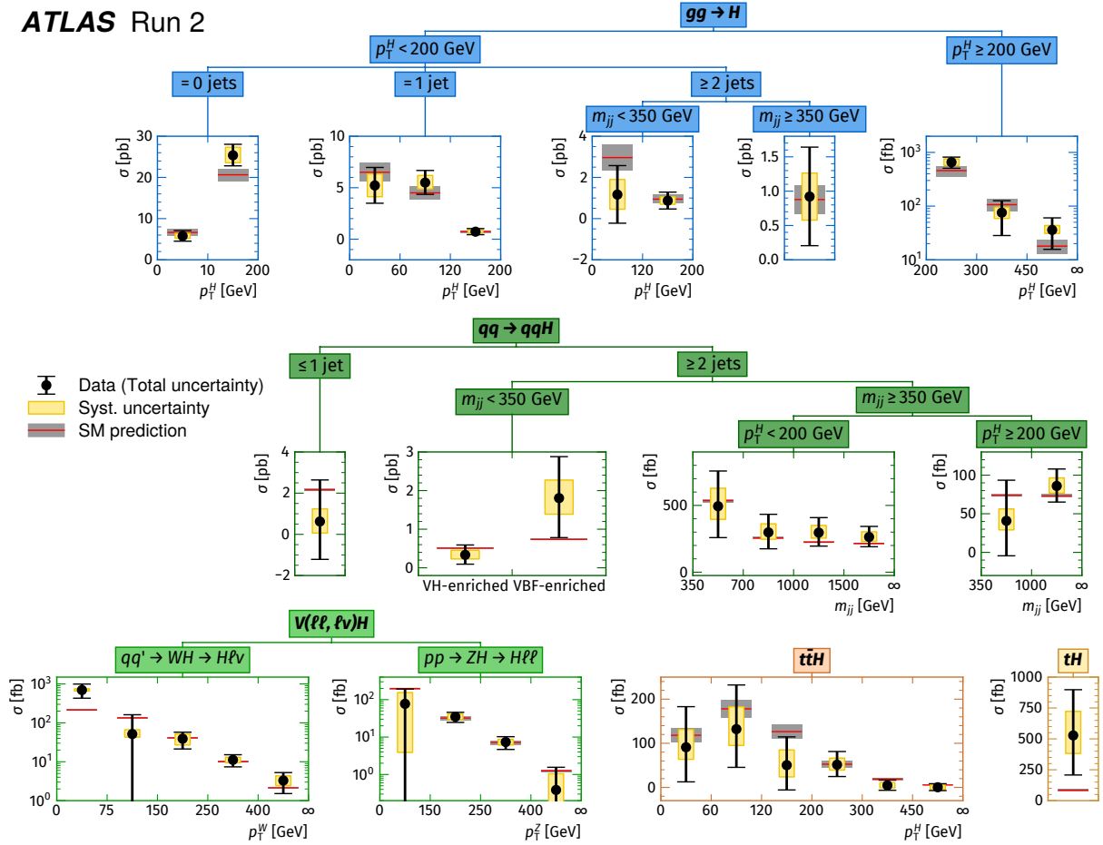
Figure 1.13: Combined measurement of the STXS cross-sections. Source: [26].
