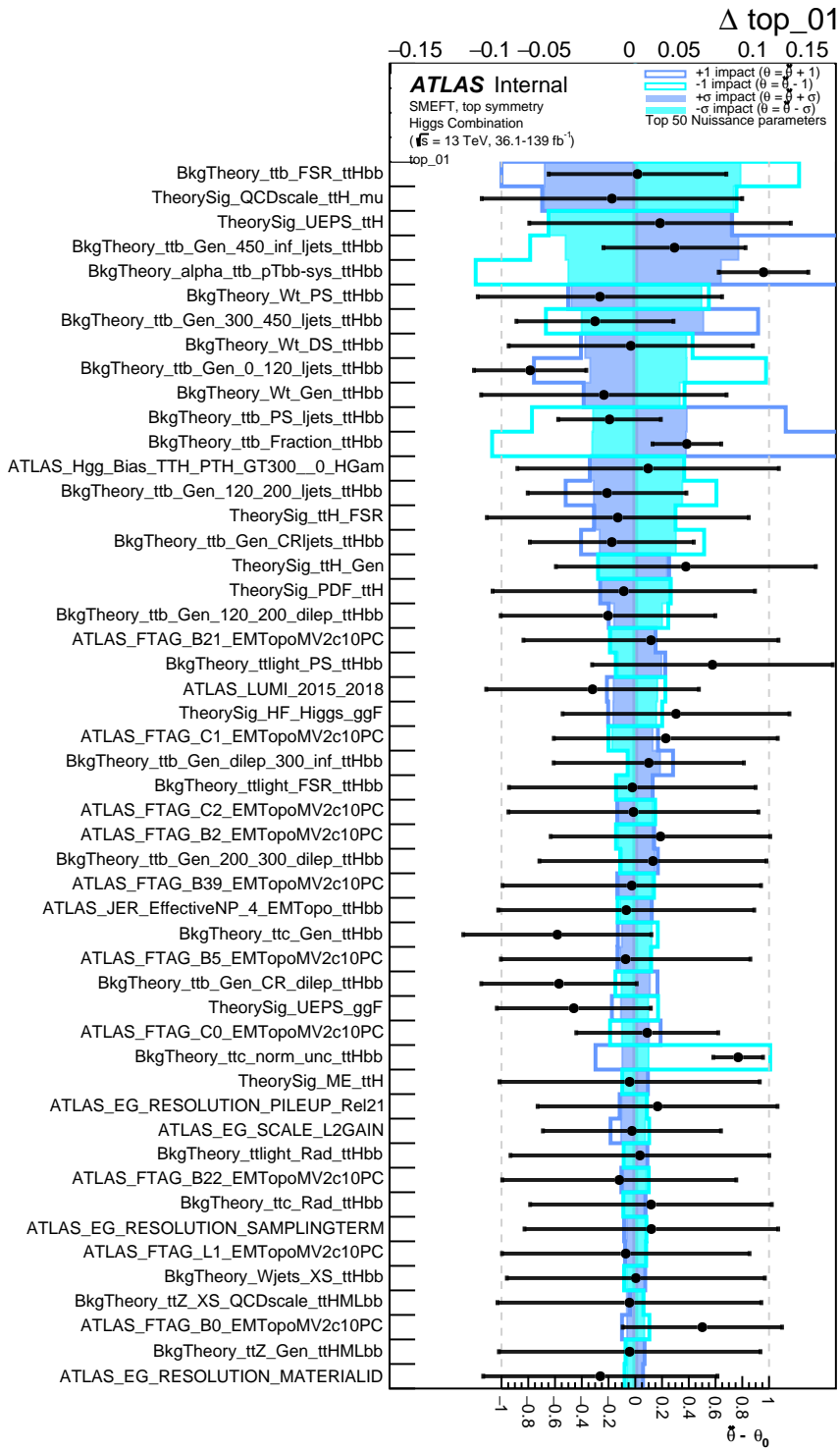
Figure A.14: Example of nuisance parameters ranking for a combined Higgs EFT measurement for the \text{top}_{01} Wilson coefficient. Rows are ranked according to the sum of the squares of post-fit impacts on the POI. Transparent (shaded) areas show the pre-fit (post-fit) impact: change in the POI central value after changing the nuisance parameter value to its best-fit-value \pm 1 ( \pm\sigma ). The corresponding axis is on the top of the plot. Black dots show best-fit-values of the nuisances and their errors. Values are encoded in the bottom axis. The colours represent the results of positive and negative variations of the systematics.
