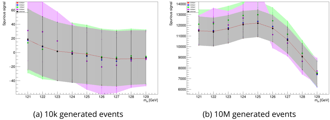
Figure 4.23: Example of spurious signal study on the bin size for a given number of generated events. A set of events following ExpPoly2 distribution has been generated and fit using the same functional form. The unbinned fit (black) and the tiniest among studied once (0.5 GeV) has shown the smallest bias.
