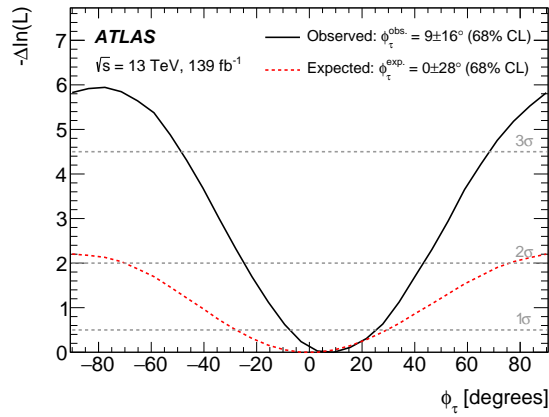
Figure 1.15: Measurement (expected and observed) of the CP mixing angle \phi_\tau . Source: [44].
