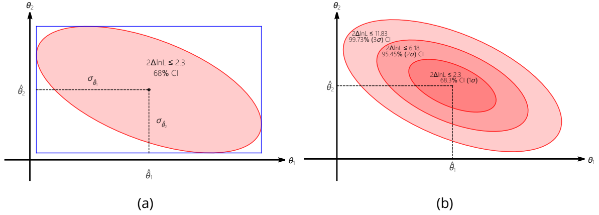
Figure A.5: Illustration of a 2D likelihood contour (a) fulfilling the condition of 2\Delta \ln \mathcal{L} \leq 2.3 , giving 68% CI (confidence interval). The maximum likelihood point (black dot in the center of the ellipse) gives ML (minimum likelihood) best-fit-value \hat{\theta}_1 and \hat{\theta}_2 for the parameters \theta_1 and \theta_2 , respectively. Blue surrounding lines give 68% CI for the parameters independently, which is the level of 1\sigma error. Figure (b) shows 1, 2 and 3\sigma uncertainty levels and the corresponding thresholds for the likelihood contours.
