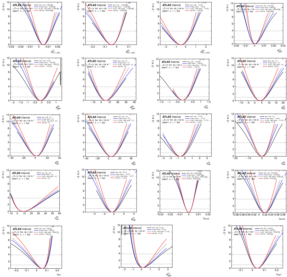
Figure C.10: Observed NII scans (black) and the ones for the case of fixing given groups of systematics to the best-fit-values (blue for fixed background theoretical ones, grey for fixing signal theoretical ones on top to the previous and red is the stat-only). Source: [135].
