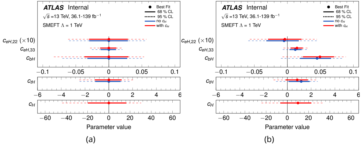
Figure 5.26: The expected (a) and observed (b) constraints for the 2HDM matching. The red and blue lines shown the constraints obtained separately for the scenarios with and without c_H , respectively. Source: [135].
