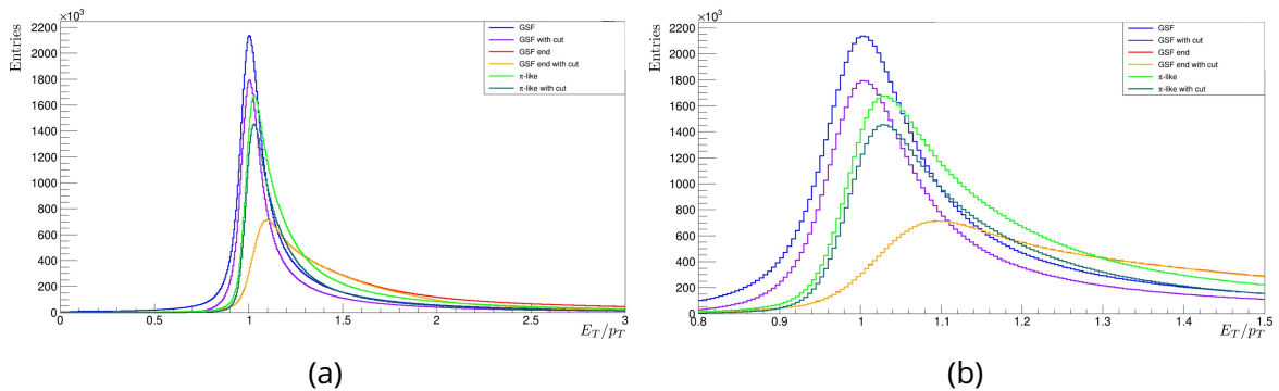
Figure 3.6: E_T/p_T distributions for various electron p_T types with and without cut on f_{brem} < 0.5 . The (b) plot is zoomed in E_T/p_T . Source: [76].
