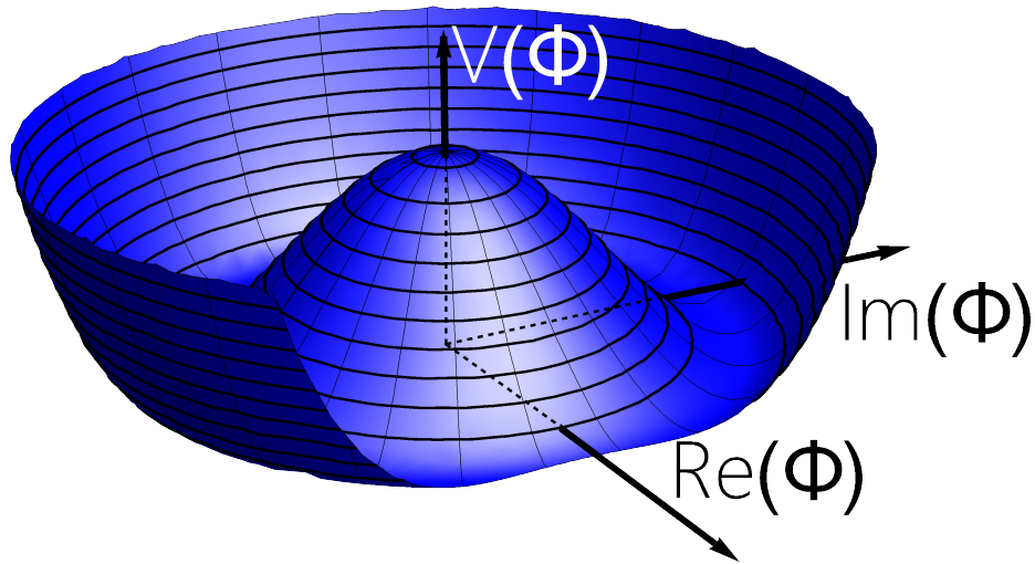
Figure 1.2: Illustration of the Higgs potential.
