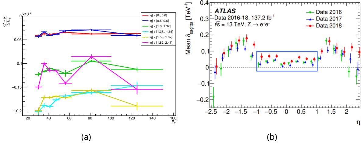
Figure 3.19: Comparison of the official sagitta bias measurement (b) to (a) the estimation with E_T/p_T method in this study (same as Fig. 3.18). One sees that for the central region of the detector |\eta| < 1.0 the official value \delta_{sagitta}^{official} \approx 0.05 \text{ TeV}^{-1} which is in a good agreement with the value from E_T/p_T study \delta_{sagitta}^{E/p} \approx 0.045 \text{ TeV}^{-1} . Source: [76].
