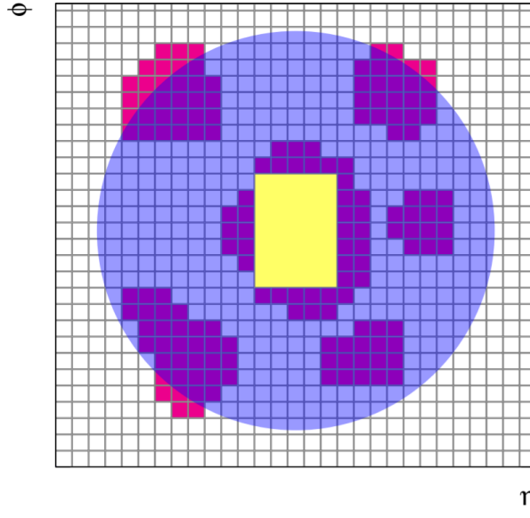
Figure 4.9: Schematic of the calorimeter isolation. The grid represents the cells of the second layer of the calorimeter in \eta \times \phi directions. The prompt photon candidate mostly deposits energy in the centre of the rectangle window (yellow). The blue cone represents the isolation cone. All topological clusters (red), for which the barycentres fall within the isolation cone are included in the computation of the isolation variable. The energy deposited in the \Delta\eta \times \Delta\phi = 0.125 \times 0.175 window of the 5 \times 7 cells (yellow) is subtracted in the computation. Source: [74].
