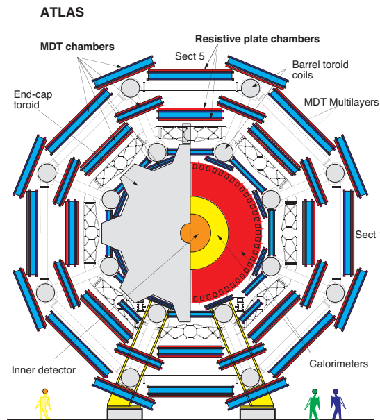
Figure 2.11: Cross-section of the ATLAS Muon Spectrometer. Source: [59].
