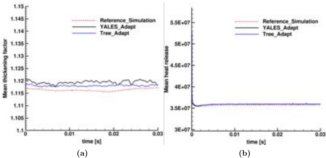
Figure 4.21: Comparison of (a) the mean thickening factor and (b) the mean heat release in the chamber for all the simulations.
