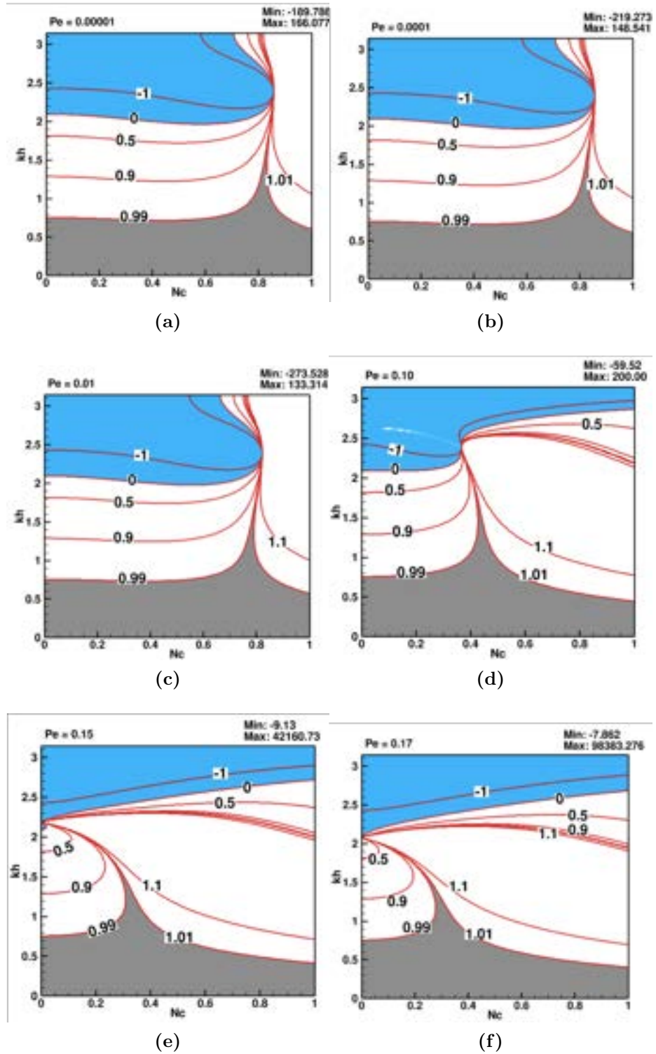
Figure 2.8: Contours of v_{g,num}/v_{g,phy} as a function of kh and Nc for mentioned values of Pe for the TTGC- CD_2 scheme. The regions of q-waves are colored in blue, while DRP regions are shaded in grey.
