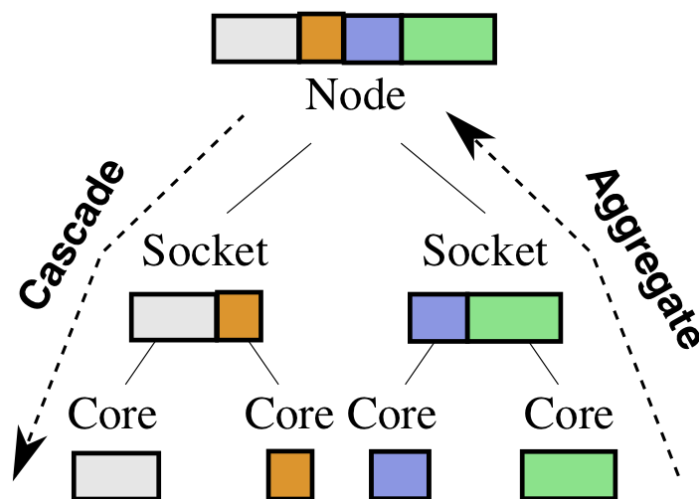
Figure 4.5: Structure of hardware topology for MPI Tree.
