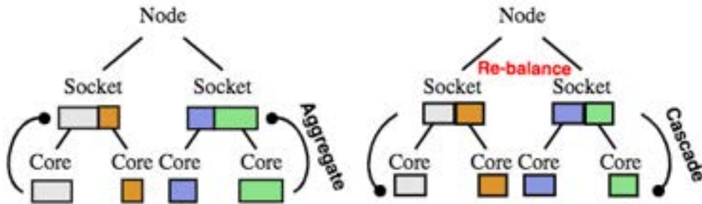
Figure 4.7: Rebalancing at a shared memory hierarchical level is three step process, aggregation, rebalance and cascade.
