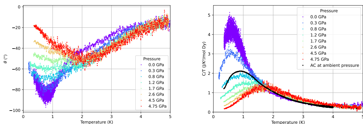
Figure 5.4.4: (left) Phase differences as a function of temperature for various pressures, offset so that they all are at -15^\circ at 5 K. (right) Effective C/T using the adjusted phase differences. The data was scaled to match as well as possible with the lowest frequency data discussed in the previous section, shown in black.
