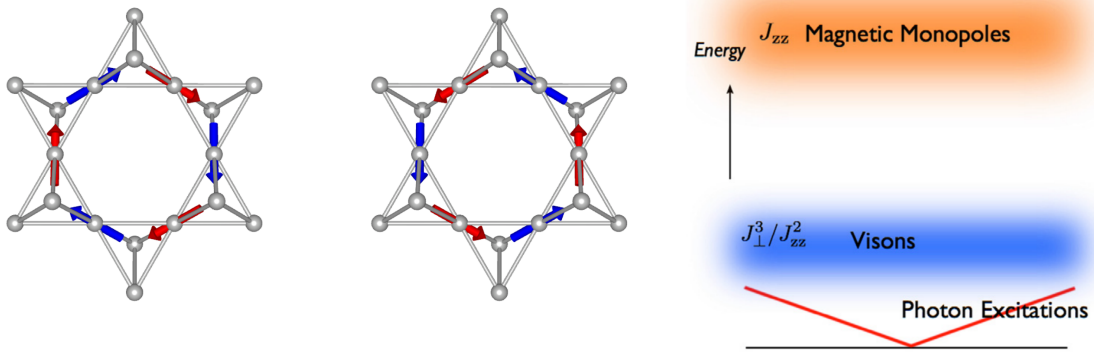
Figure 1.3.2: (left) Ring exchange tunnelling process and (right) Energy scales of the various novel excitations in quantum spin ice.
