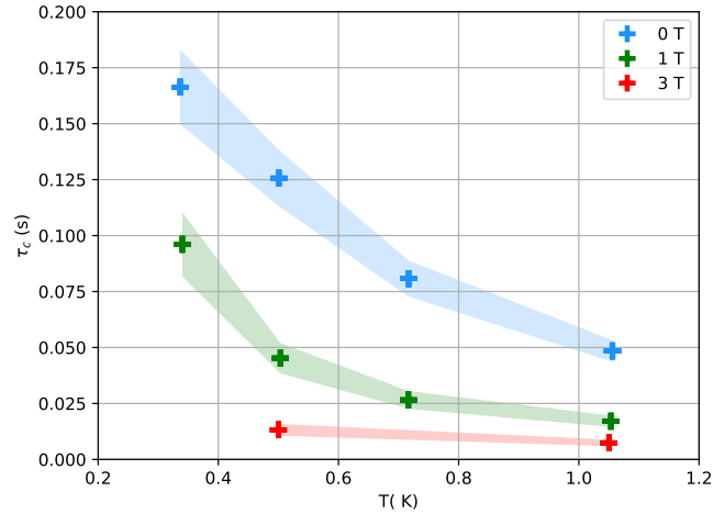
Figure 5.3.5: Decoupling time \tau_c as a function of temperature, for various fields. The shaded areas correspond to the relative uncertainty in the fit of the model.
