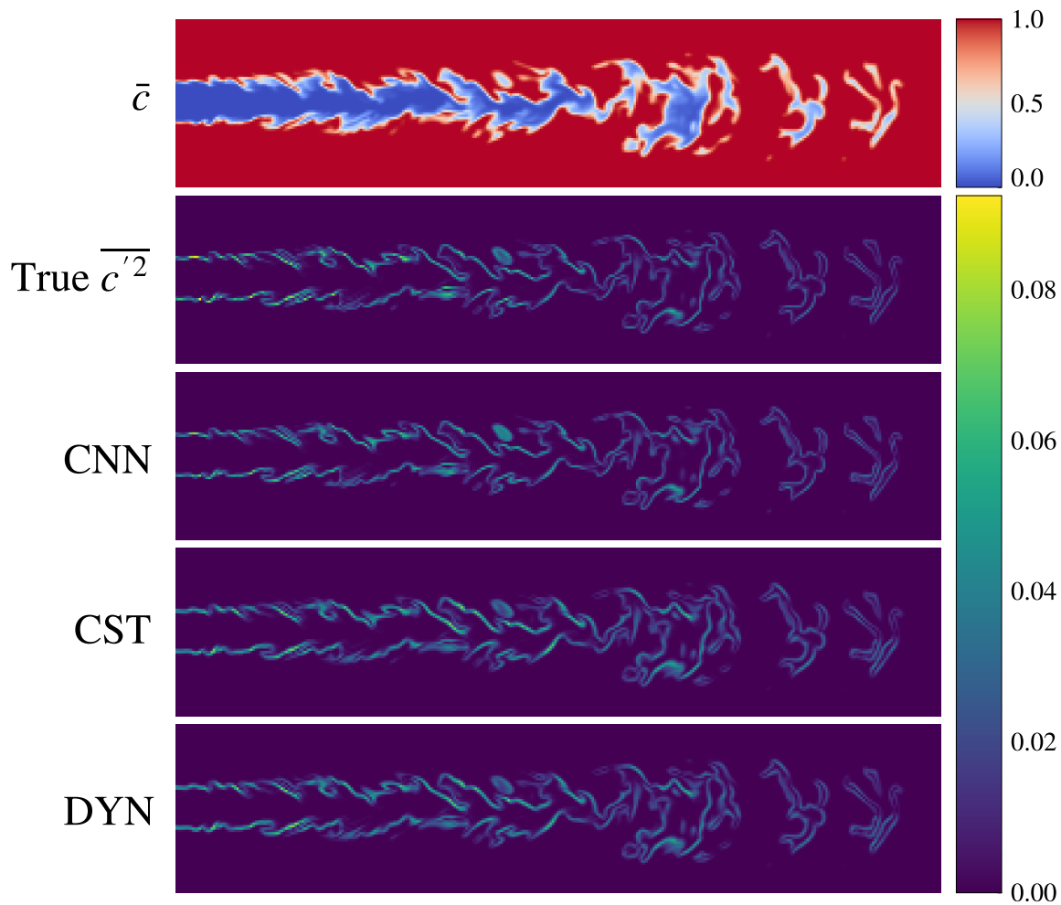
Figure 6.14: Sample R2 slices of \bar{c} , true c'^2 , CNN, CST, and DYN model predictions.
