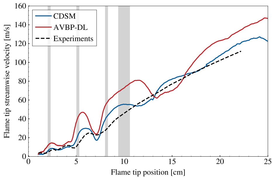
Figure 8.30: Evolution of the flame tip streamwise velocity with respect to the flame tip position. The obstacles are represented as grey vertical areas.
