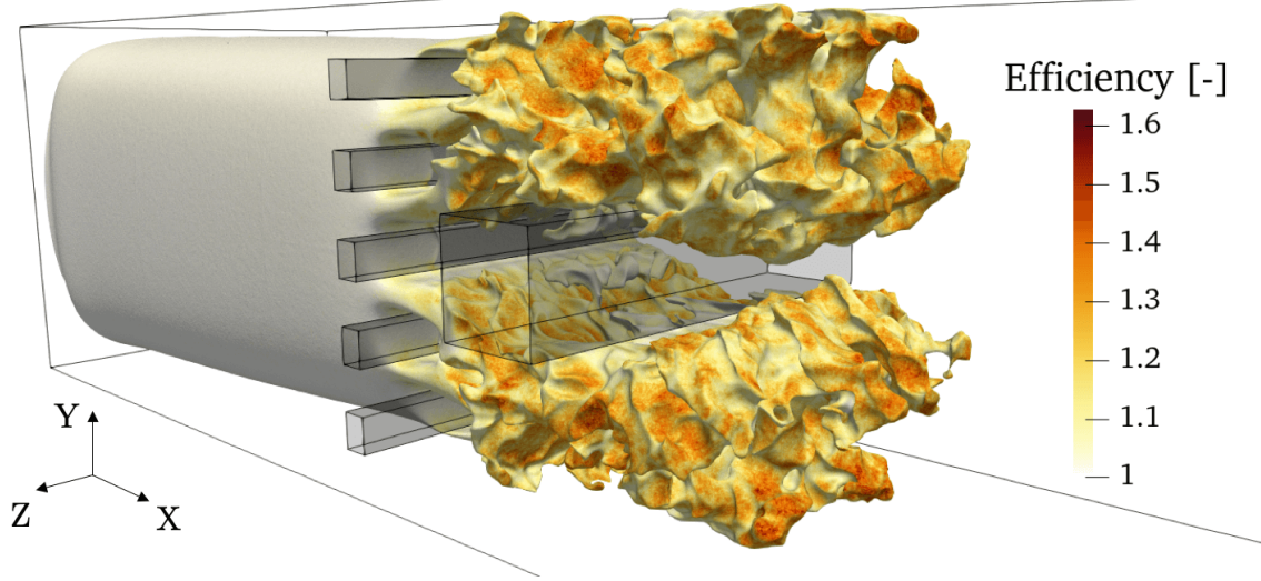
Figure 8.17: Iso-surface of \bar{c} = 0.86 colored by efficiency in the VRLES. \bar{c} = 0.86 is the progress variable value of peak heat release rate in a laminar flame.
