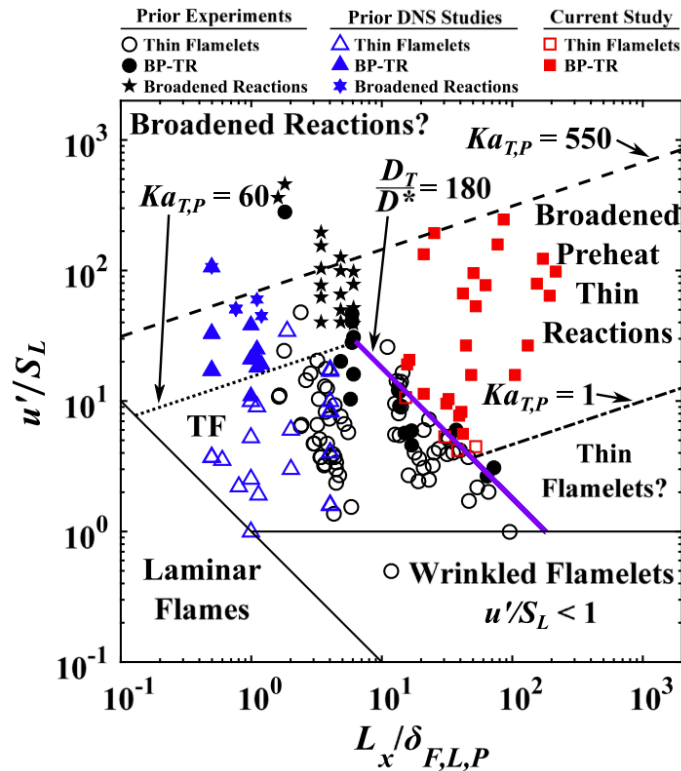
Figure 2.6: Measured premixed combustion regime diagram with DNS and experimental data points. Reprinted from Skiba et al. [346] with permission from Elsevier, license number 5364270406074.
