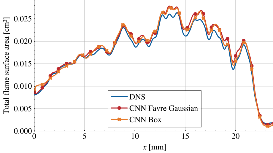
Figure 5.18: Evolution of the total flame surface area along the streamwise direction on a validation snapshot of R2 for different filter types.
