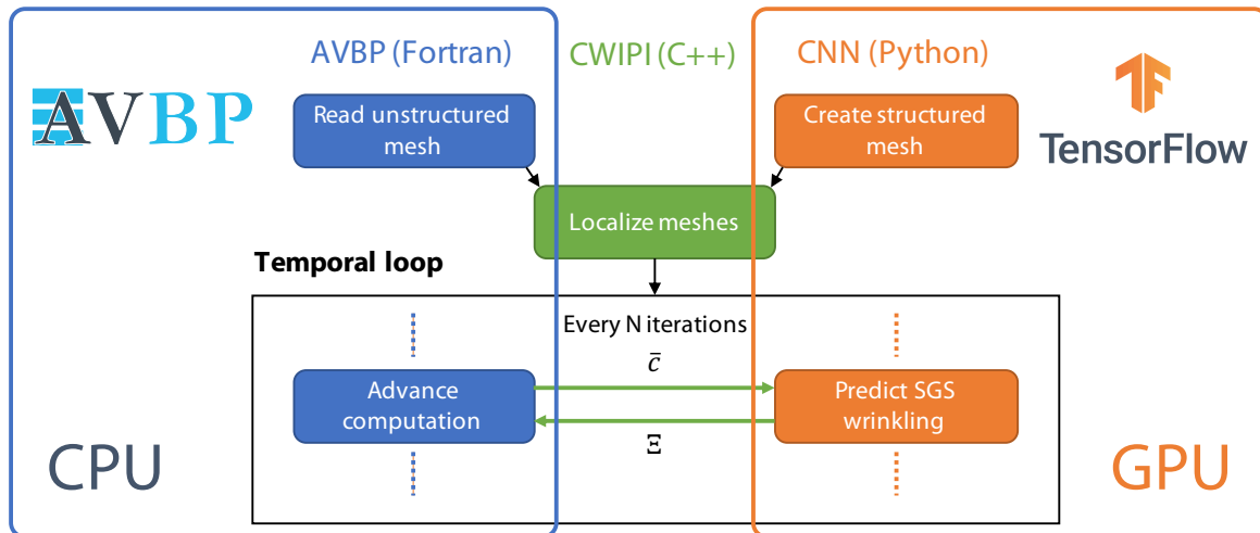
Figure 7.1: High-level overview of the AVBP-DL coupling strategy.
